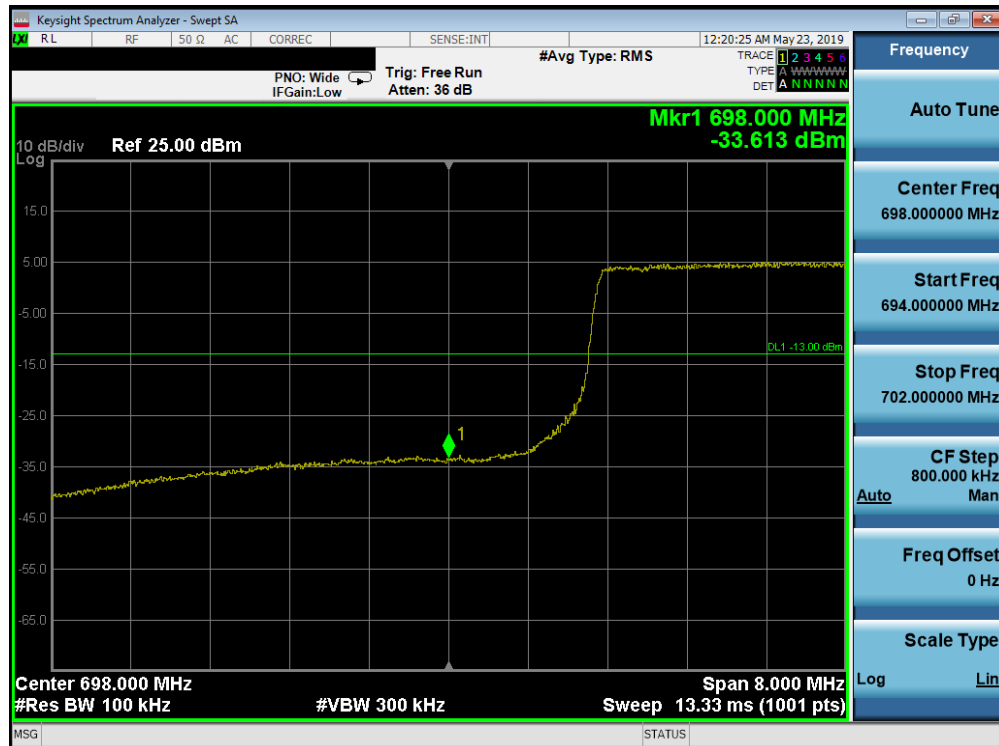
Plot 7-84. Lower Band Edge Plot (Band 12 - 10.0MHz QPSK - Full RB Configuration)
