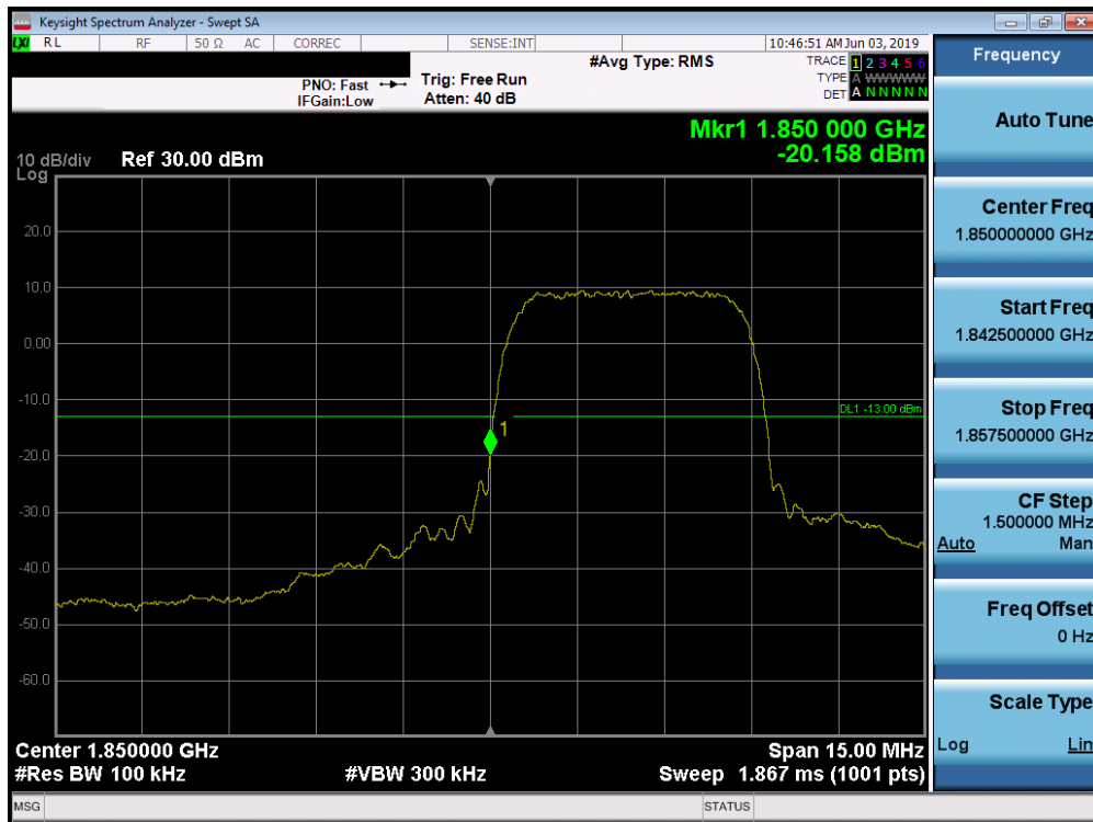
Plot 7-62. Band Edge Plot (PCS WCDMA Mode - Low Channel)
