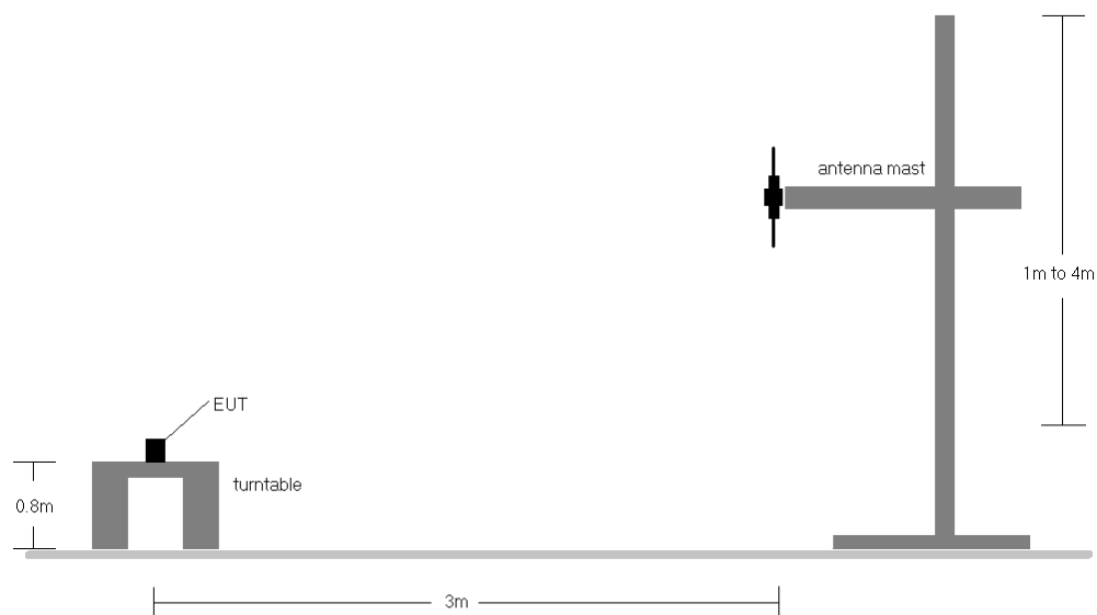
Figure 7-4. Radiated Test Setup
