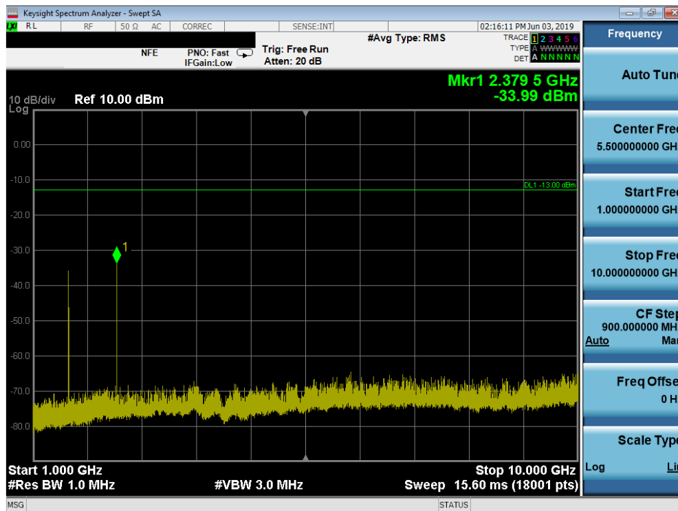
Plot 7-7. Conducted Spurious Plot (LTE Band 14, 10.0MHz QPSK – RB Size 1, RB Offset 0)
