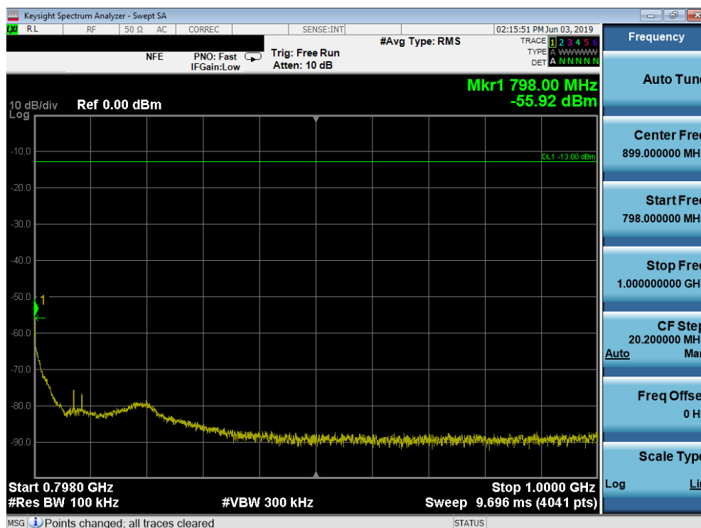
Plot 7-6. Conducted Spurious Plot (LTE Band 14, 10.0MHz QPSK – RB Size 1, RB Offset 0)
