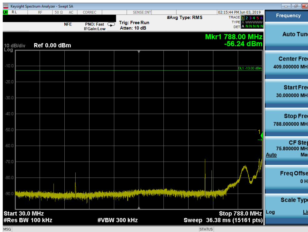
Plot 7-5. Conducted Spurious Plot (LTE Band 14, 10.0MHz QPSK – RB Size 1, RB Offset 0)
