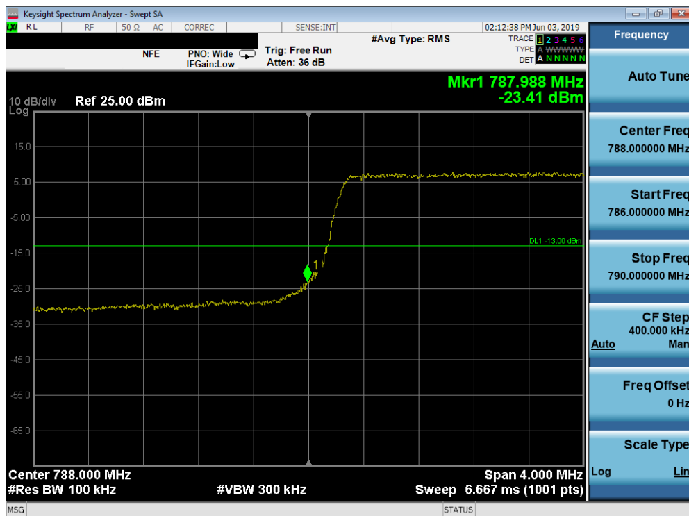
Plot 7-9. Lower Band Edge Plot (LTE Band 14, 5MHz QPSK – RB Size 25)
