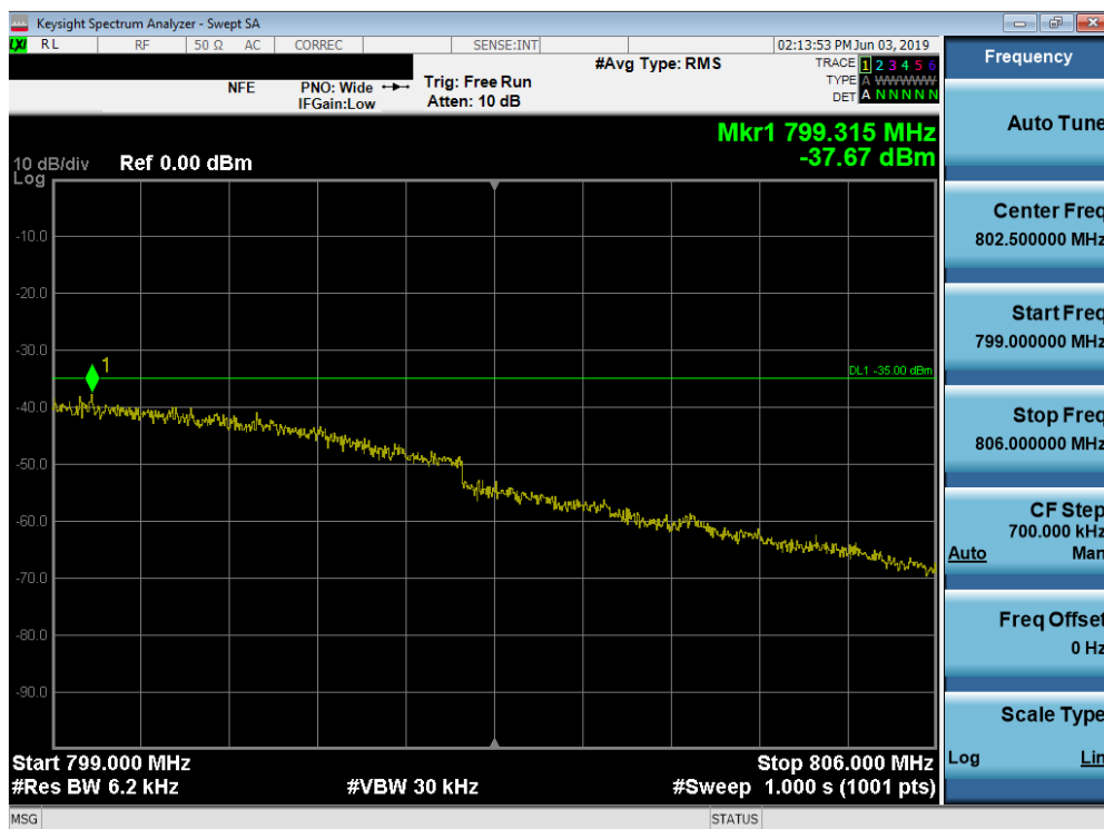
Plot 7-11. Upper Emission Mask Plot (LTE Band 14, 5MHz QPSK – RB Size 25)
