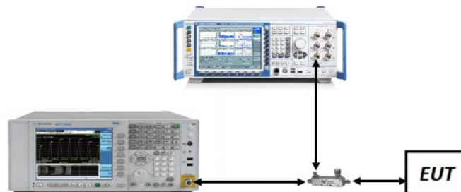
Figure 7-3. Test Instrument & Measurement Setup
