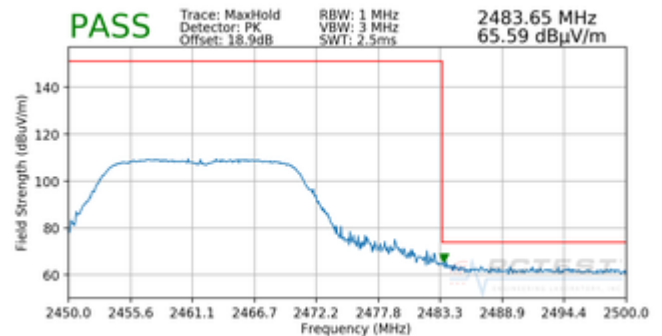
Plot 7-41. Radiated Restricted Upper Band Edge Measurement (Peak)
