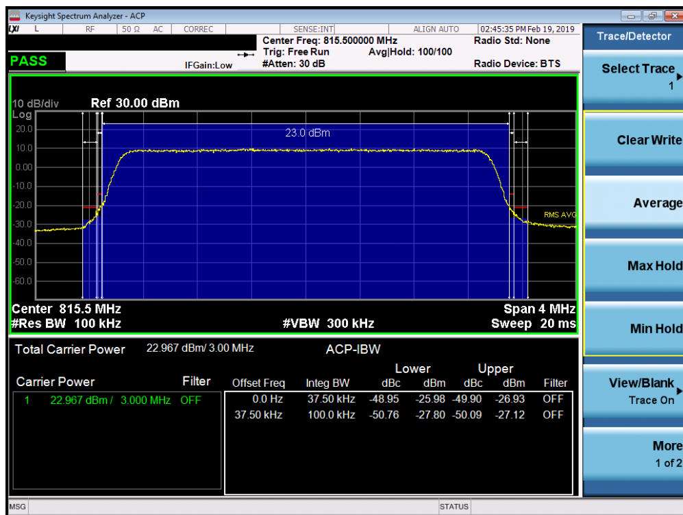
Plot 7-16. Channel Edge Plot (LTE Band 26, 3MHz 16-QAM – RB Size 15– Low Channel)
