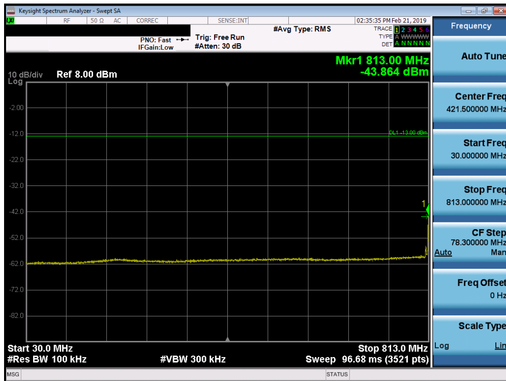
Plot 7-11. Conducted Spurious Plot (LTE Band 26, 10MHz QPSK – RB Size 1, RB Offset 0 – Mid Channel)
