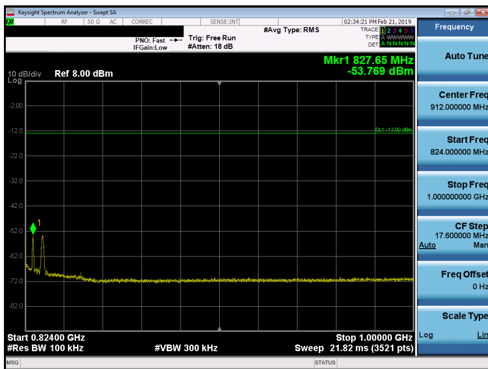
Plot 7-12. Conducted Spurious Plot (LTE Band 26, 10MHz QPSK – RB Size 1, RB Offset 0 – Mid Channel)
