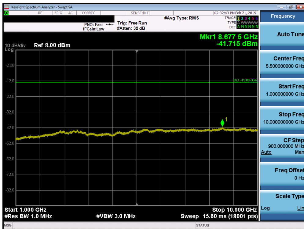
Plot 7-13. Conducted Spurious Plot (LTE Band 26, 10MHz QPSK – RB Size 1, RB Offset 0 – Mid Channel)
