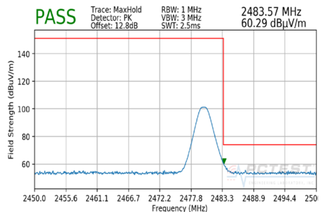
Plot 7-19. Radiated Restricted Upper Band Edge Measurement (Peak)
