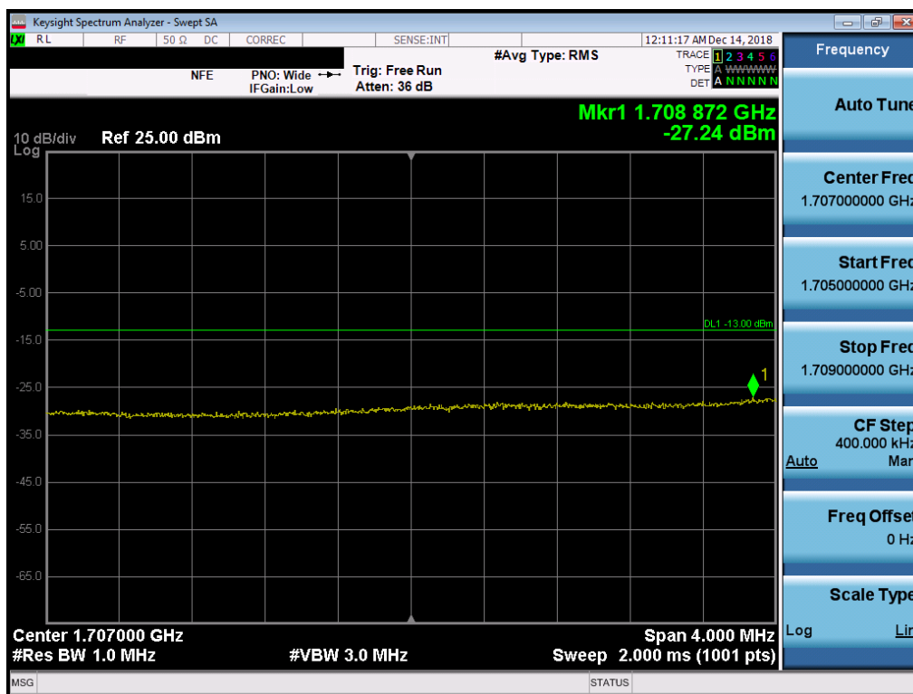
Plot 7-110. Lower Extended Band Edge Plot (Band 4 - 15.0MHz QPSK - Full RB Configuration)
