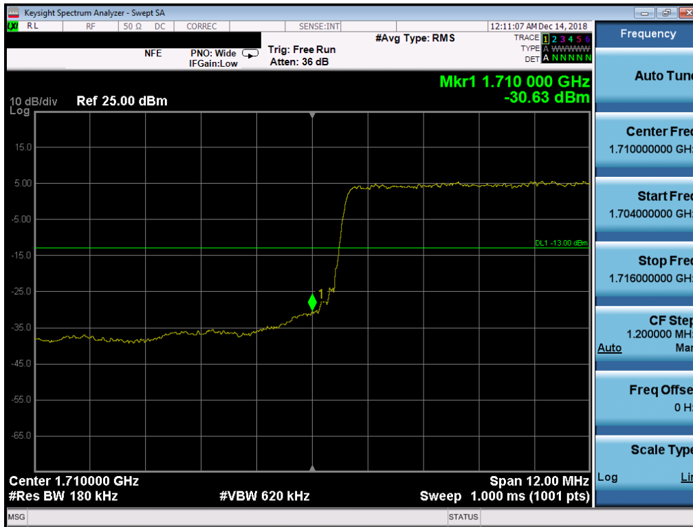
Plot 7-109. Lower Band Edge Plot (Band 4 - 15.0MHz QPSK - Full RB Configuration)
