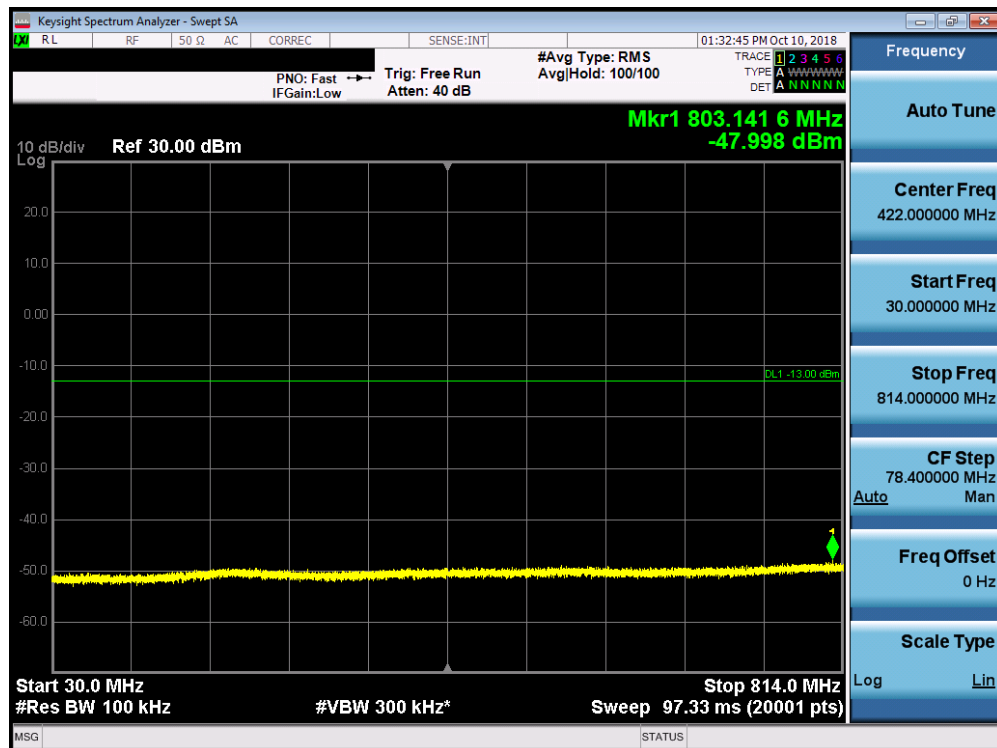
Plot 7-16. Conducted Spurious Plot (Ch. 684)
