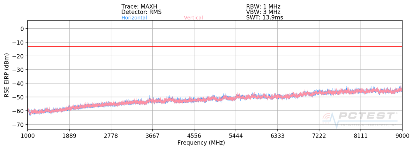
Plot 7-33. Radiated Spurious Plot Above 1GHz (BC10 CDMA Mode)
