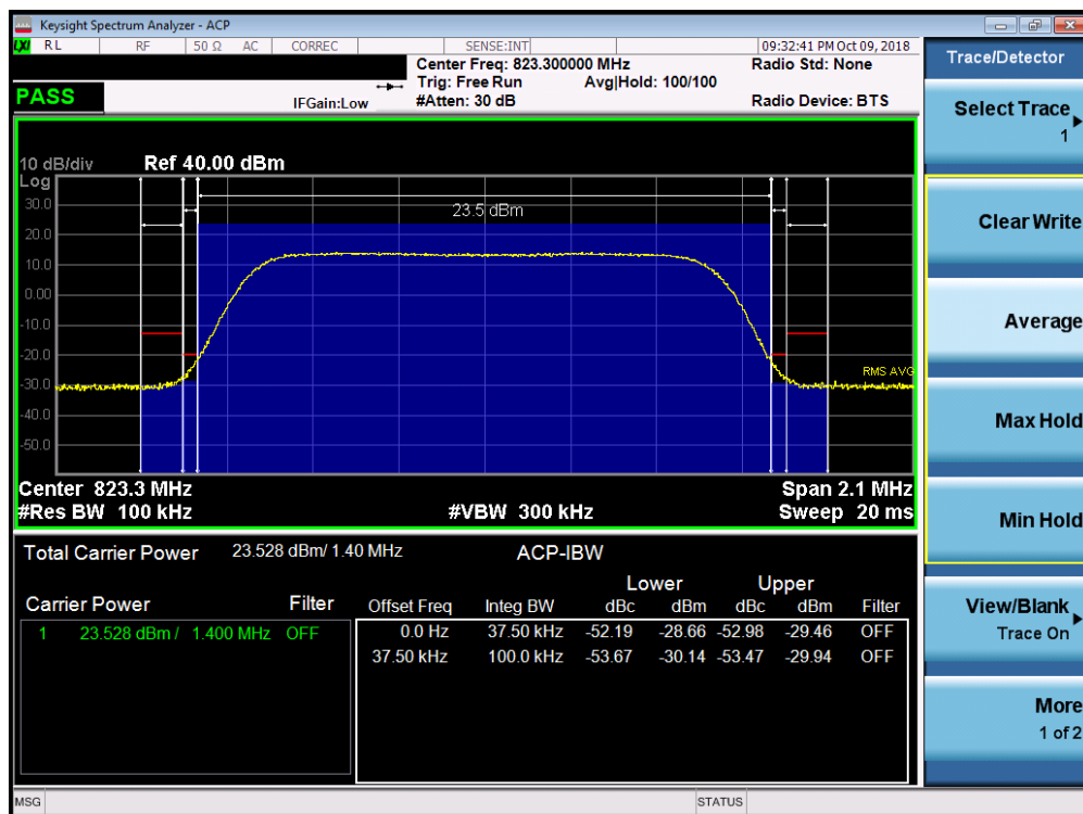
Plot 7-25. Channel Edge Plot (LTE Band 26, 1.4MHz QPSK – RB Size 6 – High Channel)
