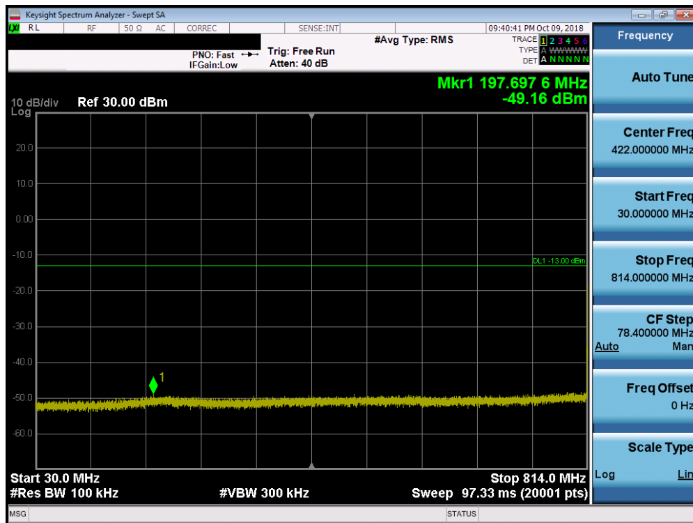
Plot 7-19. Conducted Spurious Plot (LTE Band 26, 15MHz QPSK – RB Size 1, RB Offset 0 – Low Channel)
