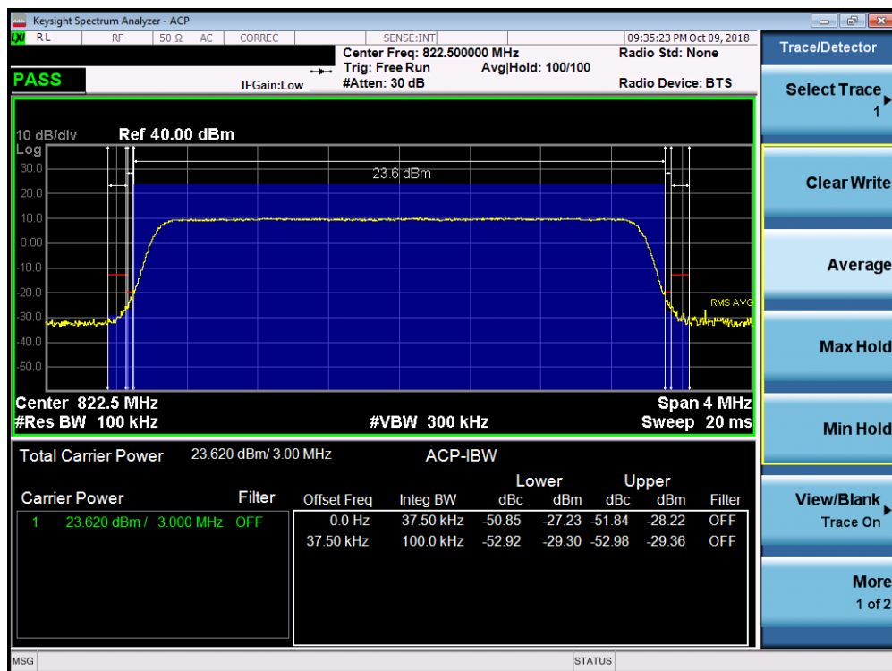
Plot 7-27. Channel Edge Plot (LTE Band 26, 3MHz QPSK – RB Size 15 – High Channel)
