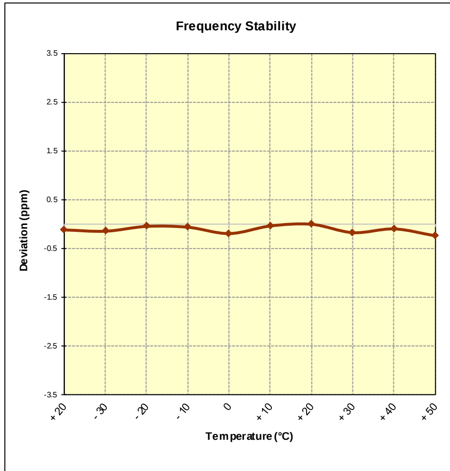
Figure 7-6. CDMA BC10 Frequency Stability Graph
