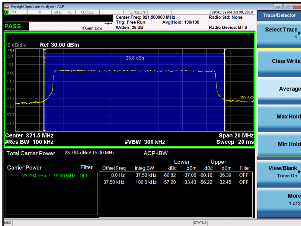
Plot 7-31. Channel Edge Plot (LTE Band 26, 15MHz QPSK – RB Size 75)
