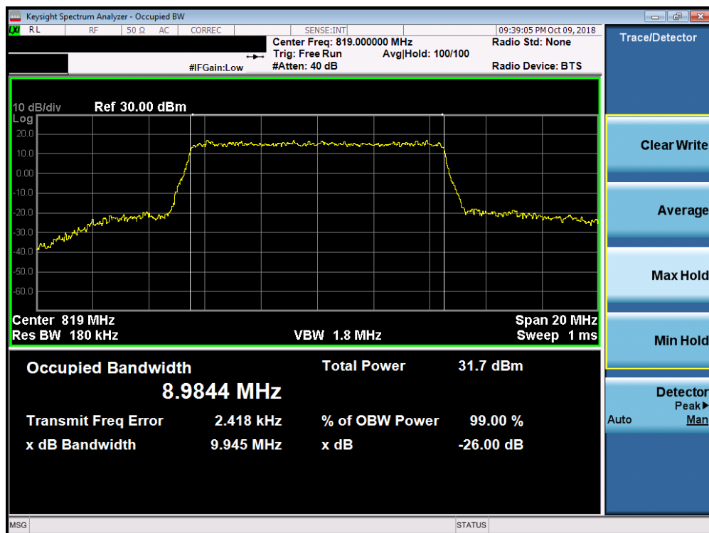
Plot 7-10. Occupied Bandwidth Plot (LTE Band 26, 10MHz 16-QAM – RB Size 50)
