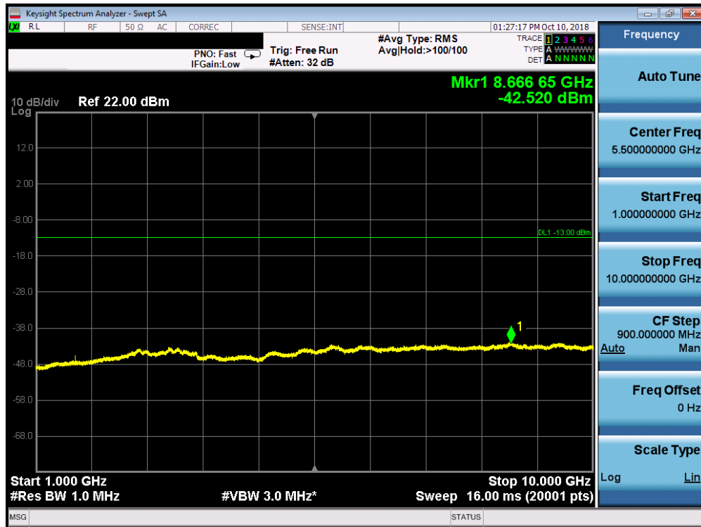
Plot 7-15. Conducted Spurious Plot (Ch. 476)
