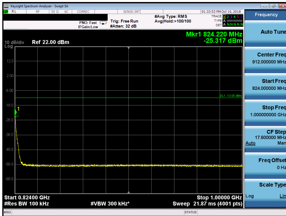
Plot 7-17. Conducted Spurious Plot (Ch. 684)
