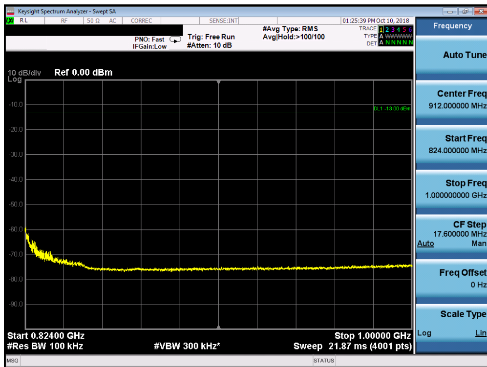
Plot 7-14. Conducted Spurious Plot (Ch. 476)
