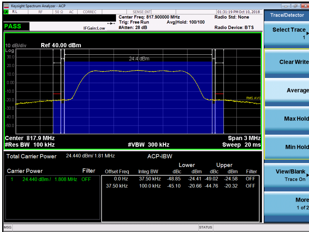
Plot 7-22. Channel Edge Plot (Ch. 476)
