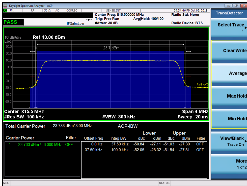
Plot 7-26. Channel Edge Plot (LTE Band 26, 3MHz QPSK – RB Size 15– Low Channel)
