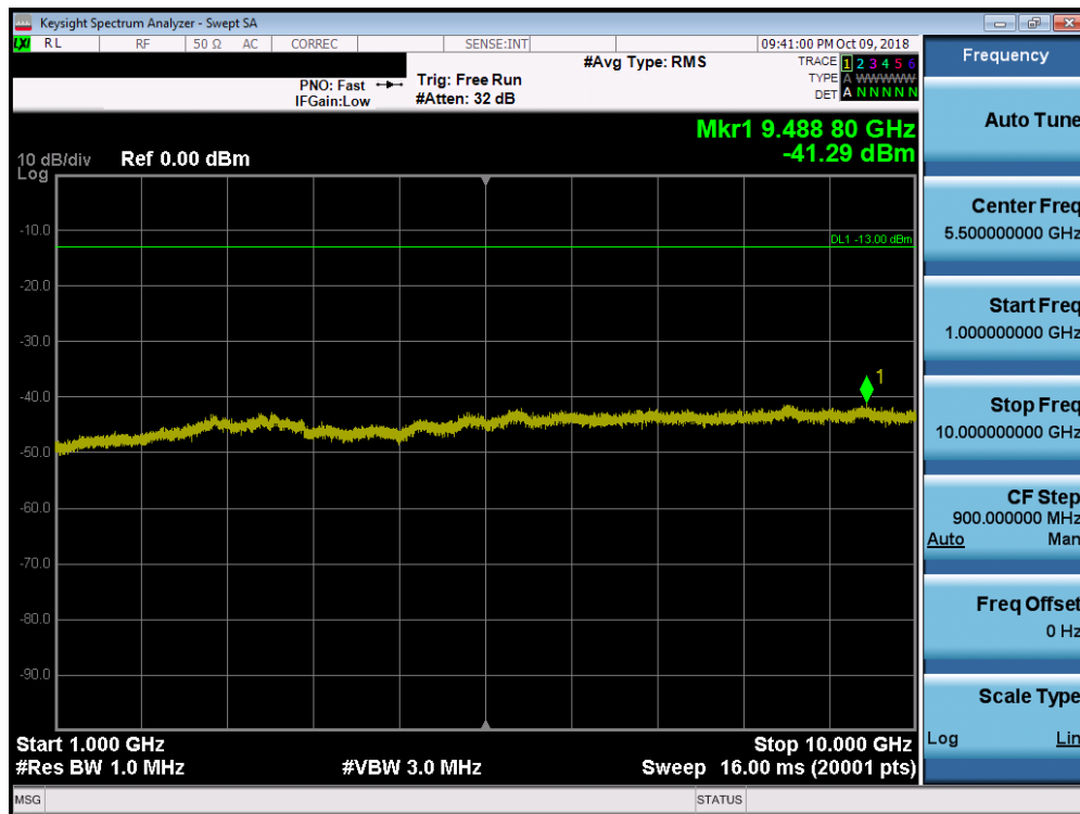
Plot 7-21. Conducted Spurious Plot (LTE Band 26, 15MHz QPSK – RB Size 1, RB Offset 0 – Low Channel)
