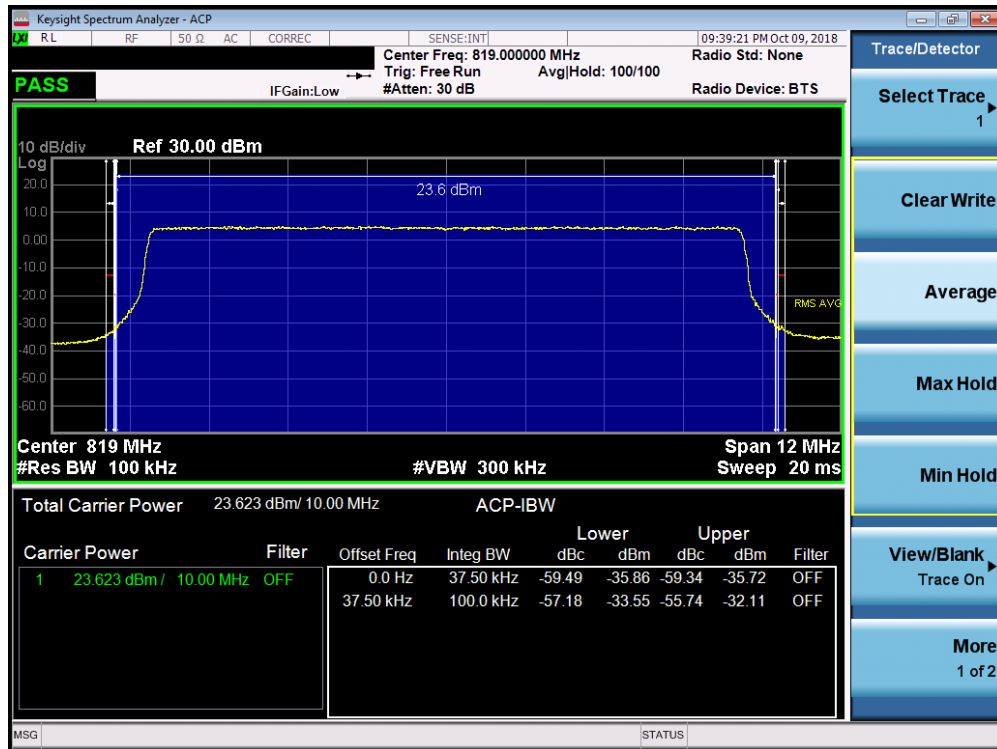
Plot 7-30. Channel Edge Plot (LTE Band 26, 10MHz QPSK – RB Size 50)
