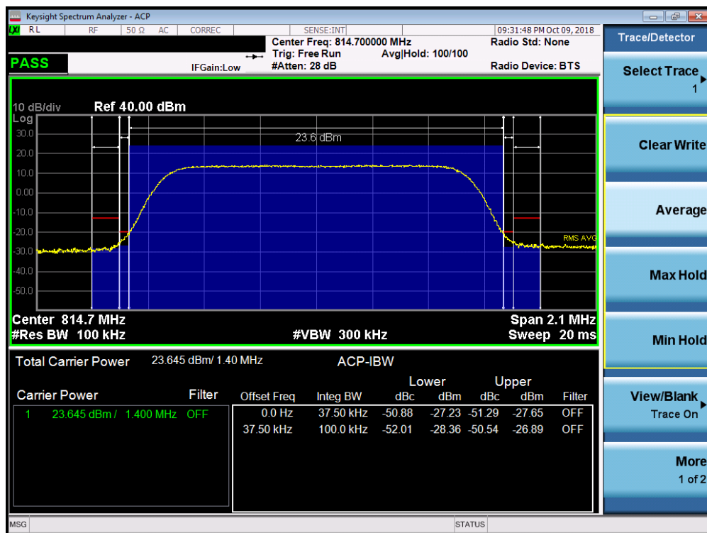
Plot 7-24. Channel Edge Plot (LTE Band 26, 1.4MHz QPSK – RB Size 6– Low Channel)
