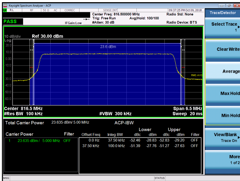
Plot 7-28. Channel Edge Plot (LTE Band 26, 5MHz QPSK – RB Size 25– Low Channel)
