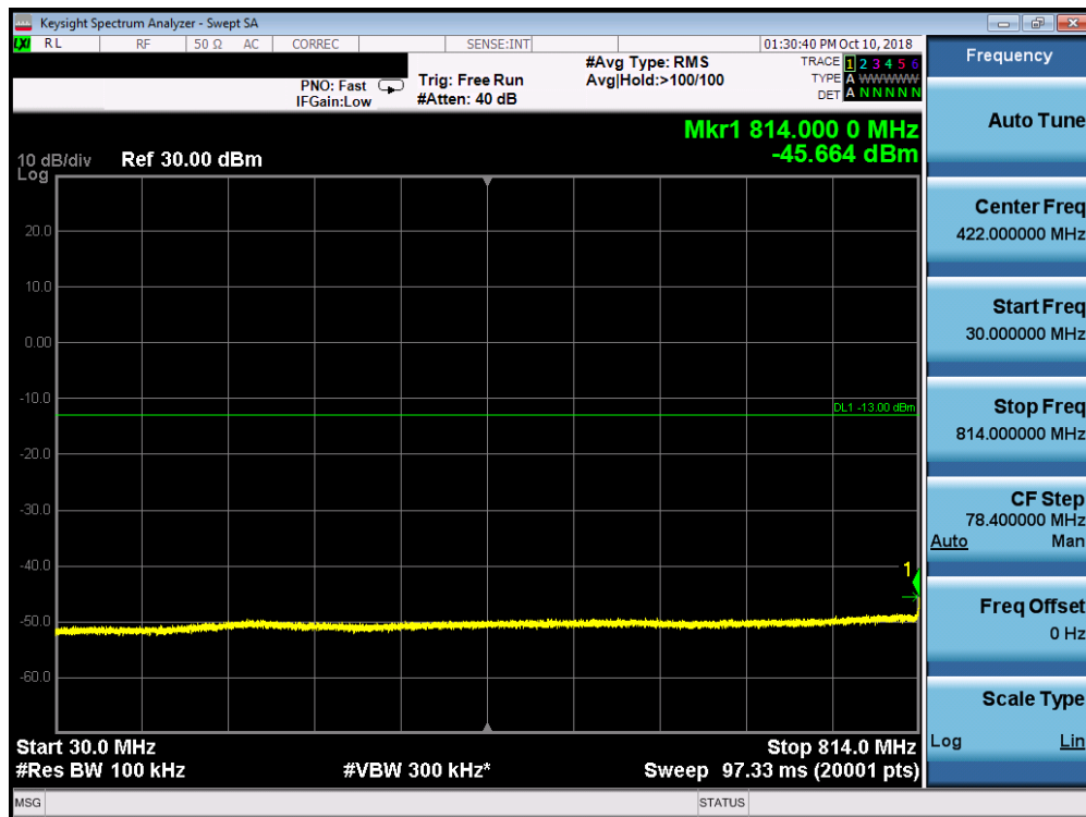
Plot 7-13. Conducted Spurious Plot (Ch. 476)
