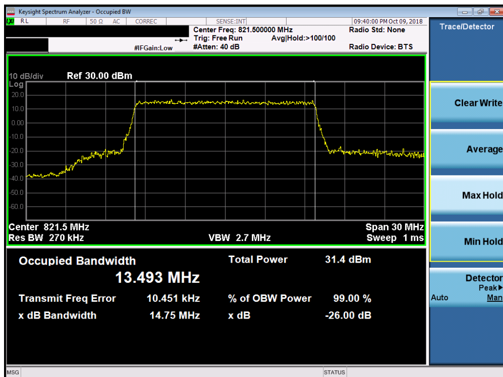
Plot 7-12. Occupied Bandwidth Plot (LTE Band 26, 15MHz 16-QAM – RB Size 75)
