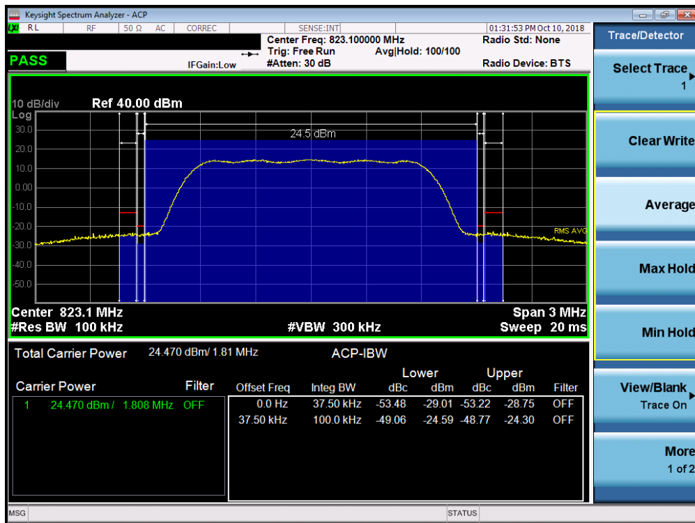
Plot 7-23. Channel Edge Plot (Ch. 684)
