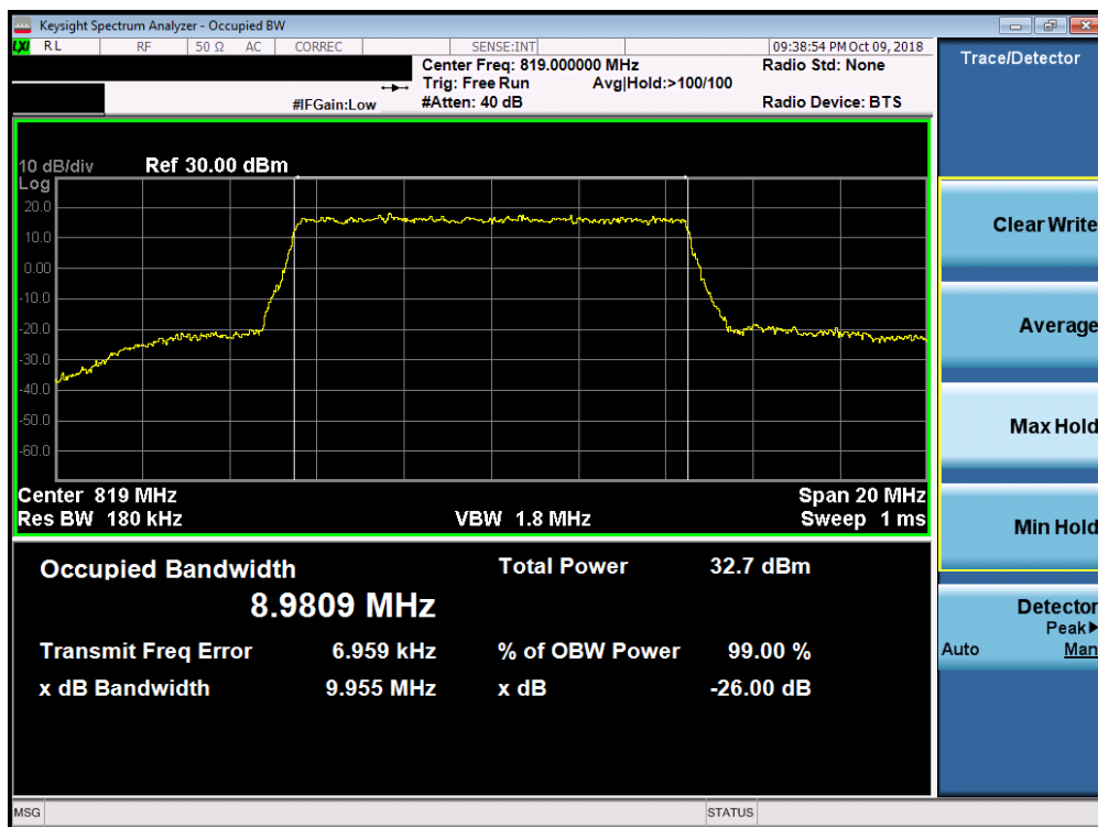
Plot 7-9. Occupied Bandwidth Plot (LTE Band 26, 10MHz QPSK – RB Size 50)
