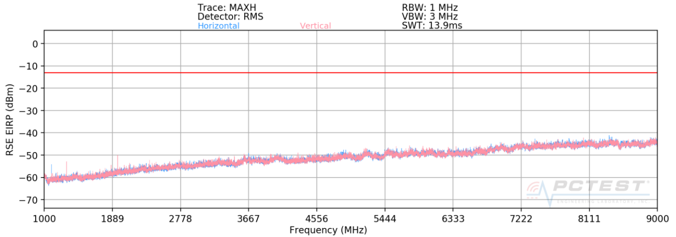
Plot 7-34. Radiated Spurious Plot Above 1GHz (Band 26 LTE Mode)
