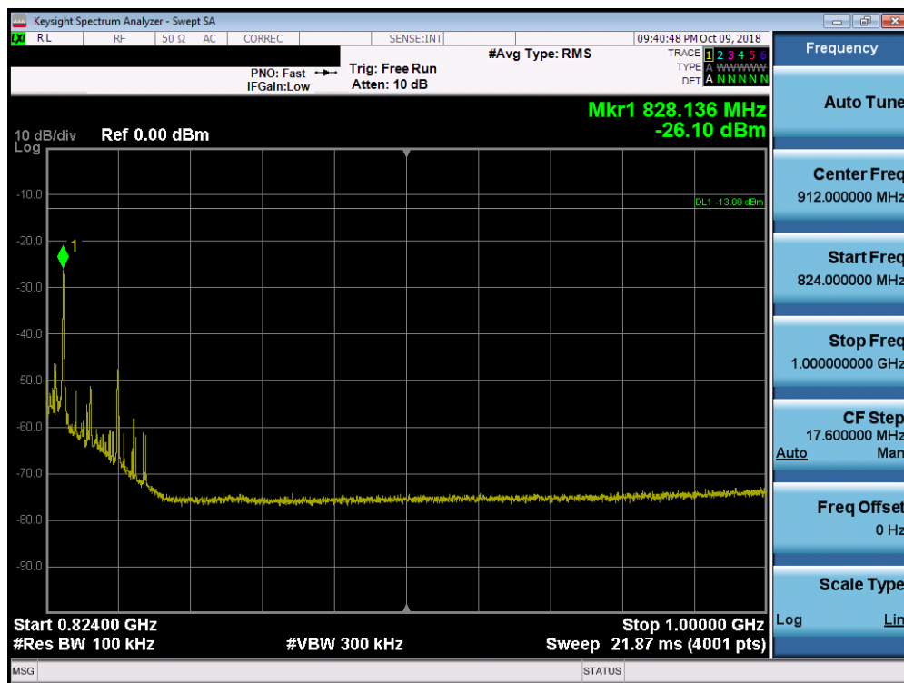
Plot 7-20. Conducted Spurious Plot (LTE Band 26, 15MHz QPSK – RB Size 1, RB Offset 0 – Low Channel)
