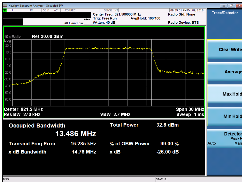
Plot 7-11. Occupied Bandwidth Plot (LTE Band 26, 15MHz QPSK – RB Size 75)
