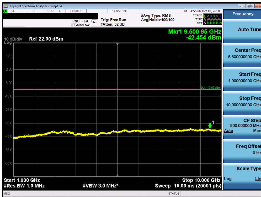
Plot 7-18. Conducted Spurious Plot (Ch. 684)
