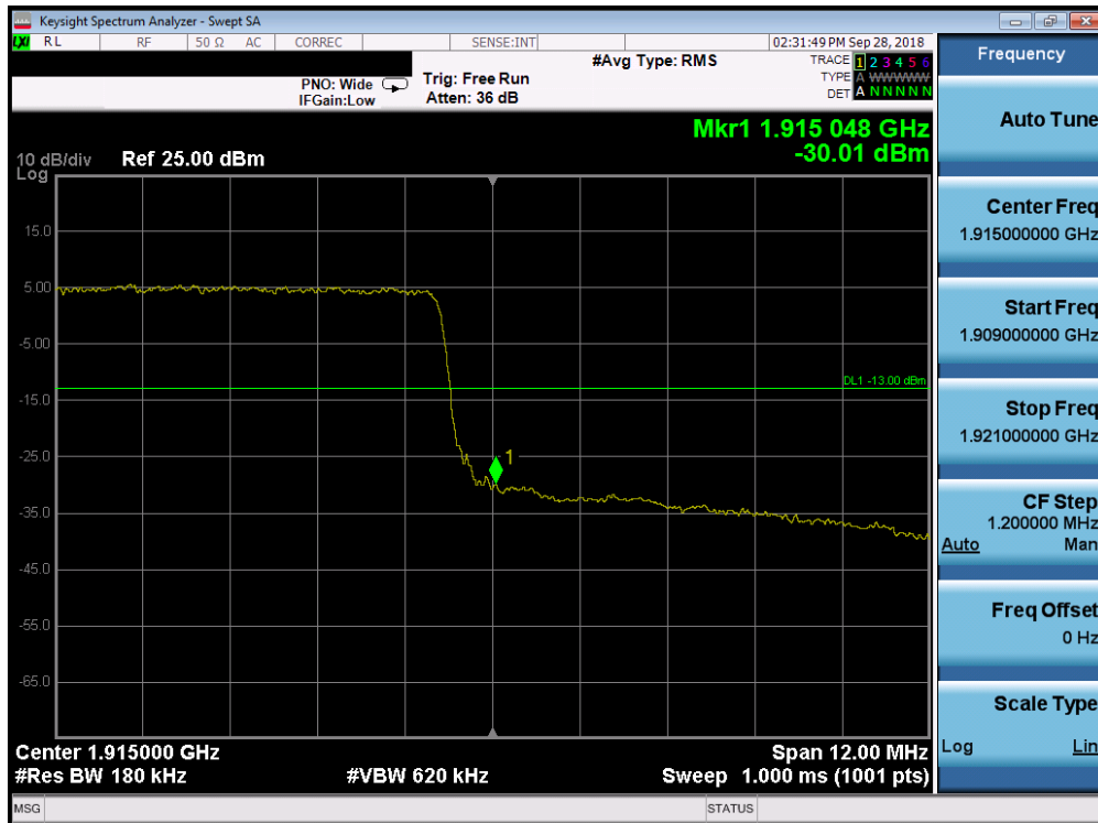
Plot 7-197. Upper Band Edge Plot (Band 25 - 15.0MHz QPSK - Full RB Configuration)
