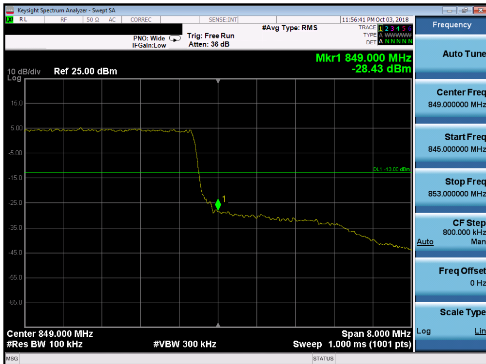
Plot 7-142. Upper Band Edge Plot (Band 26/5 - 10.0MHz QPSK - Full RB Configuration)
