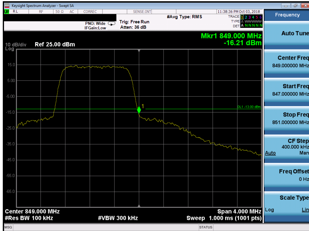
Plot 7-136. Upper Band Edge Plot (Band 26/5 - 1.4MHz QPSK - Full RB Configuration)
