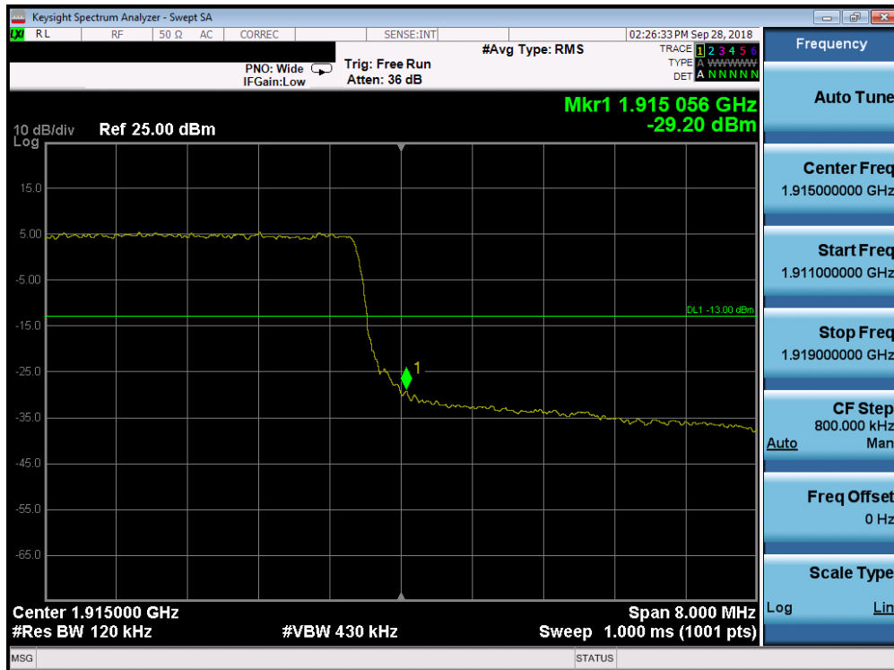
Plot 7-191. Upper Band Edge Plot (Band 25 - 10.0MHz QPSK - Full RB Configuration)
