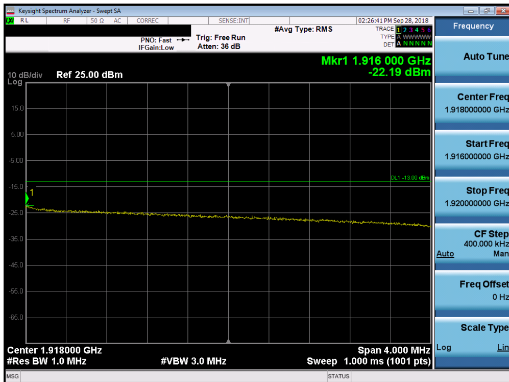
Plot 7-192. Upper Extended Band Edge Plot (Band 25 - 10.0MHz QPSK - Full RB Configuration)
