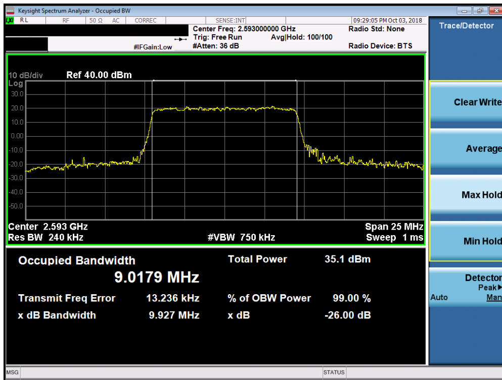
Plot 7-48. Occupied Bandwidth Plot (Band 41 - 10.0MHz QPSK - Full RB Configuration)
