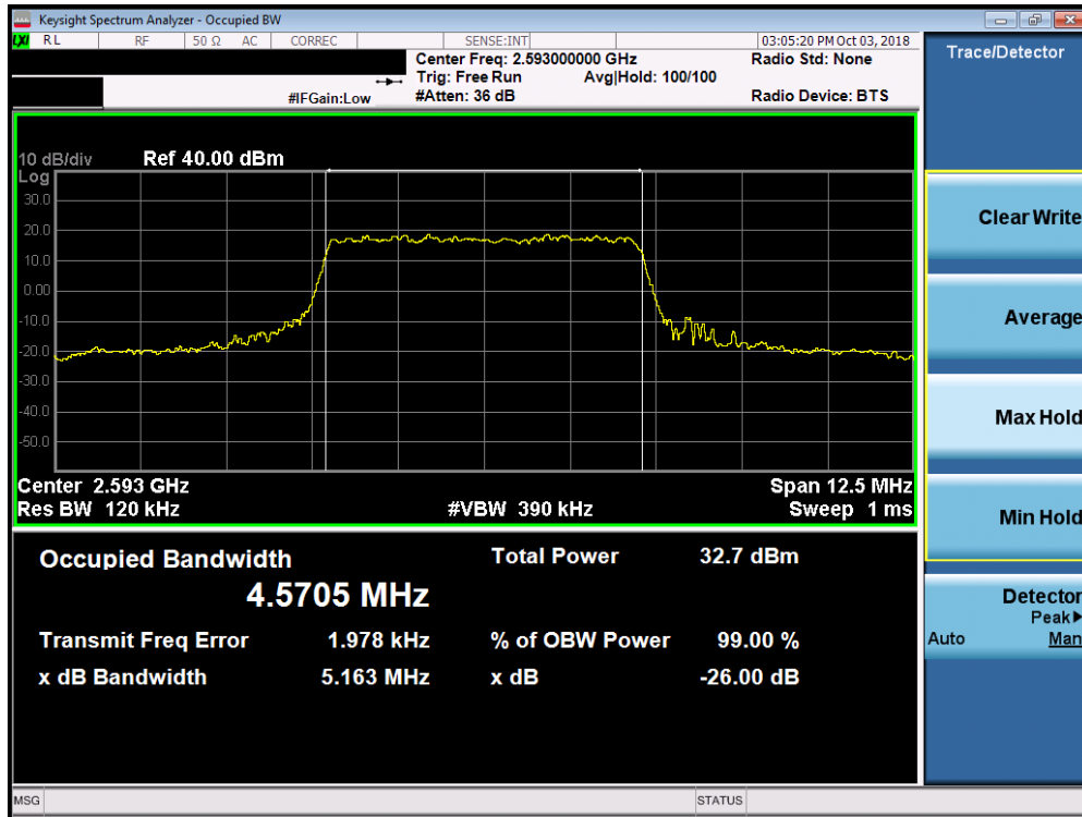
Plot 7-54. Occupied Bandwidth Plot (Band 41 - 5.0MHz QPSK - Full RB Configuration)
