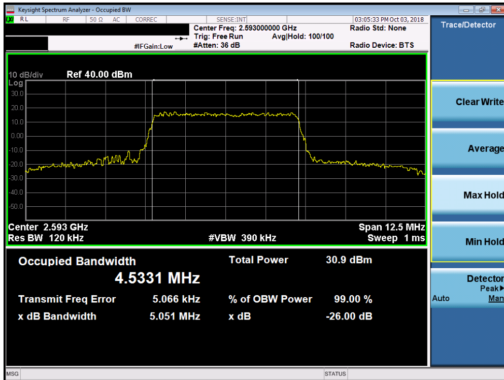
Plot 7-55. Occupied Bandwidth Plot (Band 41 - 5.0MHz 16-QAM - Full RB Configuration)
