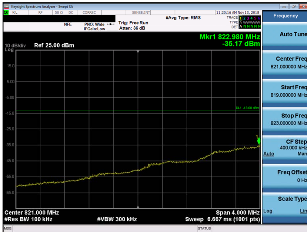
Plot 7-42. Lower Extended Band Edge Plot (Band 26 - 1.4MHz QPSK - Full RB Configuration)
