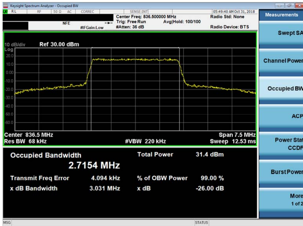
Plot 7-3. Occupied Bandwidth Plot (Band 26 - 3.0MHz QPSK - Full RB Configuration)
