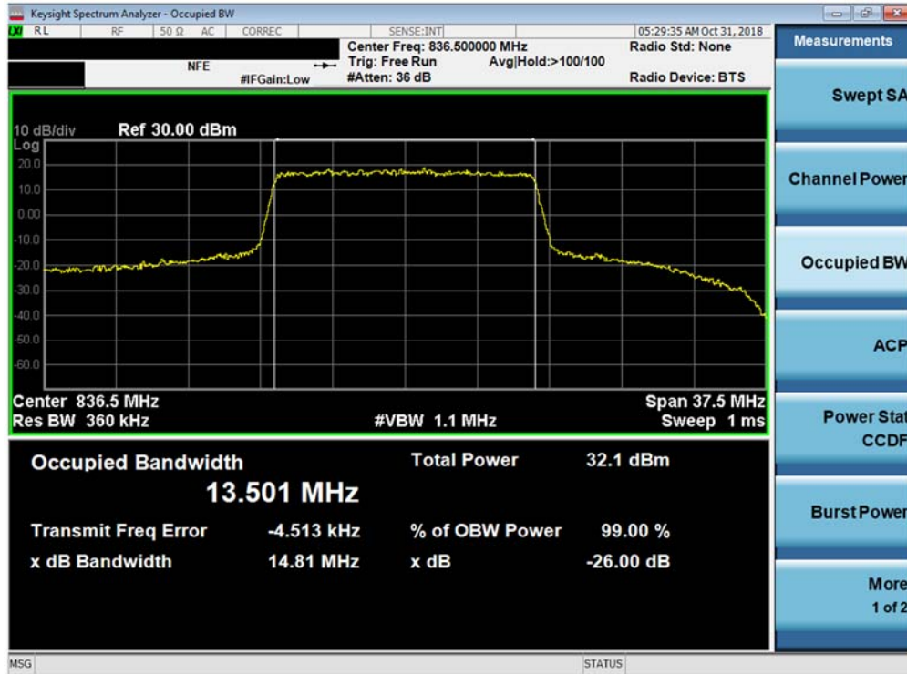
Plot 7-9. Occupied Bandwidth Plot (Band 26 - 15.0MHz QPSK - Full RB Configuration)
