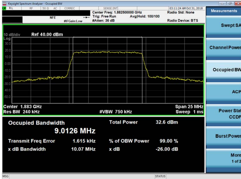
Plot 7-17. Occupied Bandwidth Plot (Band 25 - 10.0MHz QPSK - Full RB Configuration)
