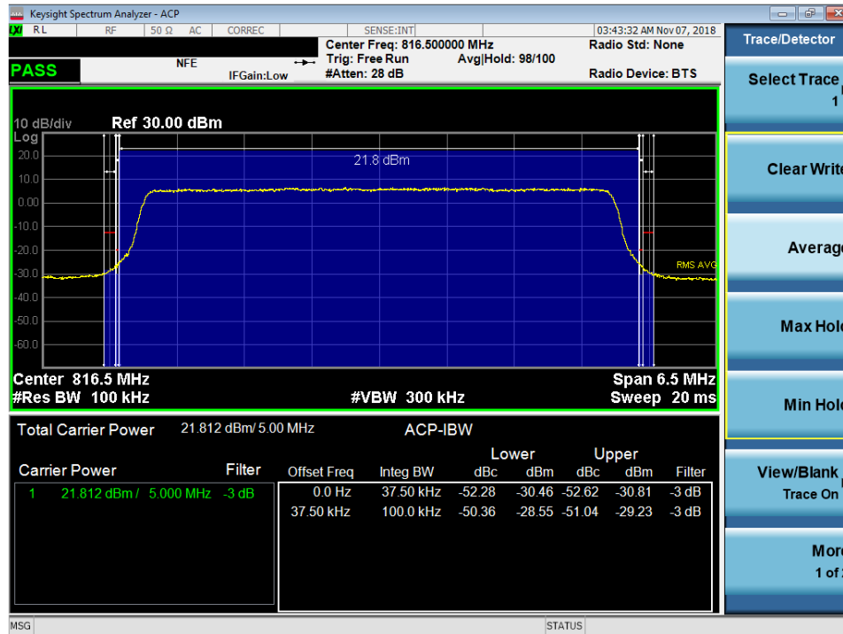
Plot 7-21. Channel Edge Plot (LTE Band 26, 5MHz QPSK – RB Size 25– Low Channel)
