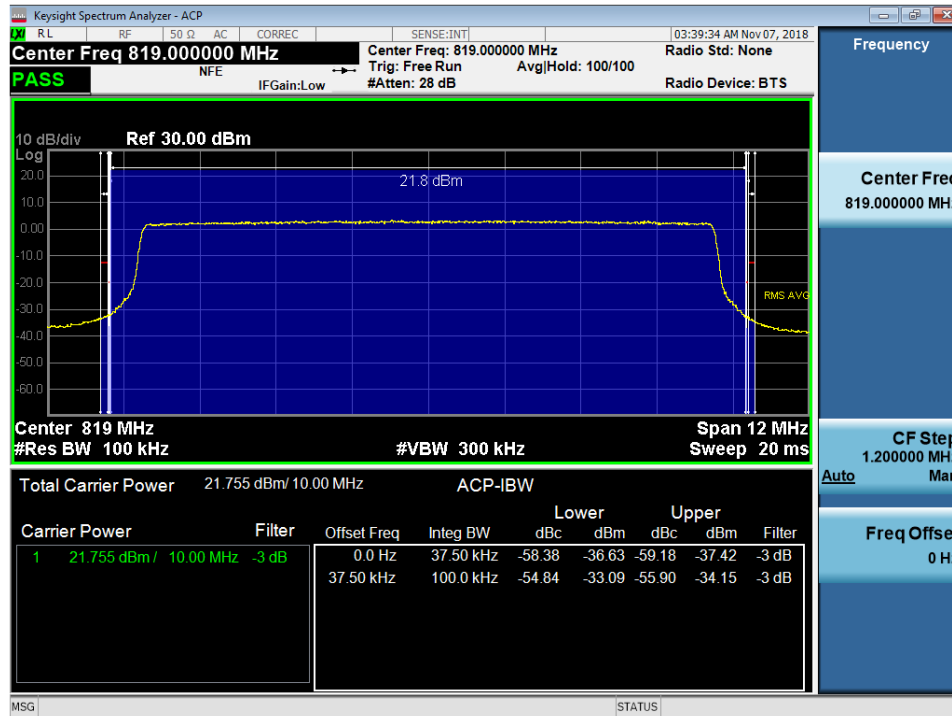
Plot 7-23. Channel Edge Plot (LTE Band 26, 10MHz QPSK – RB Size 50)
