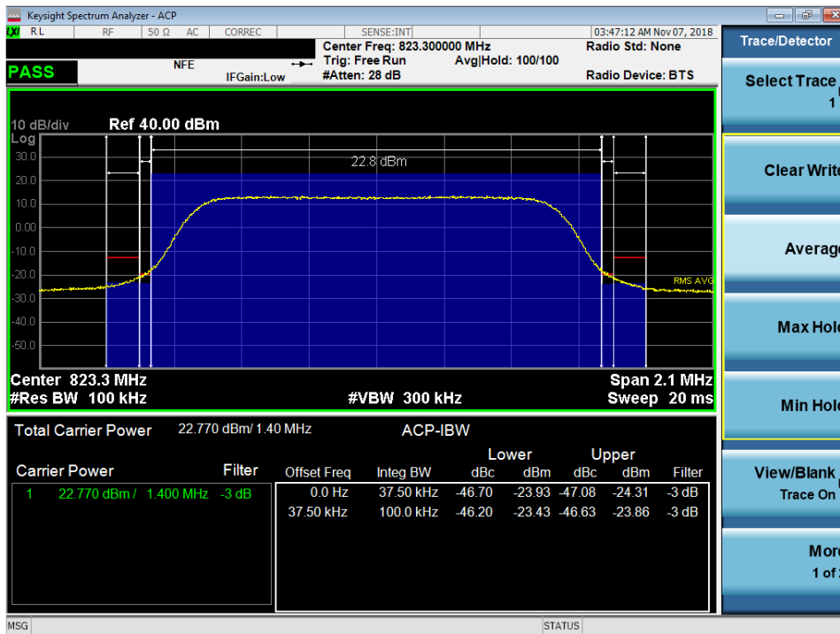
Plot 7-18. Channel Edge Plot (LTE Band 26, 1.4MHz QPSK – RB Size 6 – High Channel)
