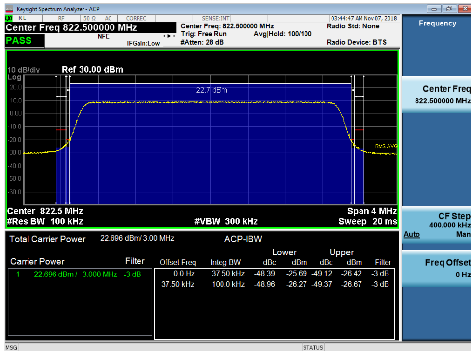
Plot 7-20. Channel Edge Plot (LTE Band 26, 3MHz QPSK – RB Size 15 – High Channel)
