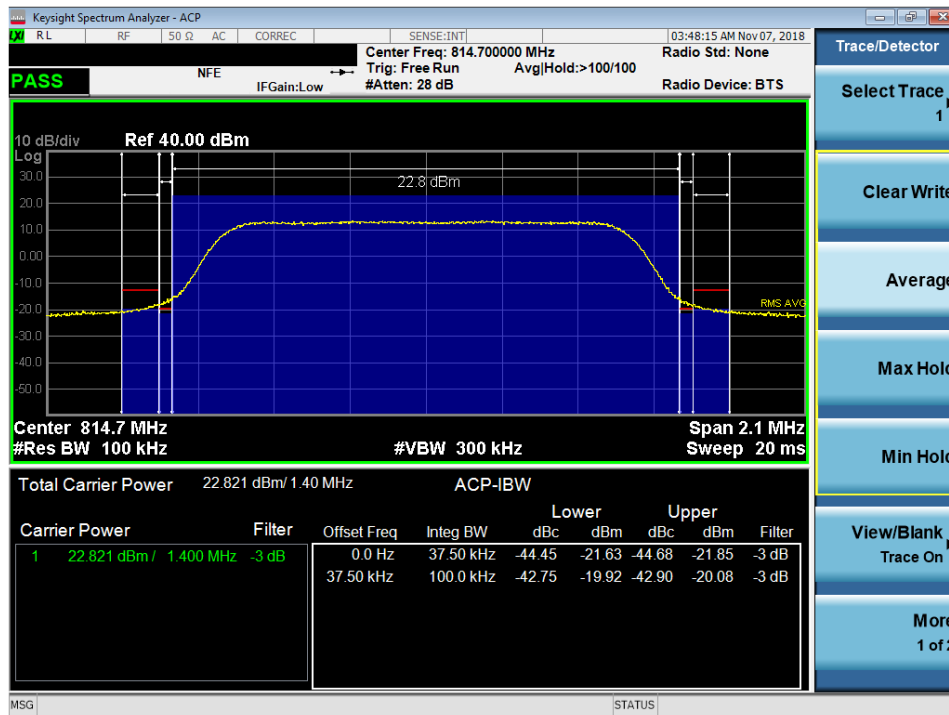
Plot 7-17. Channel Edge Plot (LTE Band 26, 1.4MHz QPSK – RB Size 6– Low Channel)
