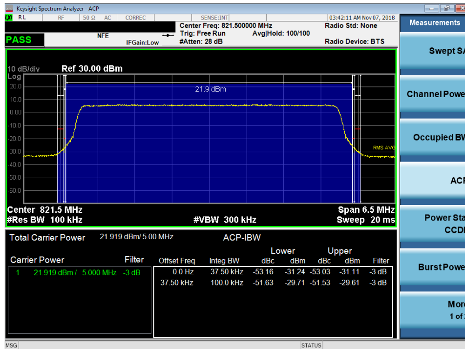
Plot 7-22. Channel Edge Plot (LTE Band 26, 5MHz QPSK – RB Size 25 – High Channel)
