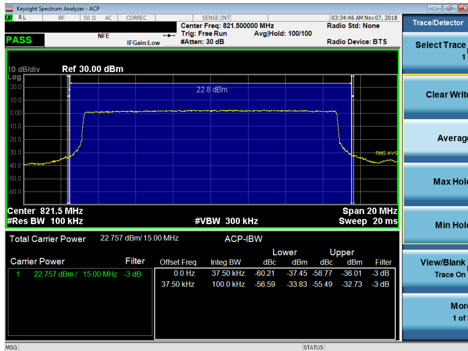
Plot 7-24. Channel Edge Plot (LTE Band 26, 15MHz QPSK – RB Size 75)
