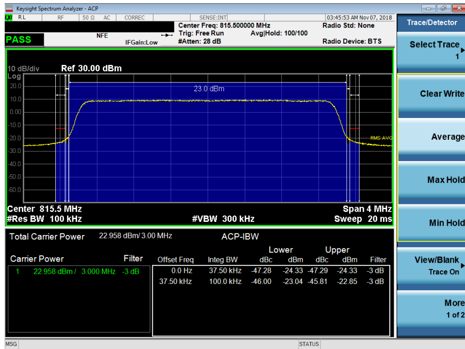
Plot 7-19. Channel Edge Plot (LTE Band 26, 3MHz QPSK – RB Size 15– Low Channel)
