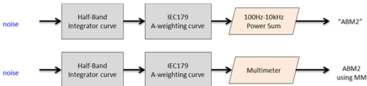
Figure 4-9 ABM2 Validation Block Diagram
