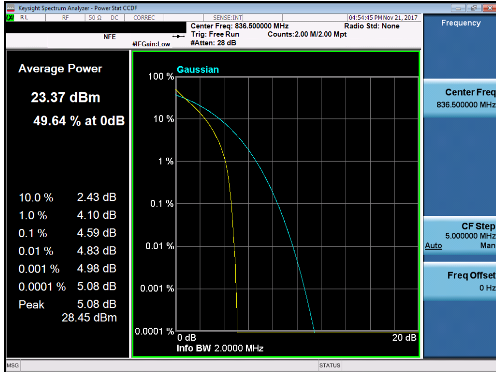
Plot 7-141. PAR Plot (Band 5 - 1.4MHz QPSK - Full RB Configuration)
