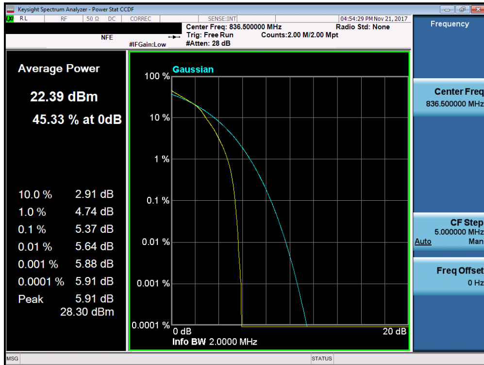
Plot 7-142. PAR Plot (Band 5 - 1.4MHz 16-QAM - Full RB Configuration)
