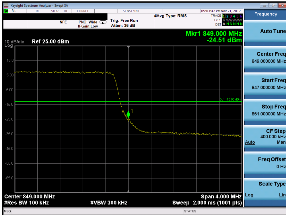
Plot 7-86. Upper Band Edge Plot (Band 5 - 5.0MHz QPSK - Full RB Configuration)
