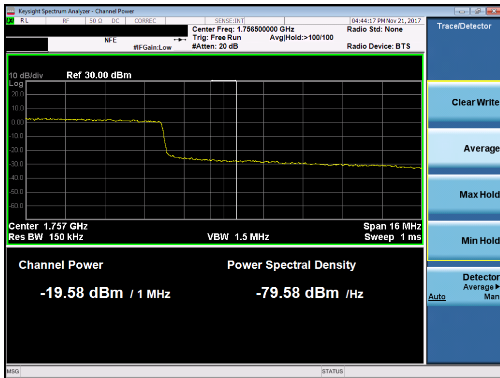
Plot 7-112. Upper Extended Band Edge Plot (Band 4 - 20.0MHz QPSK - Full RB Configuration)
