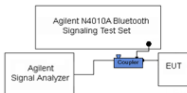
Figure 7-3. Test Instrument & Measurement Setup
