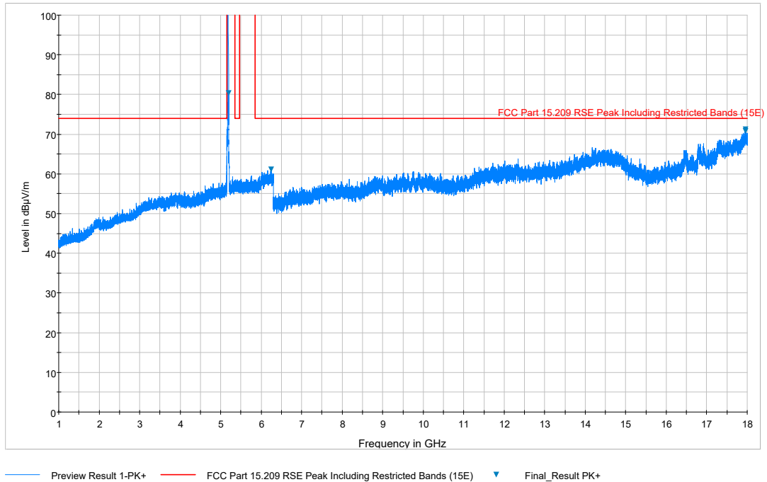
Plot 7-67. Radiated Spurious Plot above 1GHz (802.11a – U1 Ch. 40, Ant. Pol. H)
