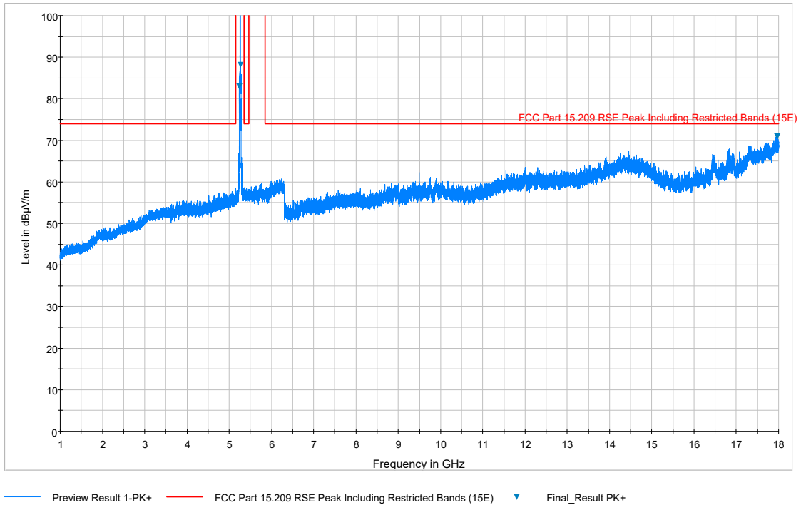
Plot 7-69. Radiated Spurious Plot above 1GHz (802.11a – U2A Ch. 56, Ant. Pol. H)
