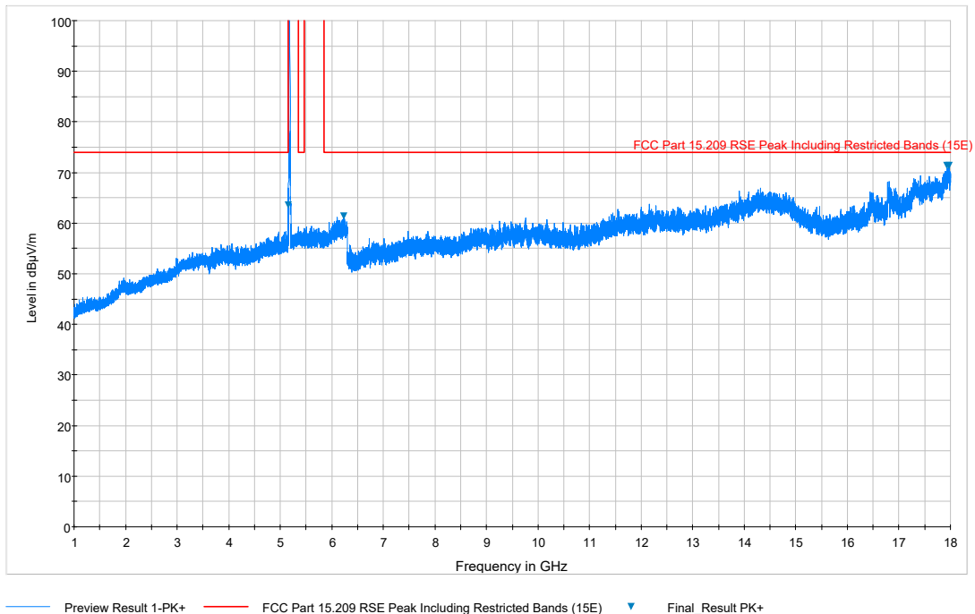
Plot 7-68. Radiated Spurious Plot above 1GHz (802.11a – U1 Ch. 40, Ant. Pol. V)
