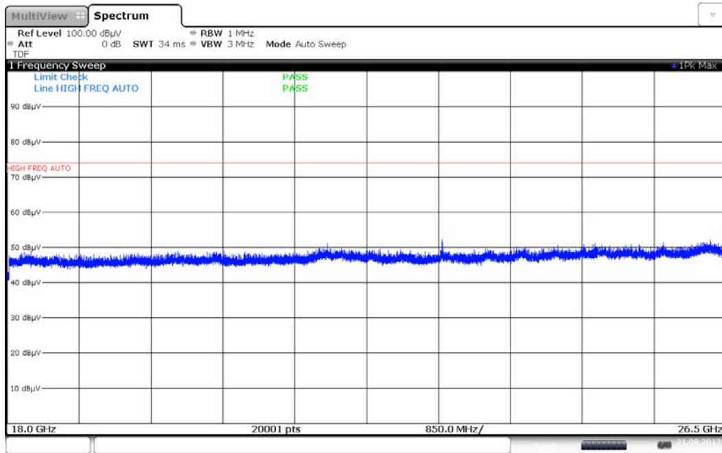
Plot 7-75. Radiated Spurious Plot 18GHz - 26.5GHz (802.11a – Ant. Pol. H)
