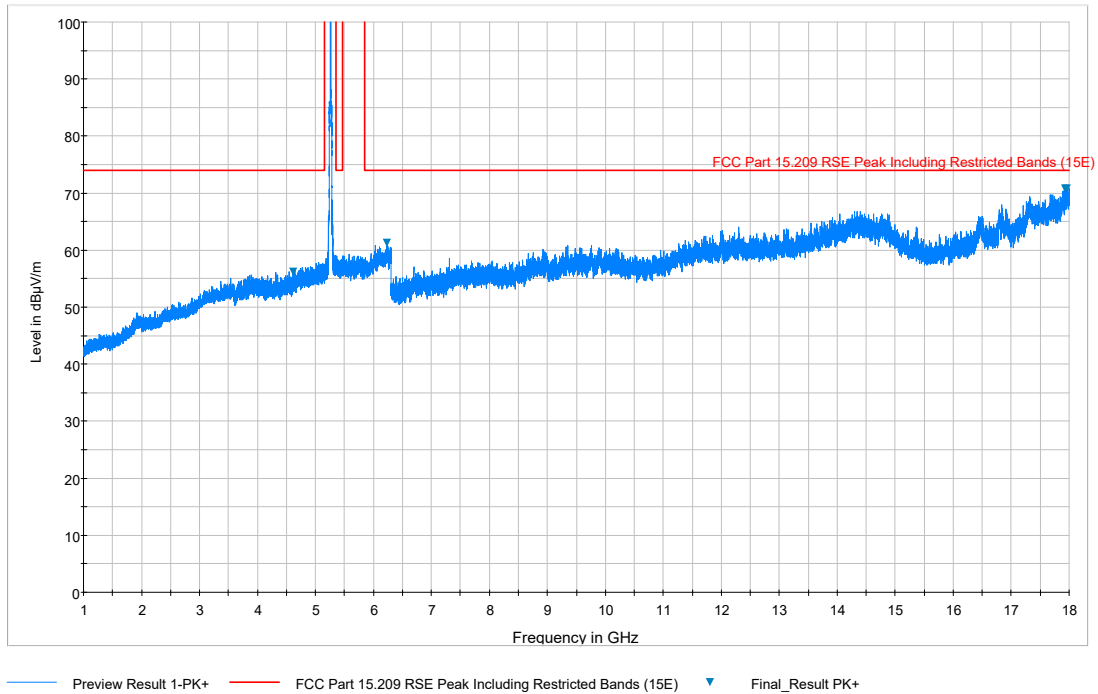
Plot 7-70. Radiated Spurious Plot above 1GHz (802.11a – U2A Ch. 56, Ant. Pol. V)
