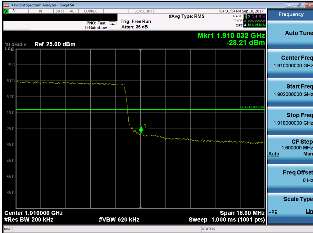
Plot 7-156. Upper Band Edge Plot (Band 2 - 20.0MHz QPSK - Full RB Configuration)
