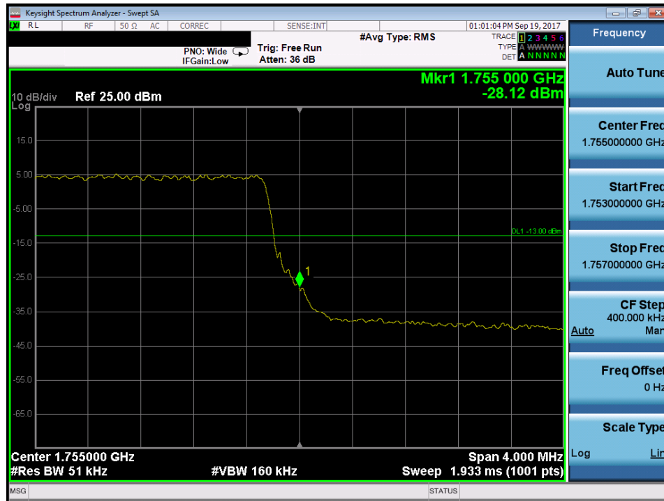
Plot 7-102. Upper Band Edge Plot (Band 4 - 5.0MHz QPSK - Full RB Configuration)
