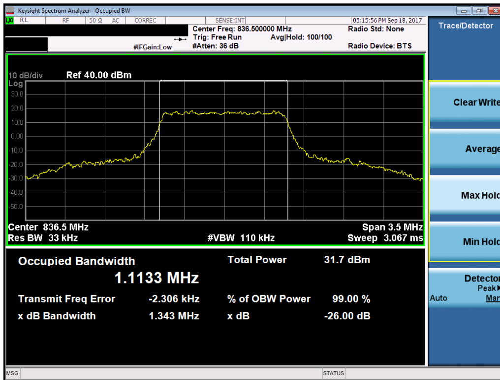
Plot 7-12. Occupied Bandwidth Plot (Band 5 - 1.4MHz 16-QAM - Full RB Configuration)
