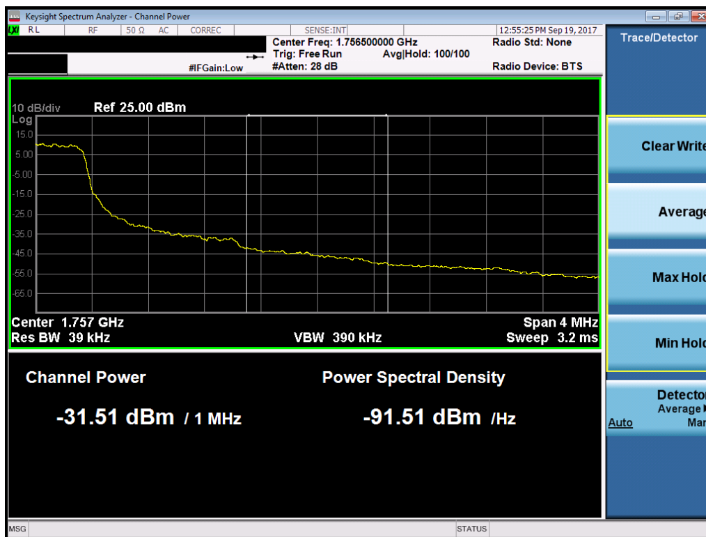
Plot 7-99. . Upper Extended Band Edge Plot (Band 4 - 1.4MHz QPSK - Full RB Configuration)
