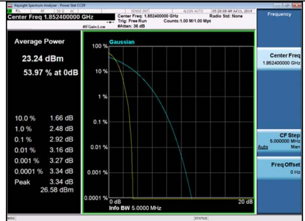
Channel 9262 / 1852.4 MHz
