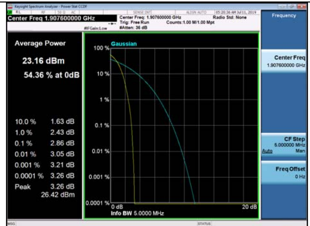
Channel 9538 / 1907.6 MHz
