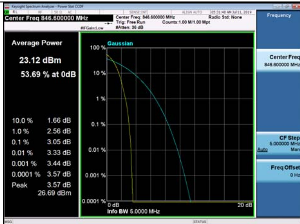
Channel 4233 / 846.6 MHz
