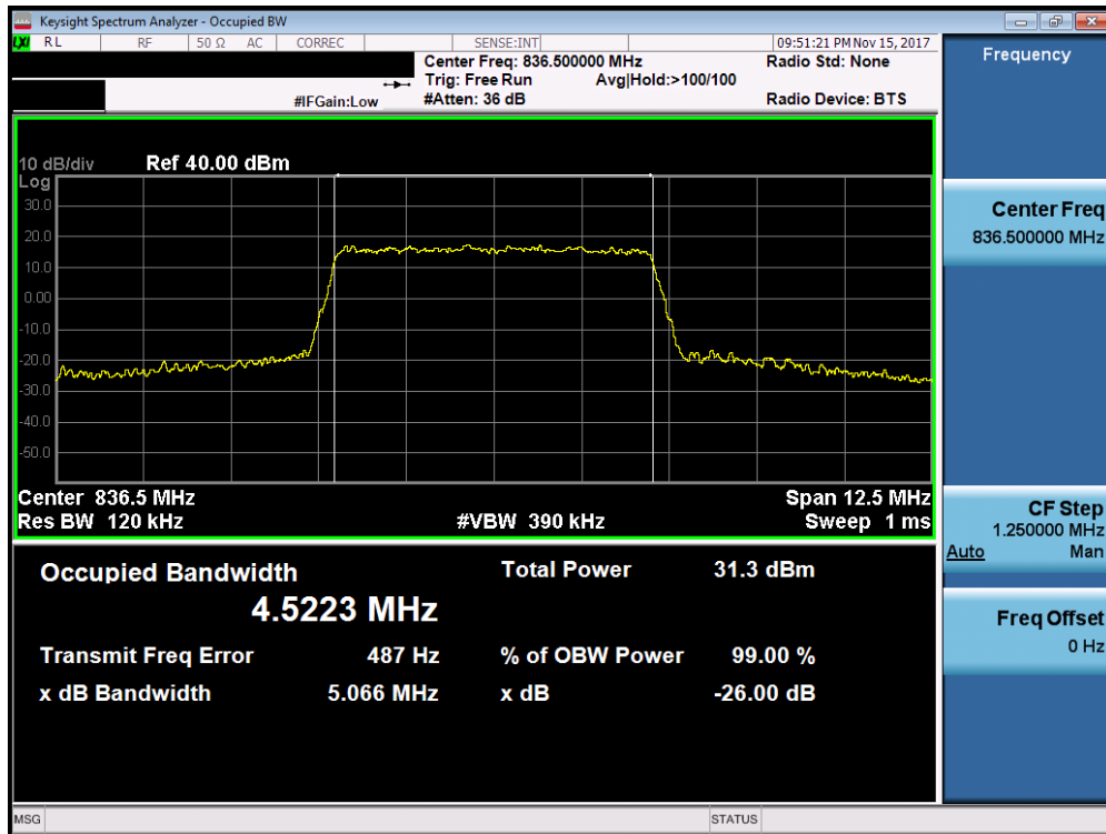
Plot 7-14. Occupied Bandwidth Plot (Band 5 – 5.0MHz QPSK - Full RB Configuration)
