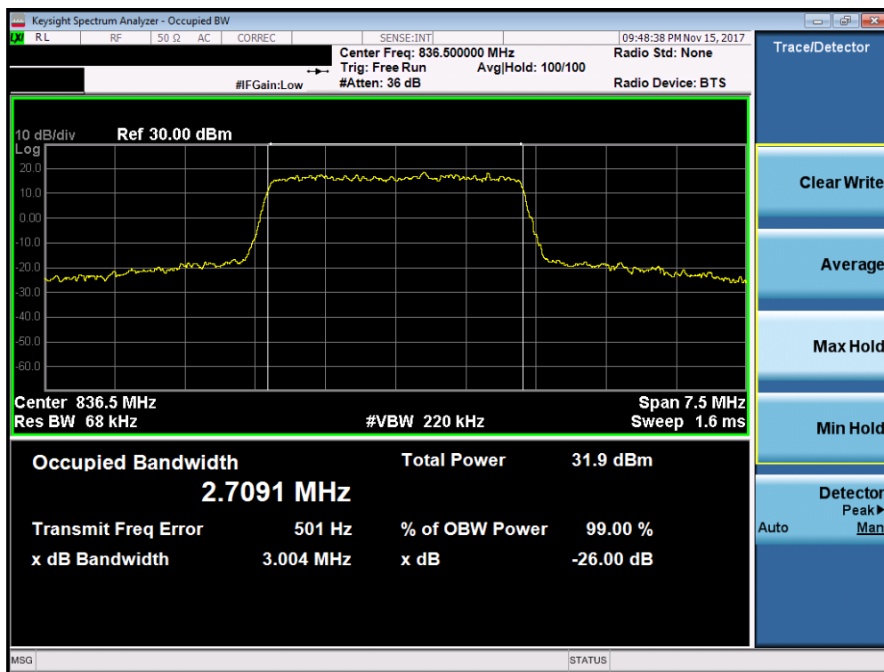
Plot 7-11. Occupied Bandwidth Plot (Band 5 – 3.0MHz QPSK - Full RB Configuration)
