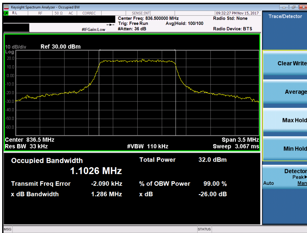
Plot 7-9. Occupied Bandwidth Plot (Band 5 - 1.4MHz QPSK - Full RB Configuration)
