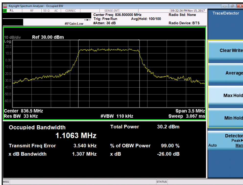
Plot 7-10. Occupied Bandwidth Plot (Band 5 - 1.4MHz QPSK - Full RB Configuration)
