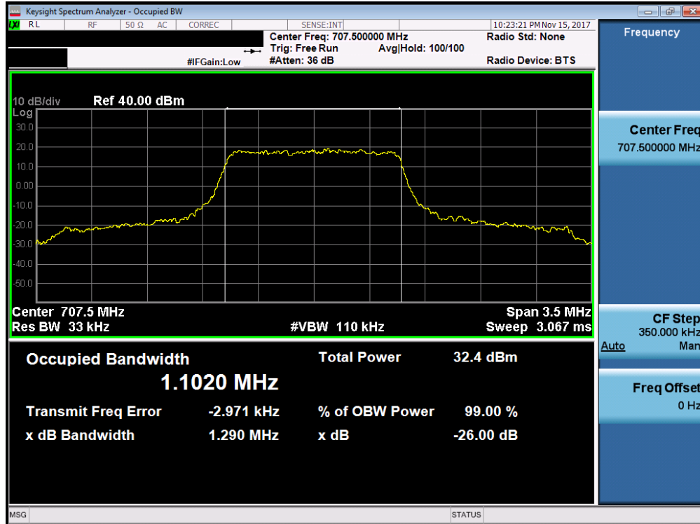
Plot 7-2. Occupied Bandwidth Plot (Band 12 - 1.4MHz QPSK - Full RB Configuration)
