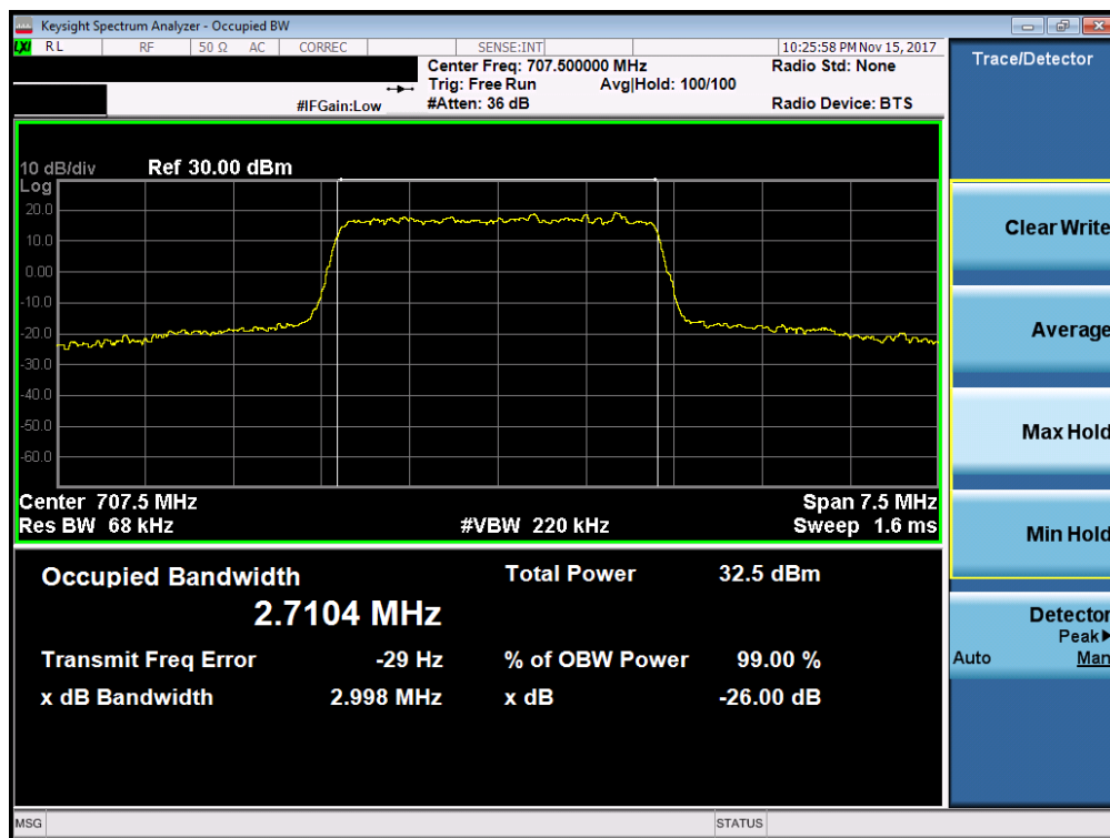
Plotcupied Bandwidth Plot (Band 12 - 3.0MHz QPSK - Full RB Configuration)
