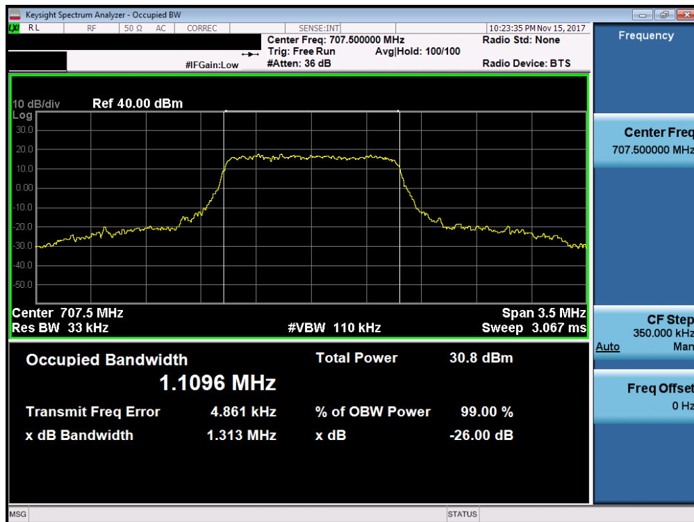
Plot 7-3. Occupied Bandwidth Plot (Band 12 - 1.4MHz 16-QAM - Full RB Configuration)
