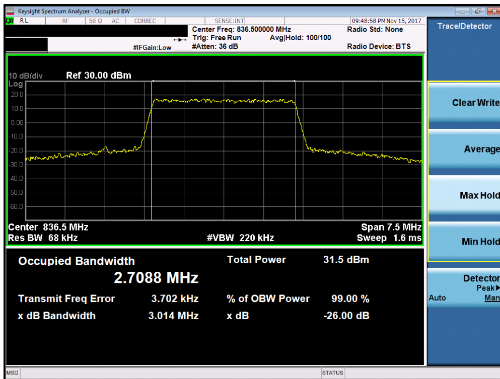
Plot 7-12. Occupied Bandwidth Plot (Band 5 – 3.0MHz QPSK - Full RB Configuration)
