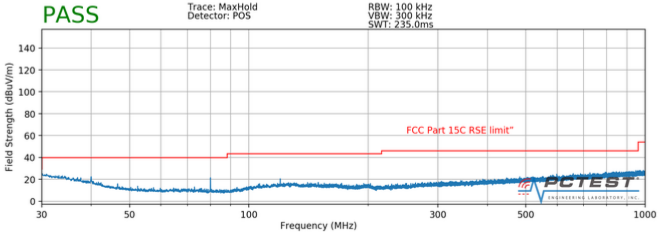
Plot 7-43. Radiated Spurious Plot below 1GHz (Pol. H)
