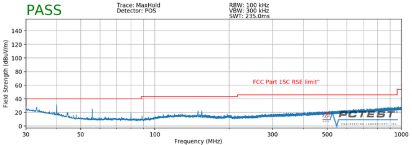
Plot 7-44. Radiated Spurious Plot below 1GHz (Pol. V)
