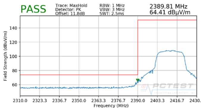
Plot 7-38. Radiated Restricted Lower Band Edge Measurement (Peak)
