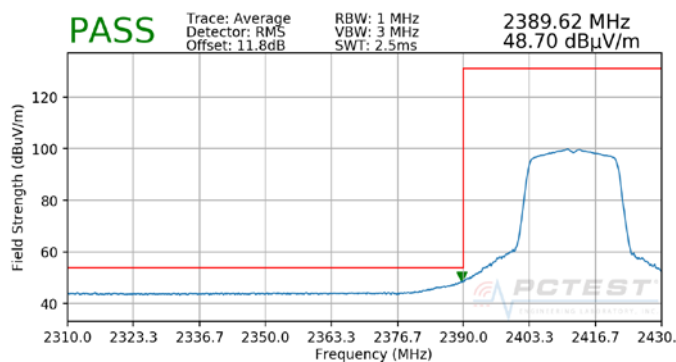
Plot 7-37. Radiated Restricted Lower Band Edge Measurement (Average)
