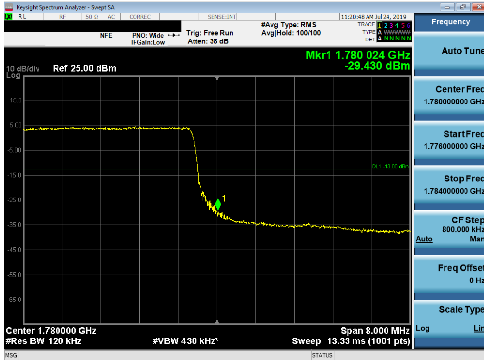
Plot 7-128. Upper Band Edge Plot (Band 66 - 10.0MHz QPSK - Full RB Configuration)
