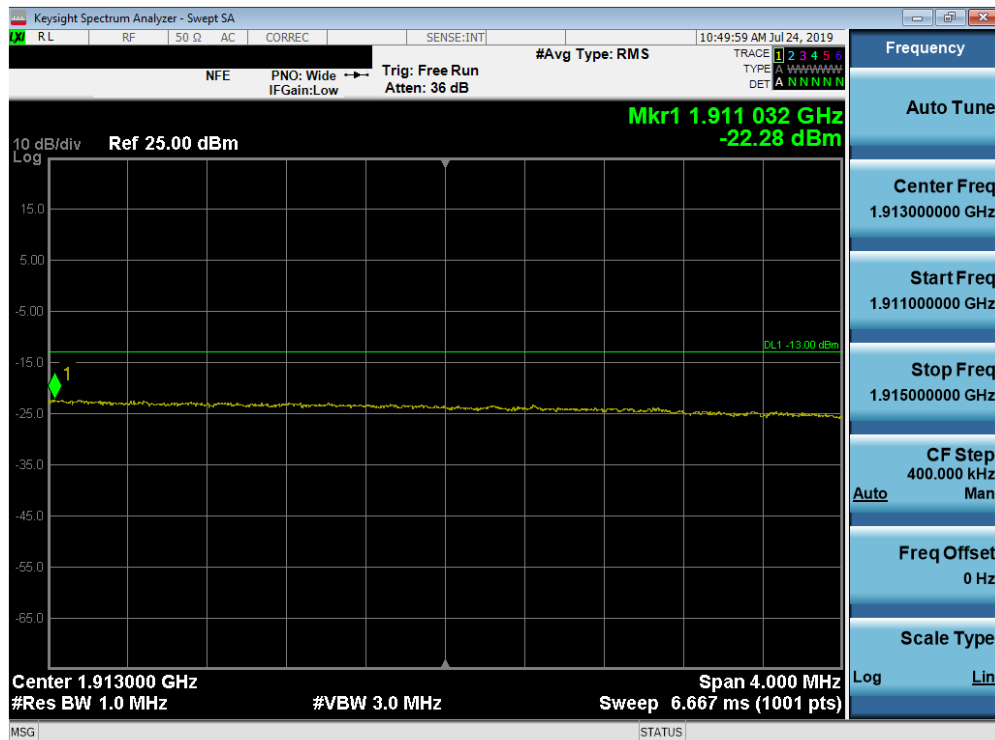
Plot 7-165. Upper Extended Band Edge Plot (Band 2 - 20.0MHz QPSK - Full RB Configuration)
