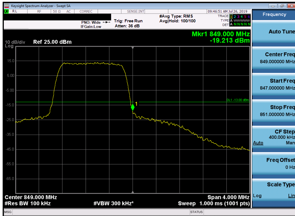
Plot 7-99. Upper Band Edge Plot (Band 5 - 1.4MHz QPSK - Full RB Configuration)
