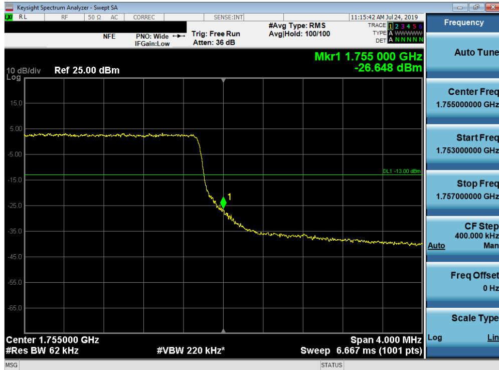
Plot 7-120. Upper Band Edge Plot (Band 4 - 5.0MHz QPSK - Full RB Configuration)
