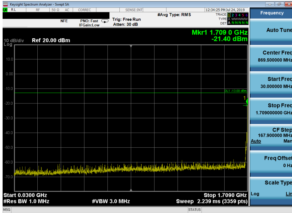
Plot 7-66. Conducted Spurious Plot (Band 66/4 - 20.0MHz QPSK - RB Size 1, RB Offset 0 - Low Channel)
