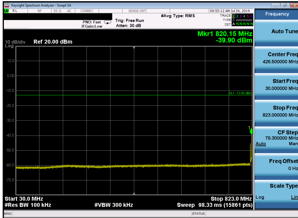
Plot 7-57. Conducted Spurious Plot (Band 5 - 10.0MHz QPSK - RB Size 1, RB Offset 0 - Low Channel)
