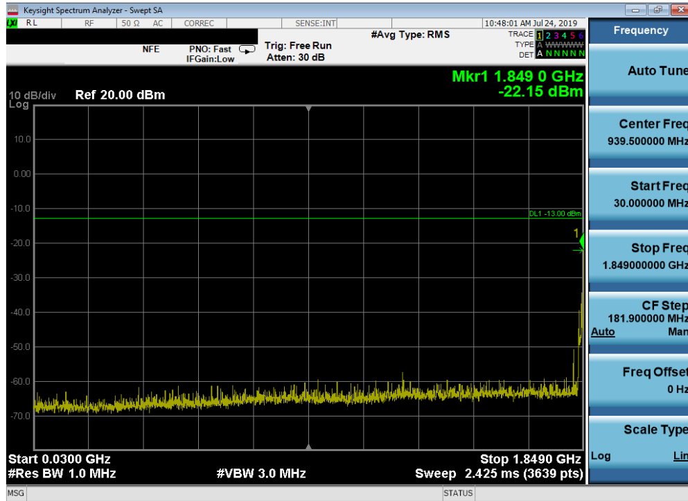
Plot 7-75. Conducted Spurious Plot (Band 2 - 20.0MHz QPSK - RB Size 1, RB Offset 0 - Low Channel)
