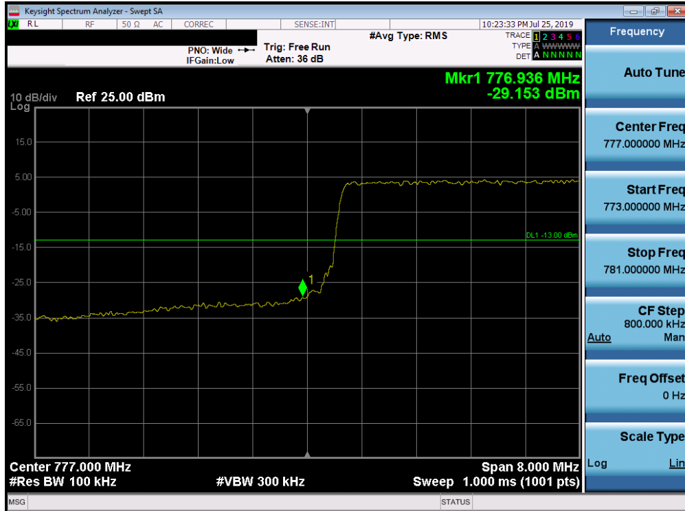
Plot 7-96. Lower Band Edge Plot (Band 13 - 10.0MHz QPSK - Full RB Configuration)
