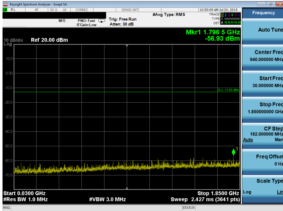
Plot 7-81. Conducted Spurious Plot (Band 2 - 20.0MHz QPSK - RB Size 1, RB Offset 0 - High Channel)
