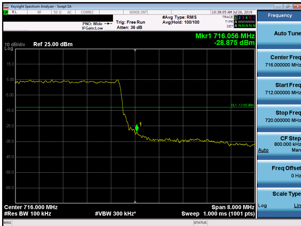
Plot 7-93. Upper Band Edge Plot (Band 12/17 - 10.0MHz QPSK - Full RB Configuration)
