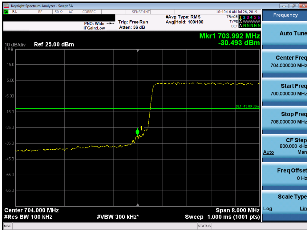
Plot 7-92. Lower Band Edge Plot (Band 17 - 10.0MHz QPSK - Full RB Configuration)
