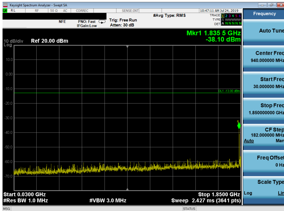
Plot 7-78. Conducted Spurious Plot (Band 2 - 20.0MHz QPSK - RB Size 1, RB Offset 0 - Mid Channel)
