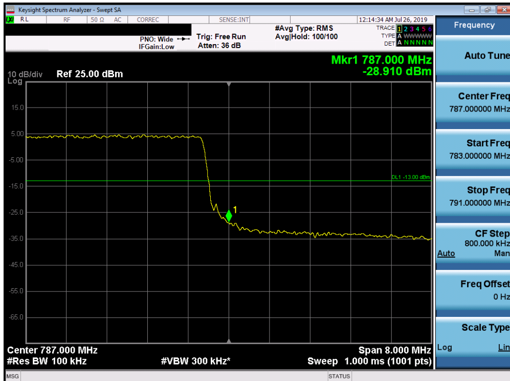
Plot 7-97. Upper Band Edge Plot (Band 13 - 10.0MHz QPSK - Full RB Configuration)
