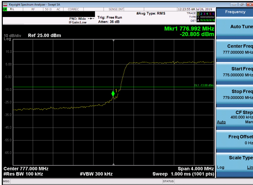
Plot 7-94. Lower Band Edge Plot (Band 13 - 5.0MHz QPSK - Full RB Configuration)
