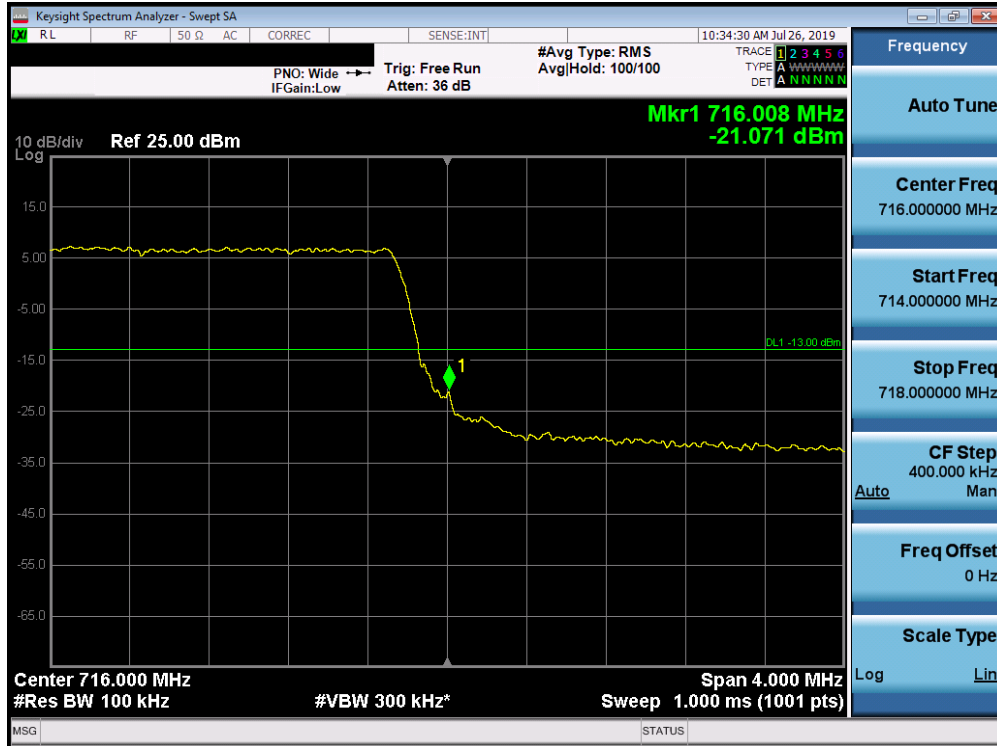
Plot 7-90. Upper Band Edge Plot (Band 12/17 - 5.0MHz QPSK - Full RB Configuration)
