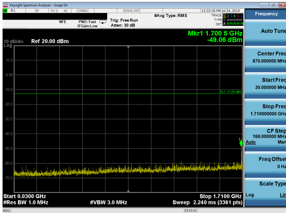
Plot 7-69. Conducted Spurious Plot (Band 66/4 - 20.0MHz QPSK - RB Size 1, RB Offset 0 - Mid Channel)
