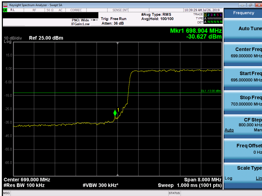
Plot 7-91. Lower Band Edge Plot (Band 12 - 10.0MHz QPSK - Full RB Configuration)
