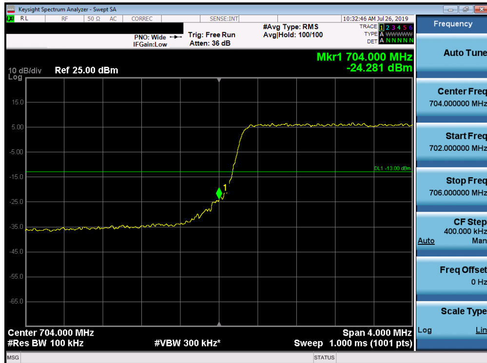
Plot 7-89. Lower Band Edge Plot (Band 17 - 5.0MHz QPSK - Full RB Configuration)
