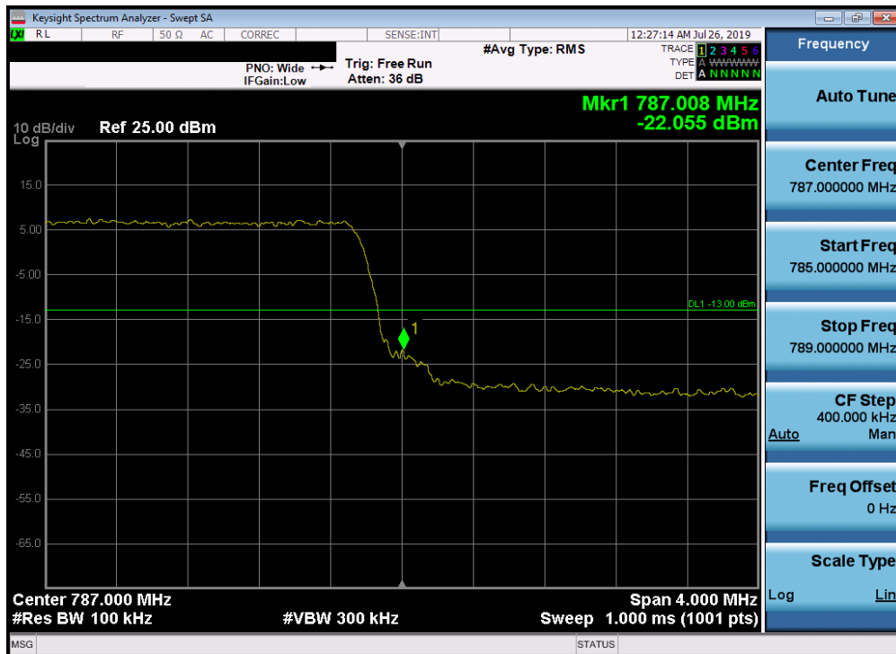
Plot 7-95. Upper Band Edge Plot (Band 13 - 5.0MHz QPSK - Full RB Configuration)
