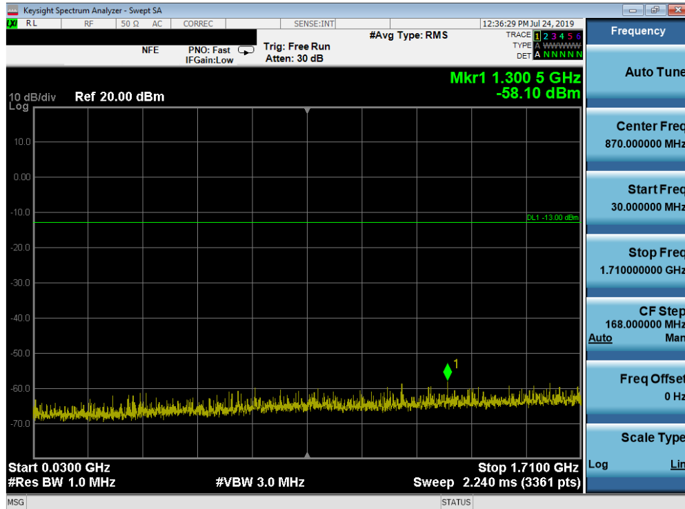
Plot 7-72. Conducted Spurious Plot (Band 66/4 - 20.0MHz QPSK - RB Size 1, RB Offset 0 - High Channel)
