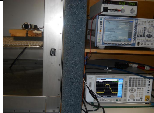
FREQUENCY STABILITY
