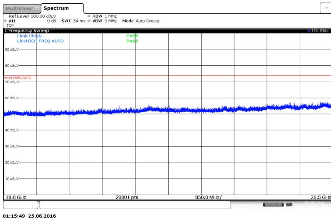
Plot 7-20. Radiated Spurious Plot above 18GHz (802.11a – Ant. Pol. V)
