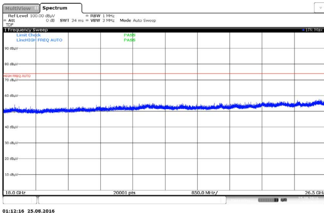
Plot 7-19. Radiated Spurious Plot above 18GHz (802.11a – Ant. Pol. H)
