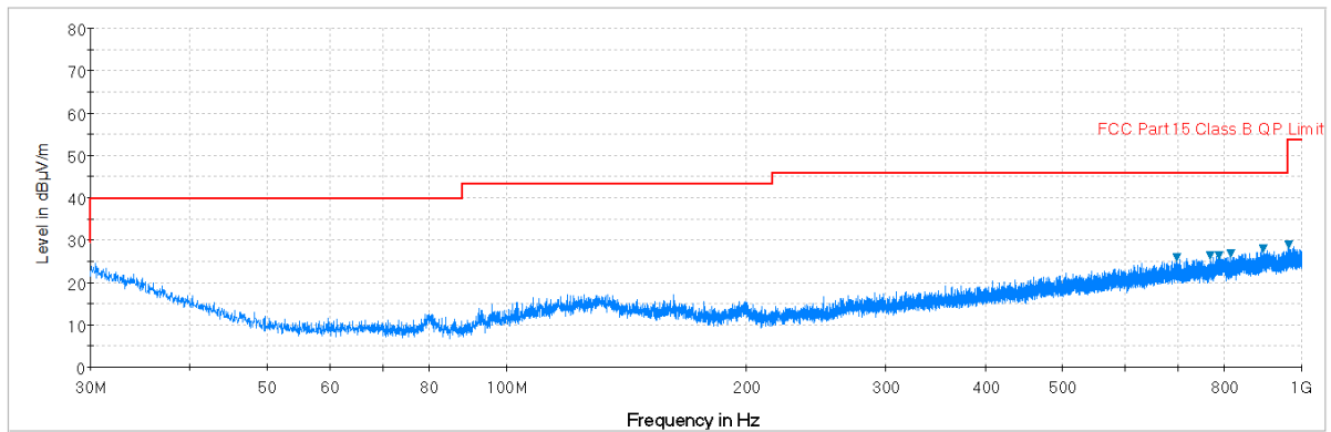
Plot 7-58. Radiated Spurious Plot below 1GHz (802.11a – U3 Ch. 157, Ant. Pol. V)
