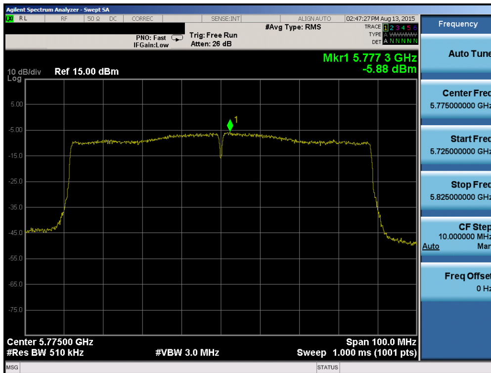
Plot 6-76. Power Spectral Density Plot (80MHz BW 802.11ac (UNII Band 3) – Ch. 155)
