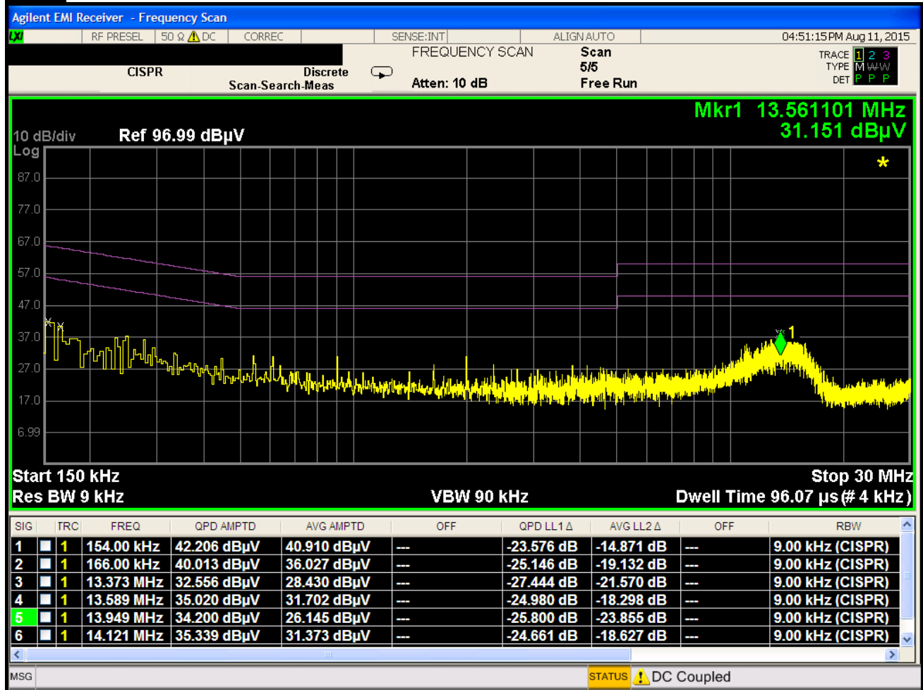
Plot 6-129. Line Conducted Plot with 802.11a UNII Band 2A (N)
