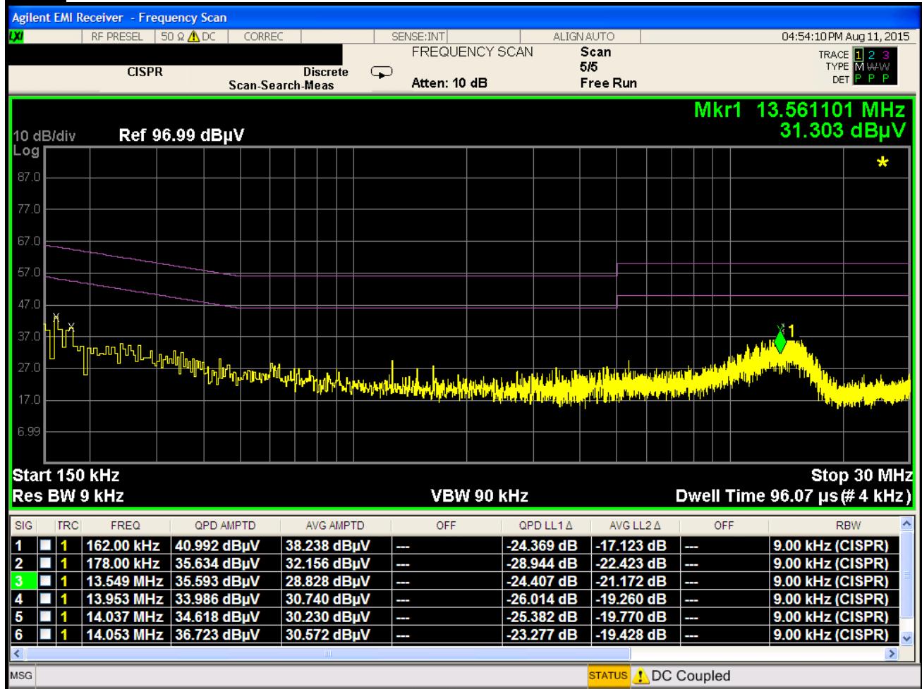
Plot 6-131. Line Conducted Plot with 802.11a UNII Band 2C (N)
