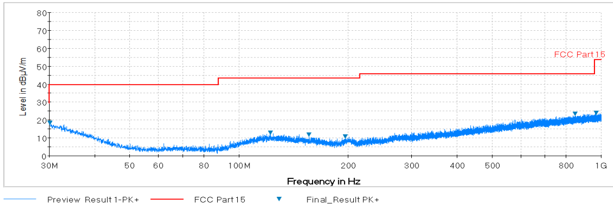
Plot 6-124. Radiated Spurious Plot below 1GHz (802.11a – U3 Ch. 157, Ant. Pol. H)
