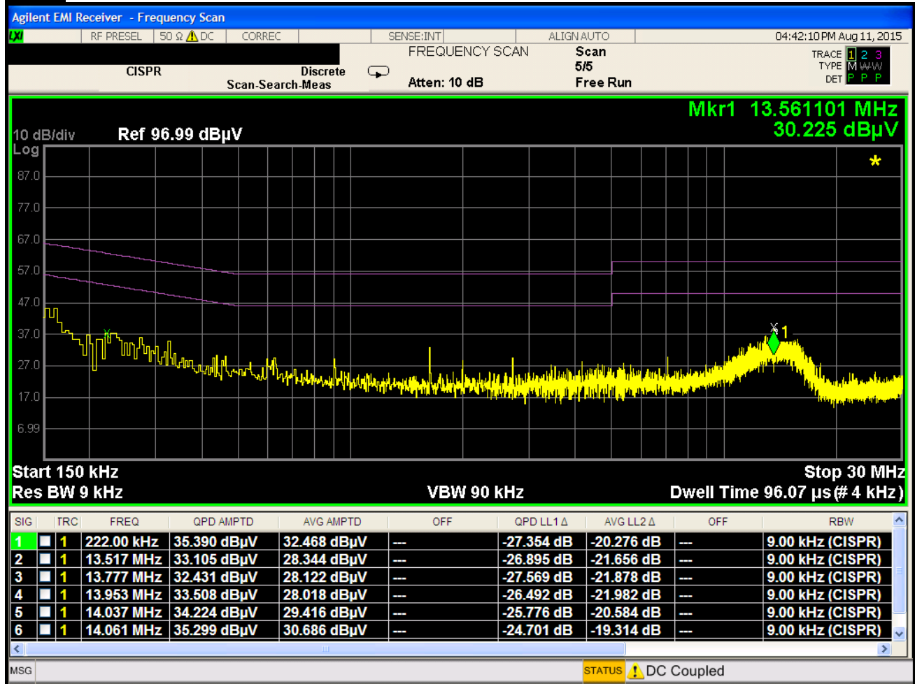
Plot 6-127. Line Conducted Plot with 802.11a UNII Band 1 (N)
