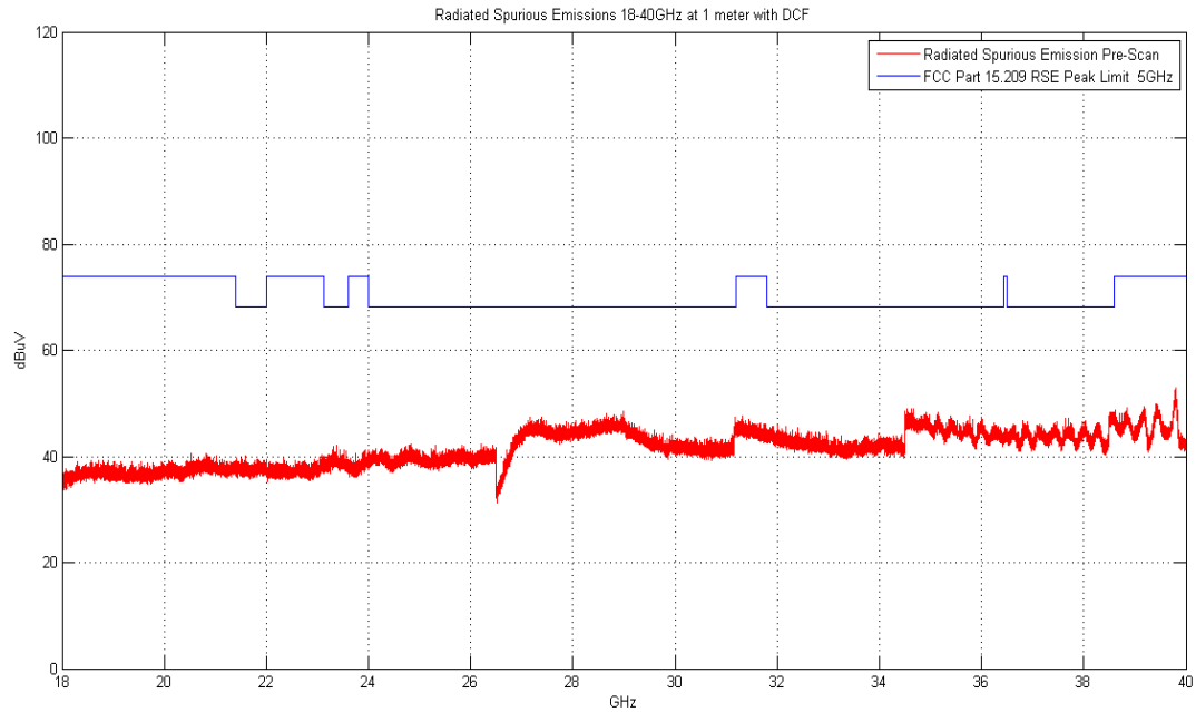
Plot 6-85. Radiated Spurious Plot above 18GHz (802.11a – Ant. Pol. H)
