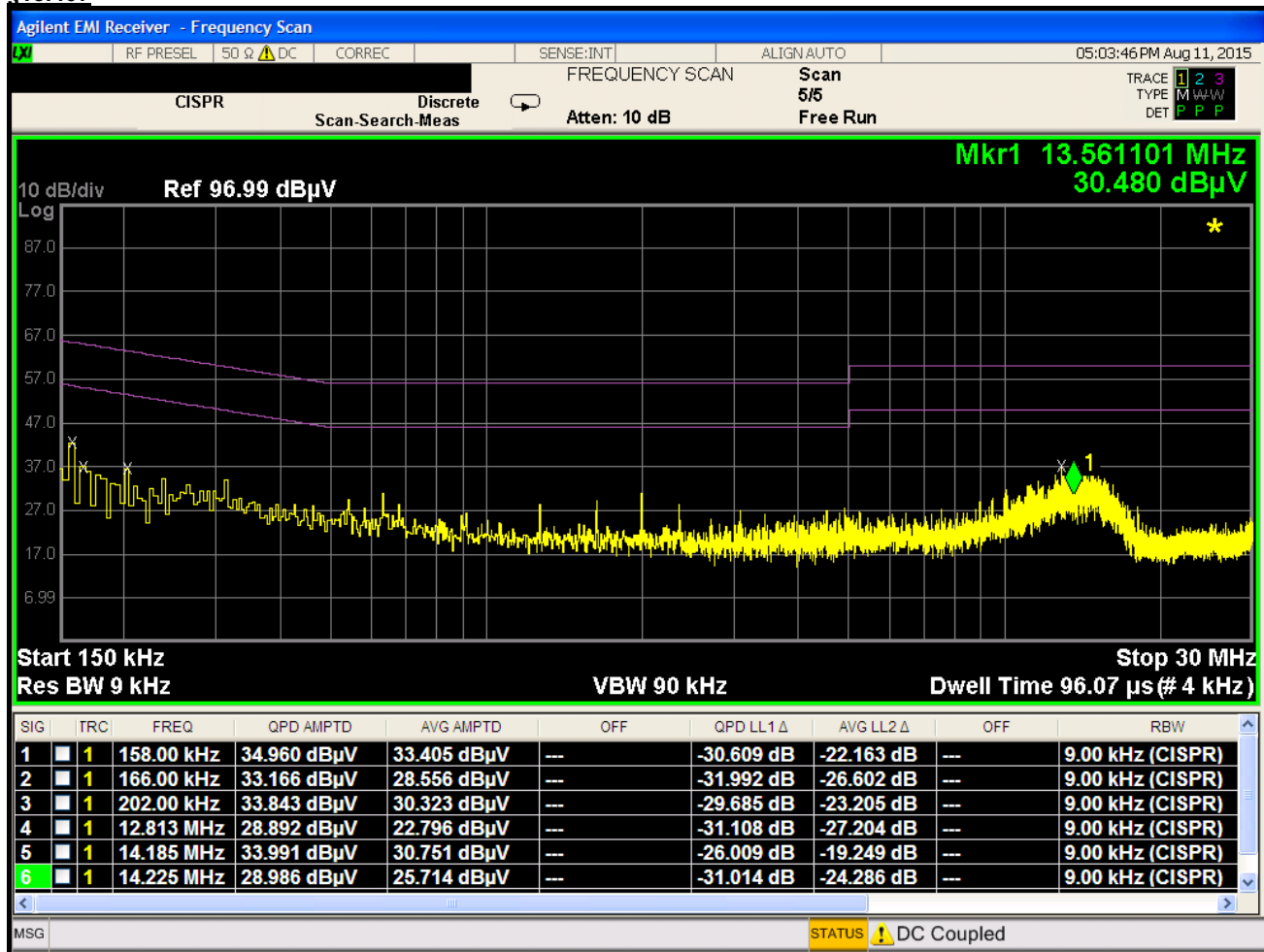
Plot 6-133. Line Conducted Plot with 802.11a UNII Band 3 (N)
