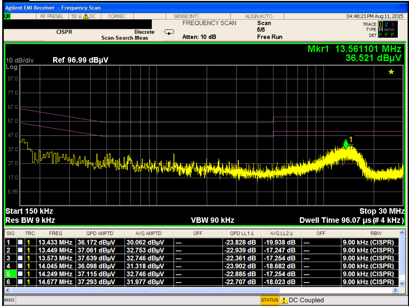
Plot 6-128. Line Conducted Plot with 802.11a UNII Band 2A (L1)
