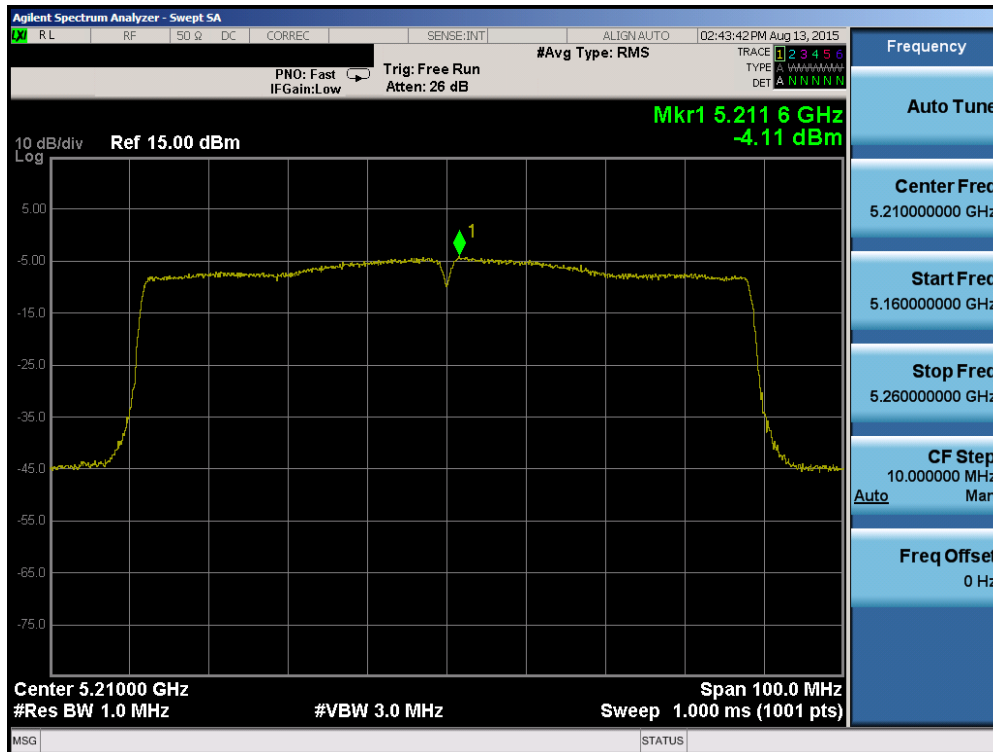
Plot 6-47. Power Spectral Density Plot (80MHz BW 802.11ac (UNII Band 1) – Ch. 42)
