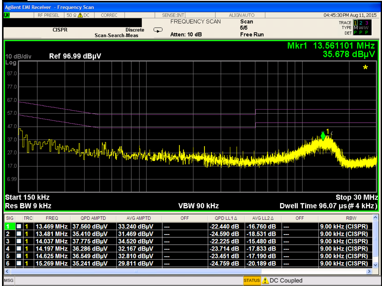
Plot 6-126. Line Conducted Plot with 802.11a UNII Band 1 (L1)
