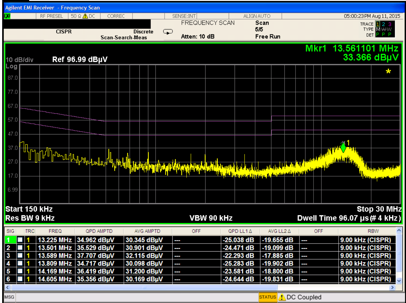
Plot 6-132. Line Conducted Plot with 802.11a UNII Band 3 (L1)
