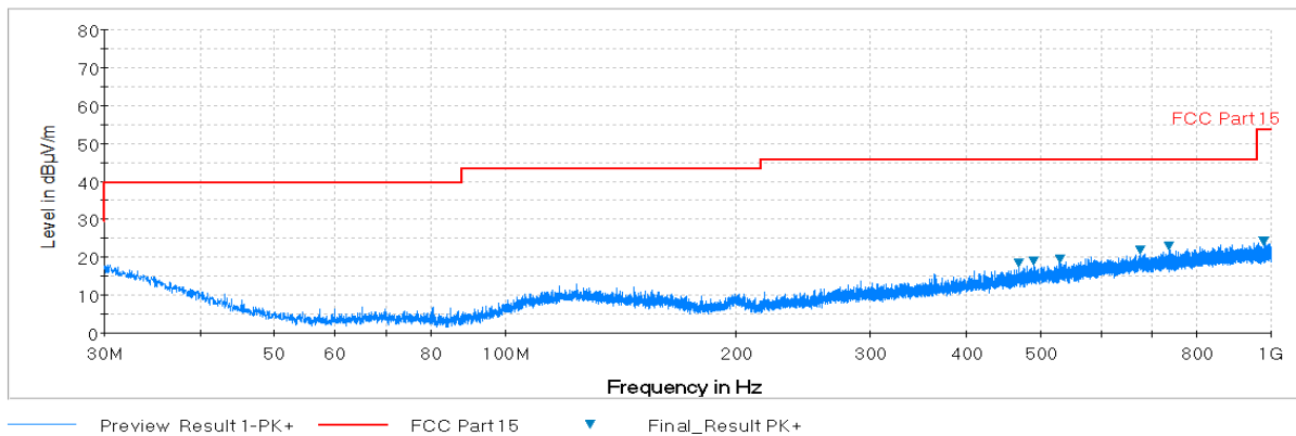
Plot 6-125. Radiated Spurious Plot below 1GHz (802.11a – U3 Ch. 157, Ant. Pol. V)
