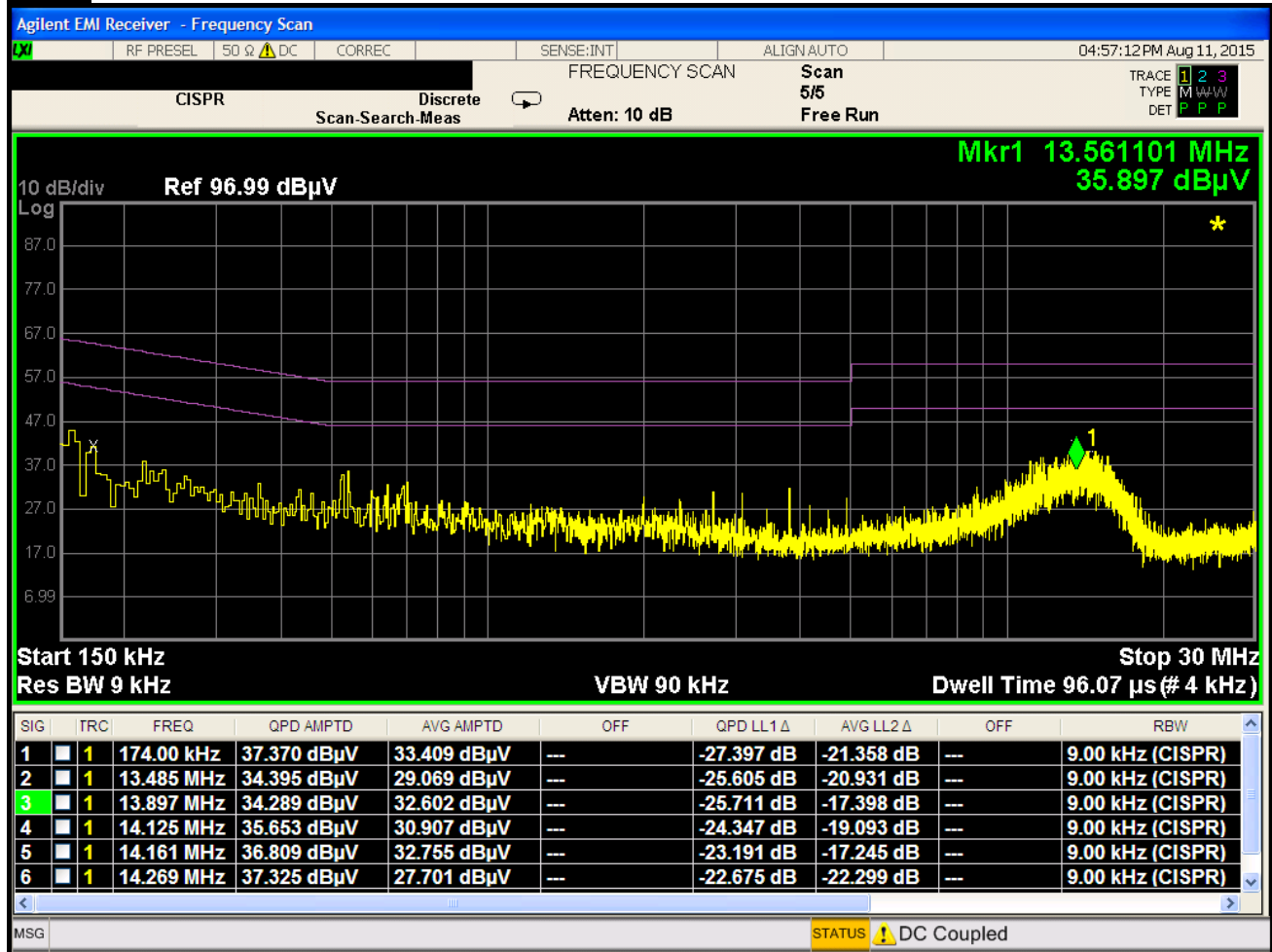
Plot 6-130. Line Conducted Plot with 802.11a UNII Band 2C (L1)
