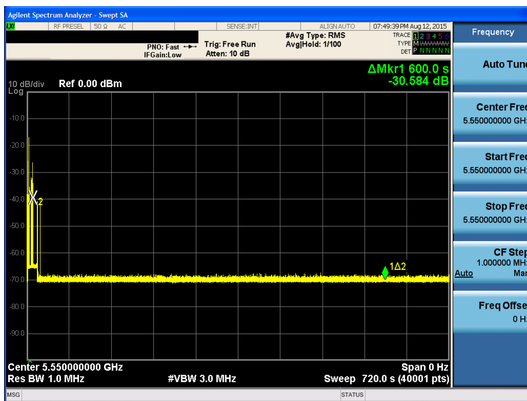
Figure 5-8. Band 2C Non-occupancy Period - Monitoring live spectrum - Elapsed time 10 minutes
