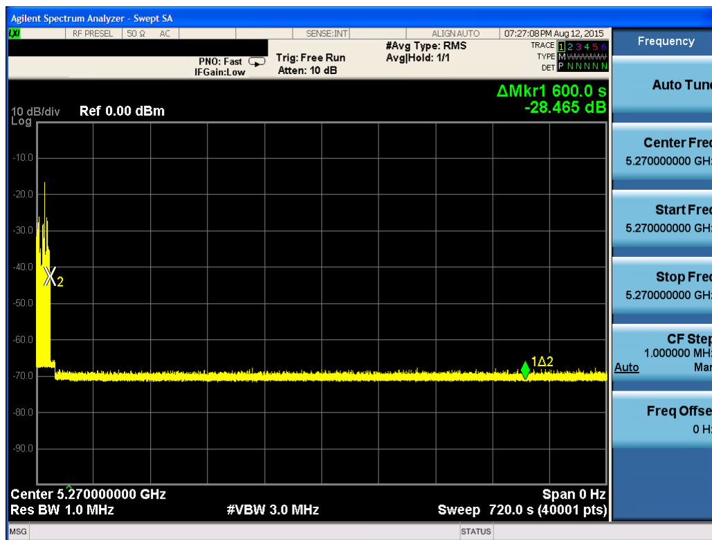
Figure 5-7. Band 2A Non-occupancy Period - Monitoring live spectrum - Elapsed time 10 minutes
