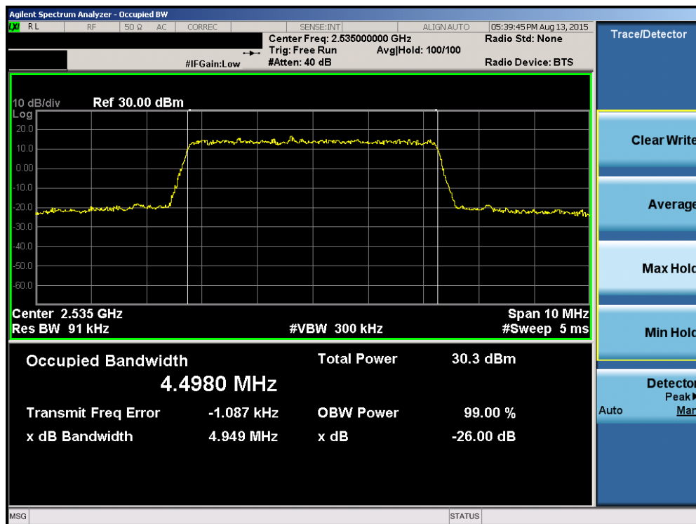
Plot 6-38. Occupied Bandwidth Plot (Band 7 – 5.0MHz 16-QAM – RB Size 25)
