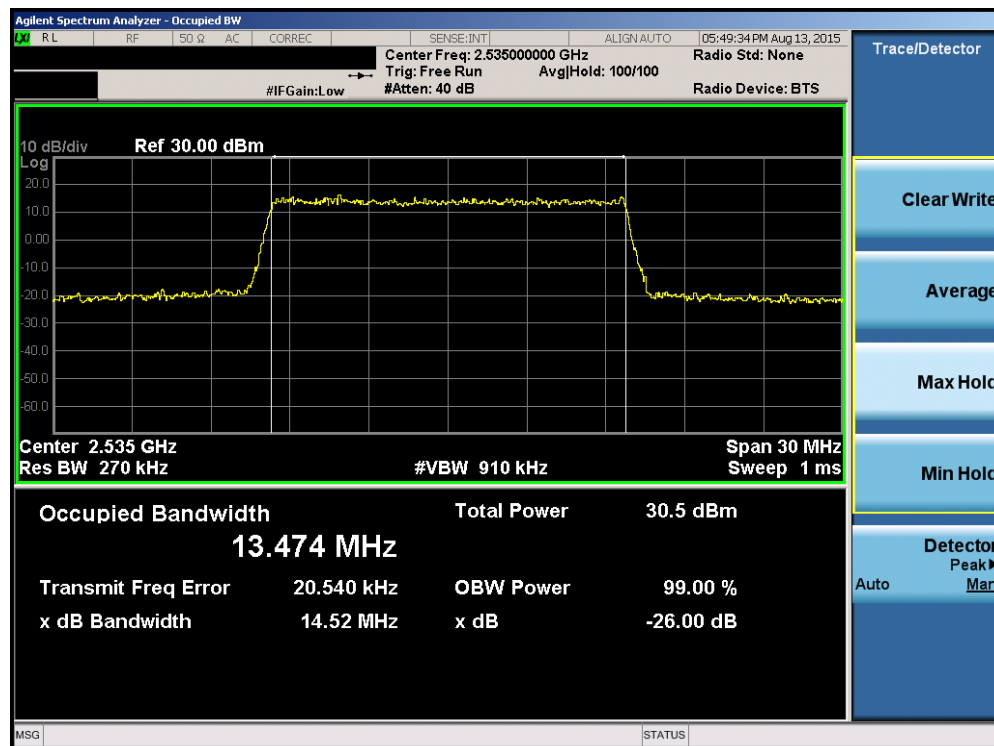
Plot 6-42. Occupied Bandwidth Plot (Band 7 – 15.0MHz 16-QAM – RB Size 75)
