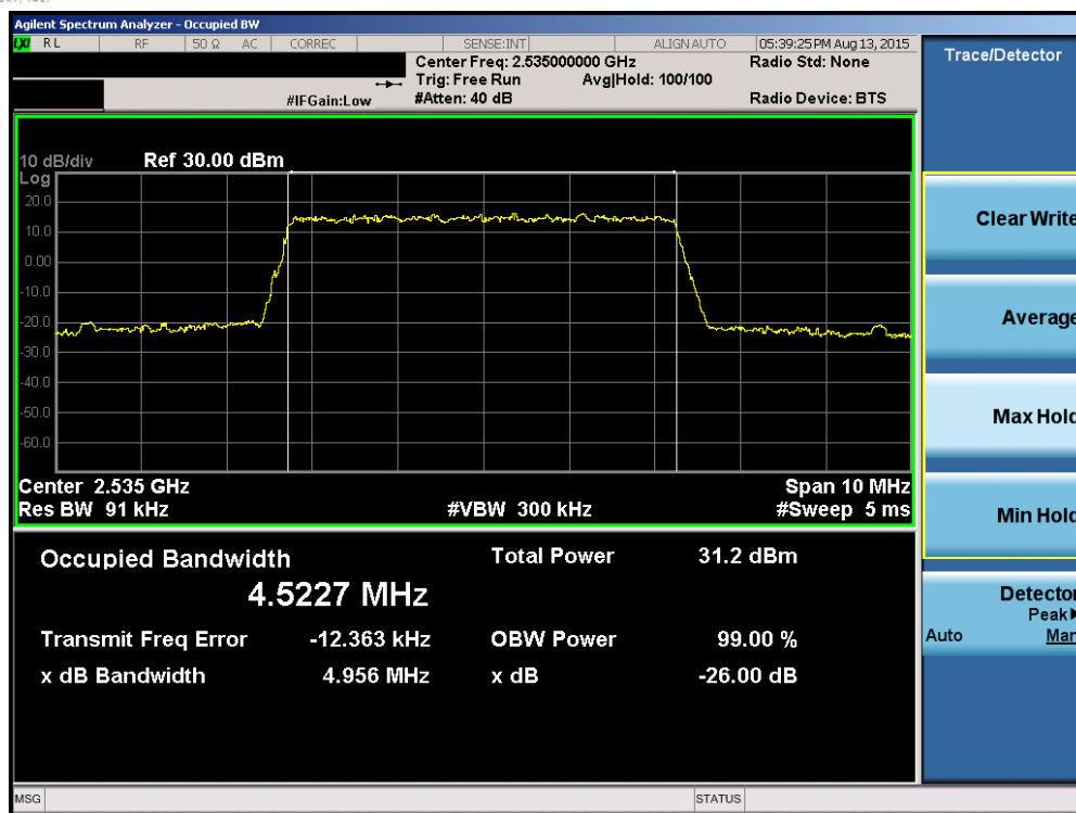
Plot 6-37. Occupied Bandwidth Plot (Band 7 – 5.0MHz QPSK – RB Size 25)
