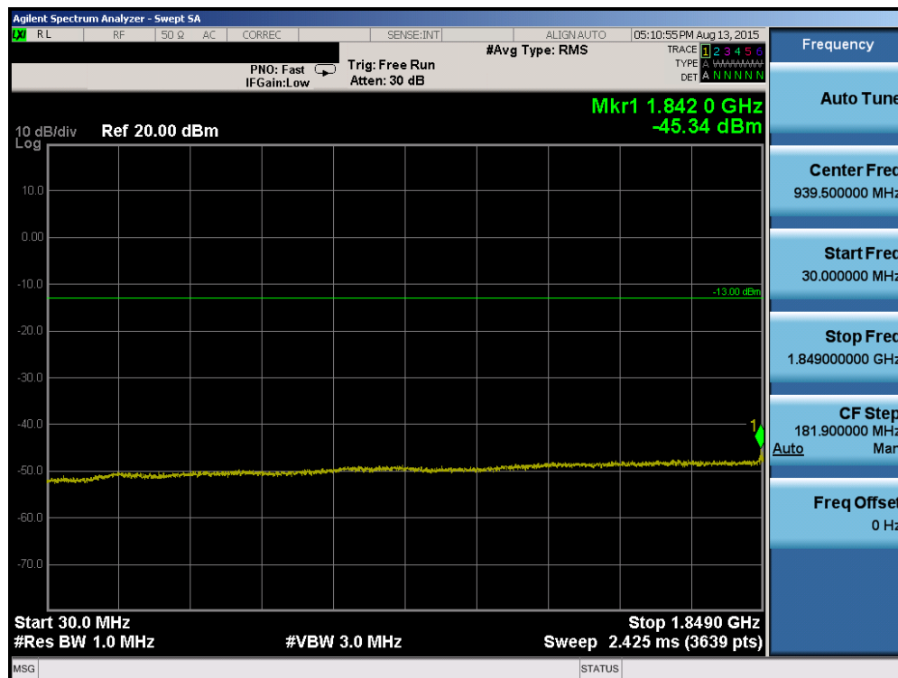
Plot 6-72. Conducted Spurious Plot (Band 2 – 10.0MHz QPSK – RB Size 1, RB Offset 0– Low Channel)
