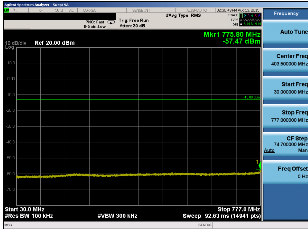
Plot 6-51. Conducted Spurious Plot (Band 13 – 5.0MHz QPSK – RB Size 1, RB Offset 0 – High Channel)
