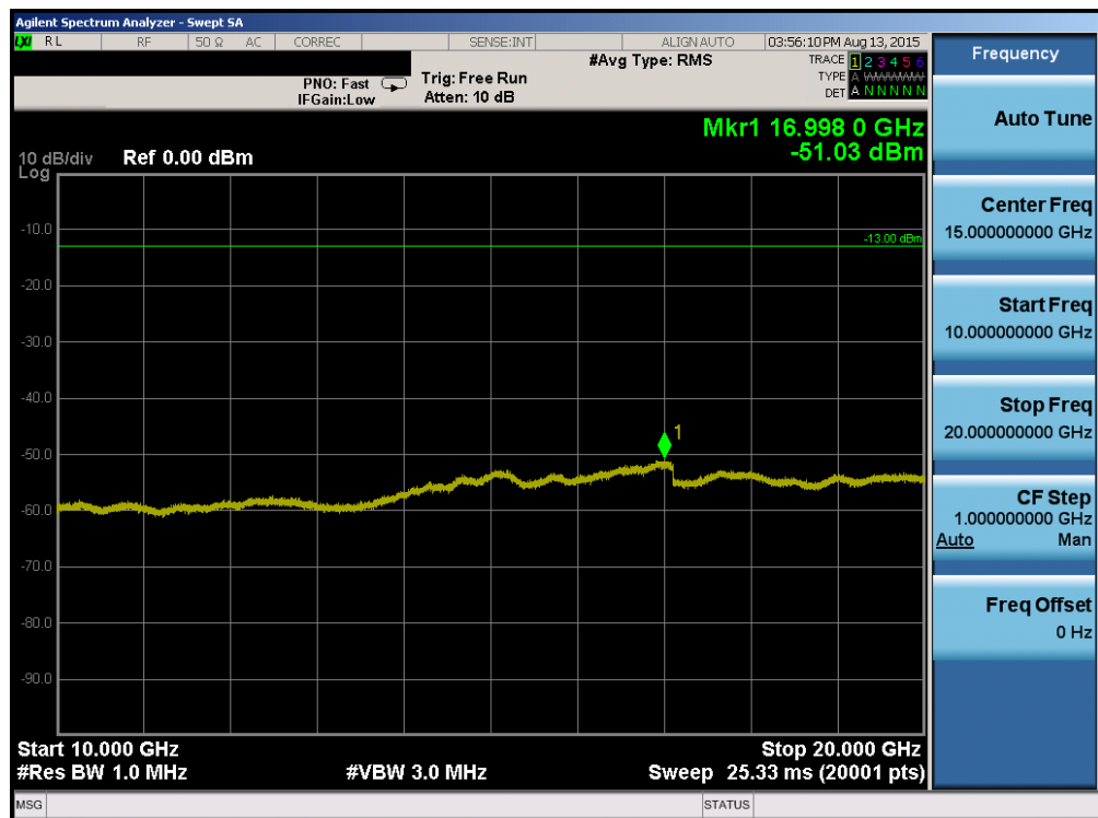
Plot 6-68. Conducted Spurious Plot (Band 4 – 1.4MHz QPSK – RB Size 1, RB Offset 0 – Mid Channel)
