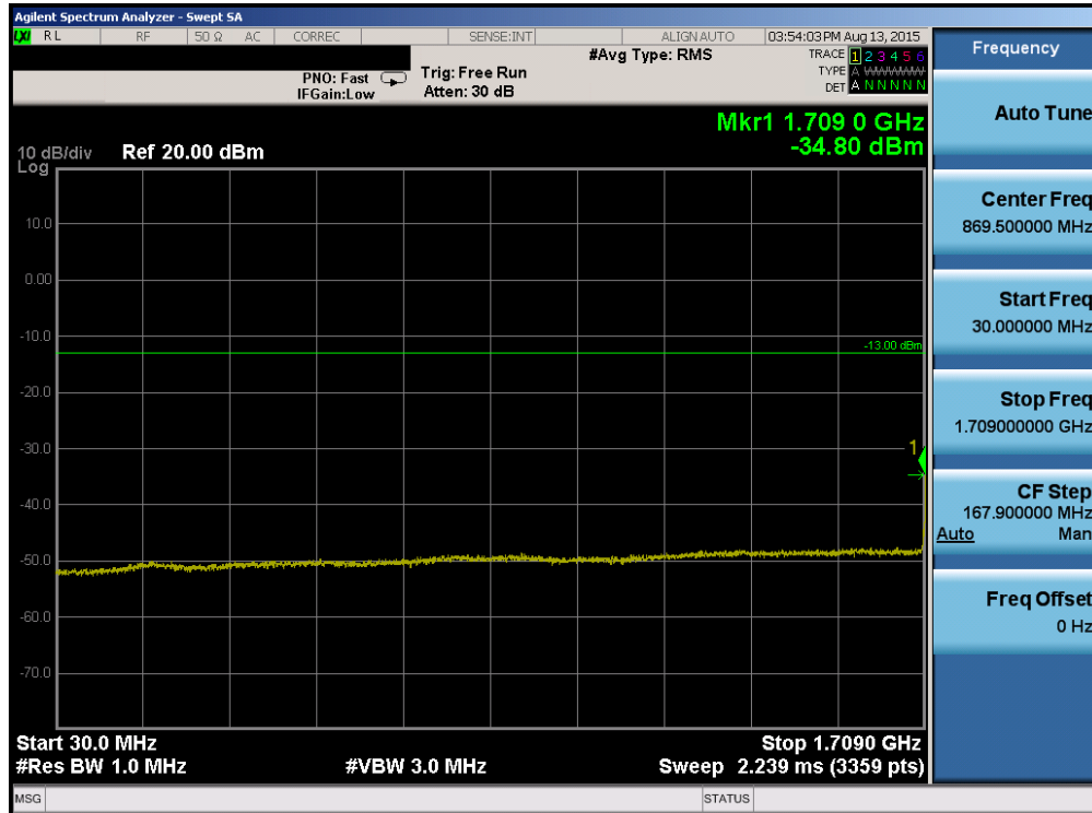
Plot 6-63. Conducted Spurious Plot (Band 4 – 1.4MHz QPSK – RB Size 1, RB Offset 0 – Low Channel)
