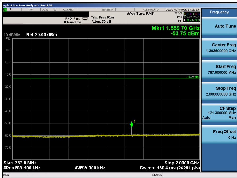
Plot 6-49. Conducted Spurious Plot (Band 13 – 5.0MHz QPSK – RB Size 1, RB Offset 0 – Mid Channel)
