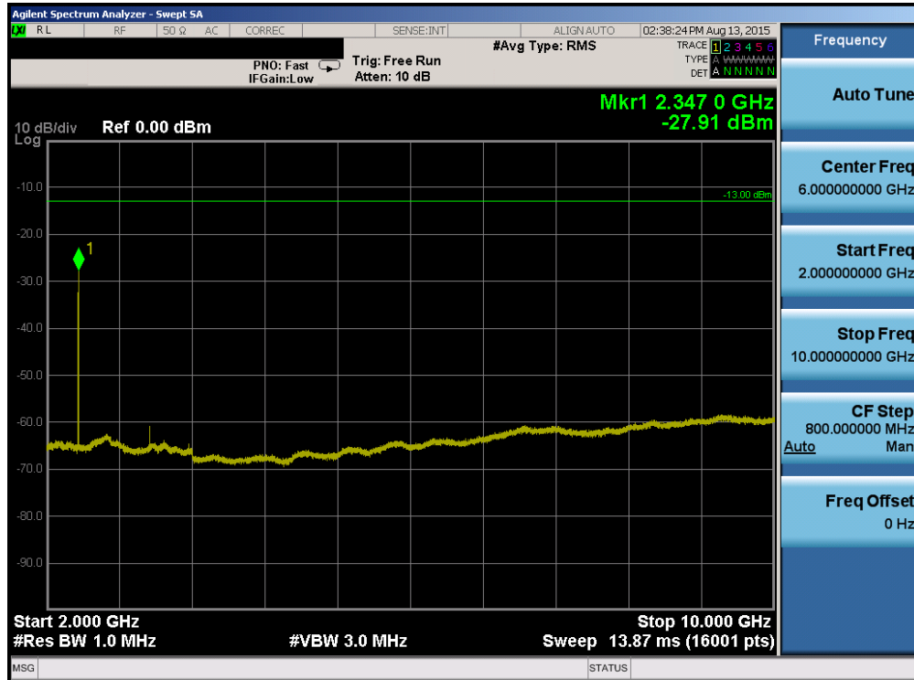
Plot 6-53. Conducted Spurious Plot (Band 13 – 5.0MHz QPSK – RB Size 1, RB Offset 0 – High Channel)
