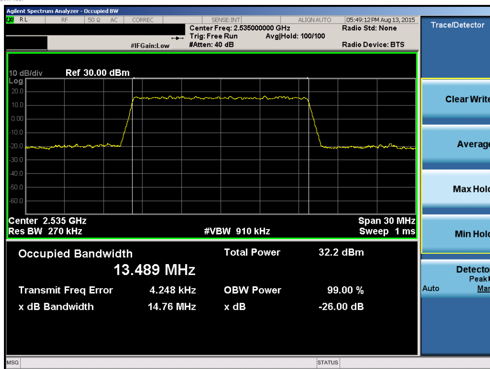
Plot 6-41. Occupied Bandwidth Plot (Band 7 – 15.0MHz QPSK – RB Size 75)
