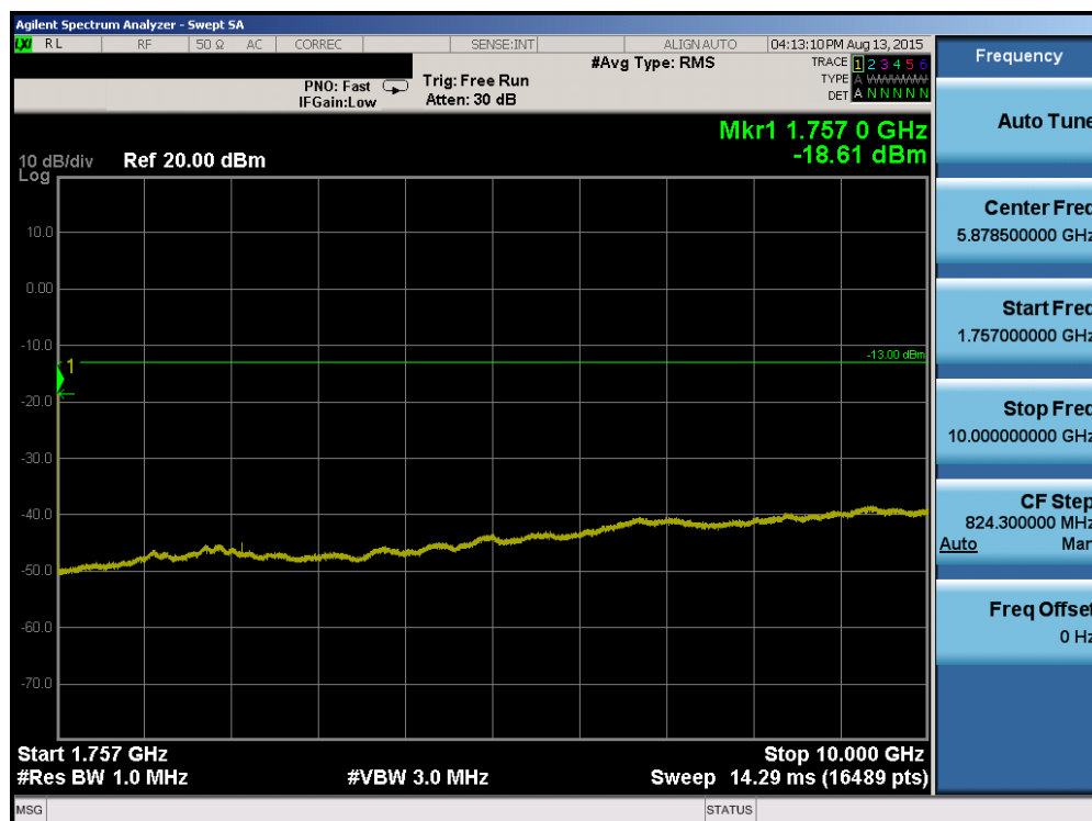
Plot 6-70. Conducted Spurious Plot (Band 4 – 1.4MHz QPSK – RB Size 1, RB Offset 0 – High Channel)
