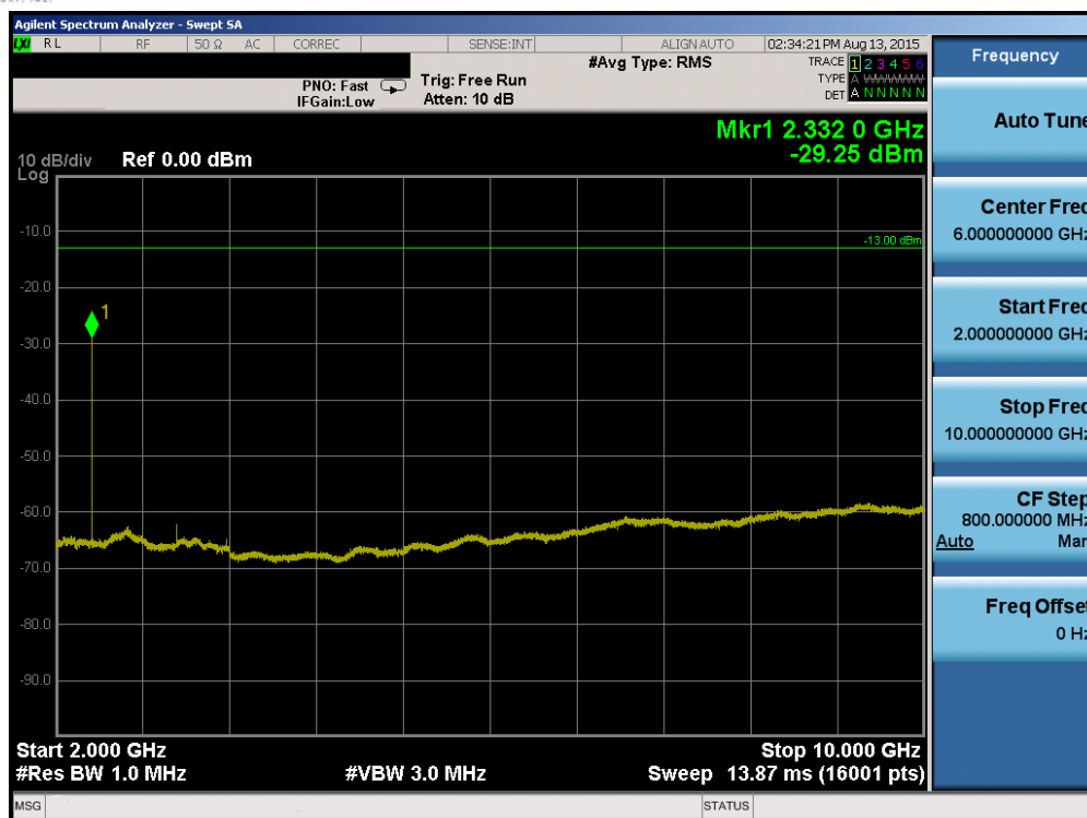
Plot 6-47. Conducted Spurious Plot (Band 13 – 5.0MHz QPSK – RB Size 1, RB Offset 0 – Low Channel)
