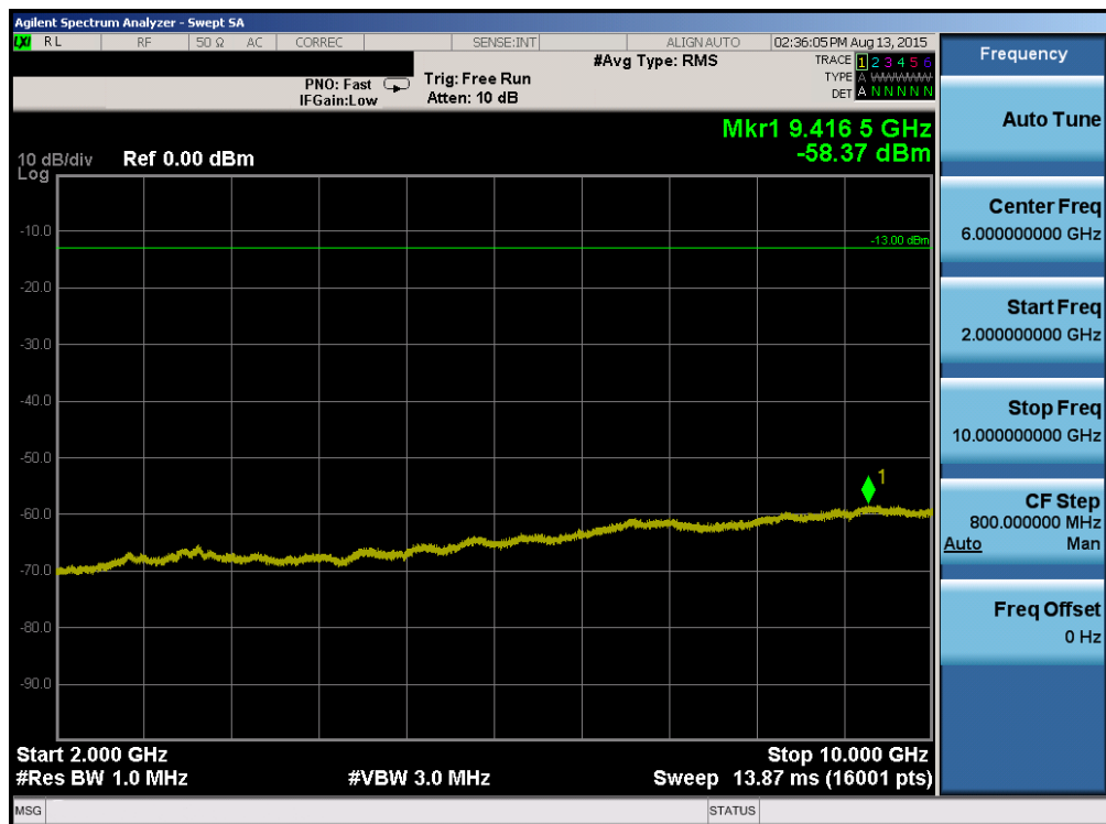
Plot 6-50. Conducted Spurious Plot (Band 13 – 5.0MHz QPSK – RB Size 1, RB Offset 0 – Mid Channel)
