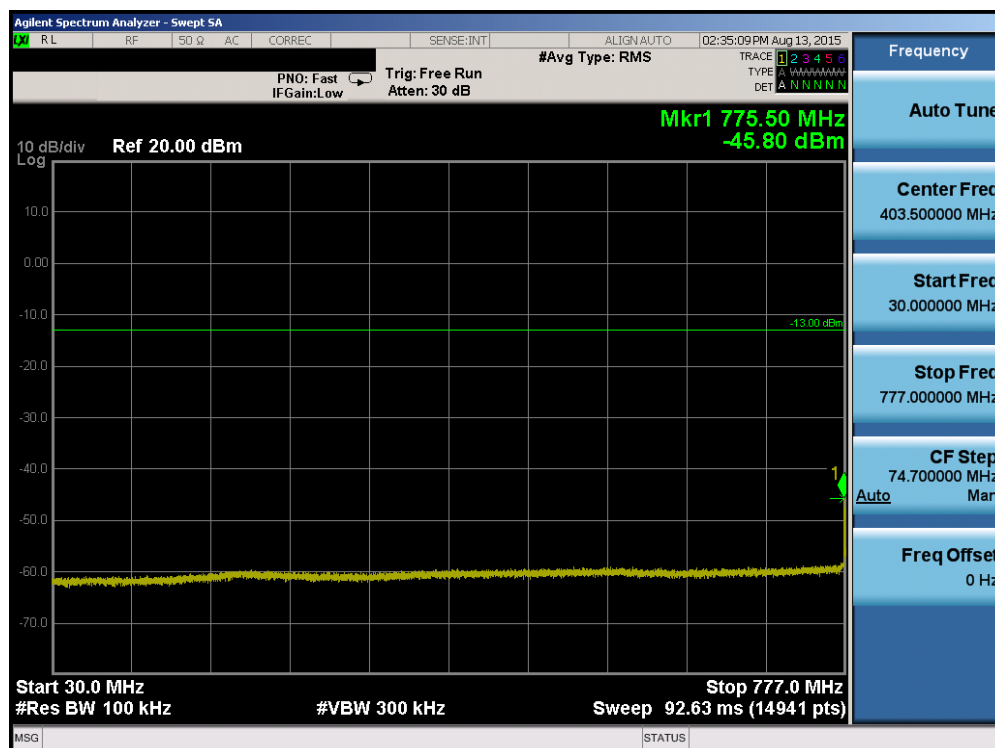
Plot 6-48. Conducted Spurious Plot (Band 13 – 5.0MHz QPSK – RB Size 1, RB Offset 0 – Mid Channel)
