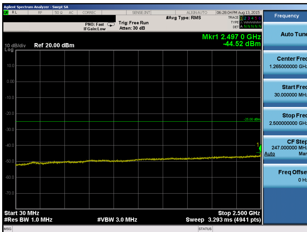
Plot 6-84. Conducted Spurious Plot (Band 7 – 20.0MHz QPSK – RB Size 1, RB Offset 0 – Mid Channel)
