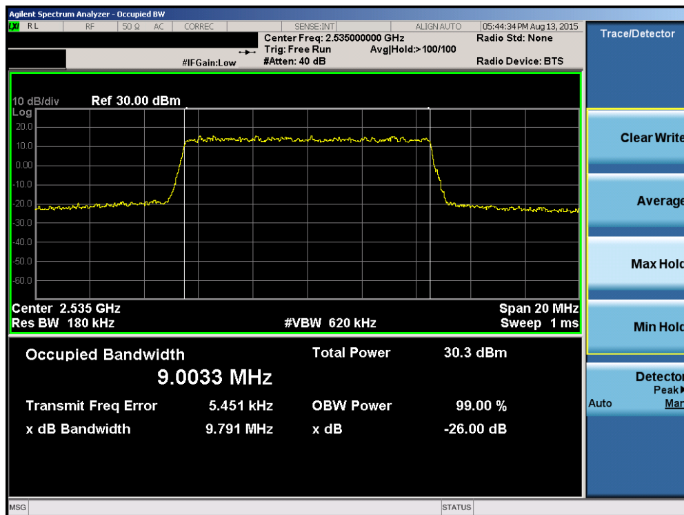
Plot 6-40. Occupied Bandwidth Plot (Band 7 – 10.0MHz 16-QAM – RB Size 50)
