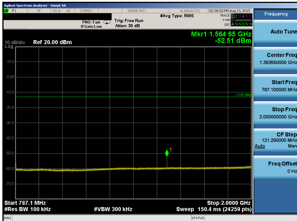
Plot 6-52. Conducted Spurious Plot (Band 13 – 5.0MHz QPSK – RB Size 1, RB Offset 0 – High Channel)
