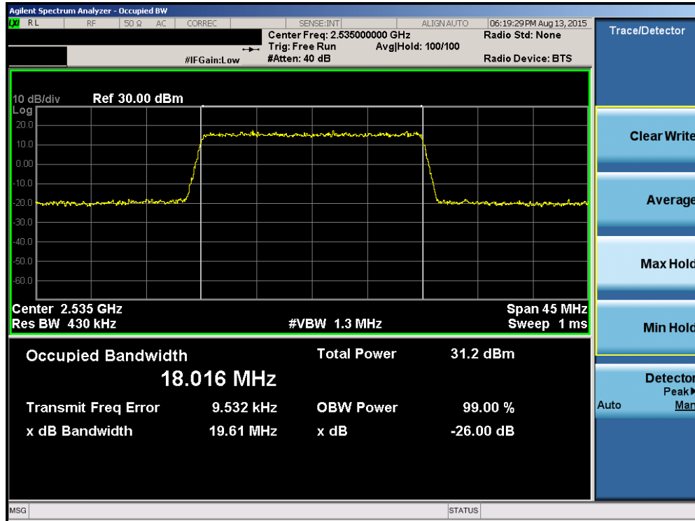
Plot 6-43. Occupied Bandwidth Plot (Band 7 – 20.0MHz QPSK – RB Size 100)
