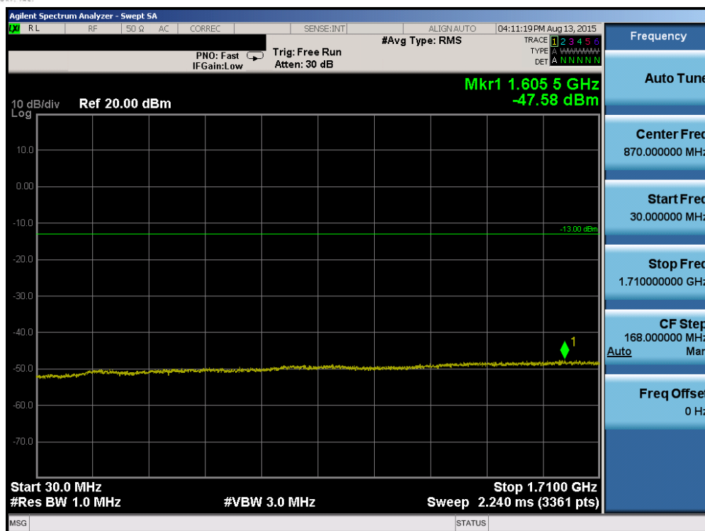
Plot 6-69. Conducted Spurious Plot (Band 4 – 1.4MHz QPSK – RB Size 1, RB Offset 0 – High Channel)
