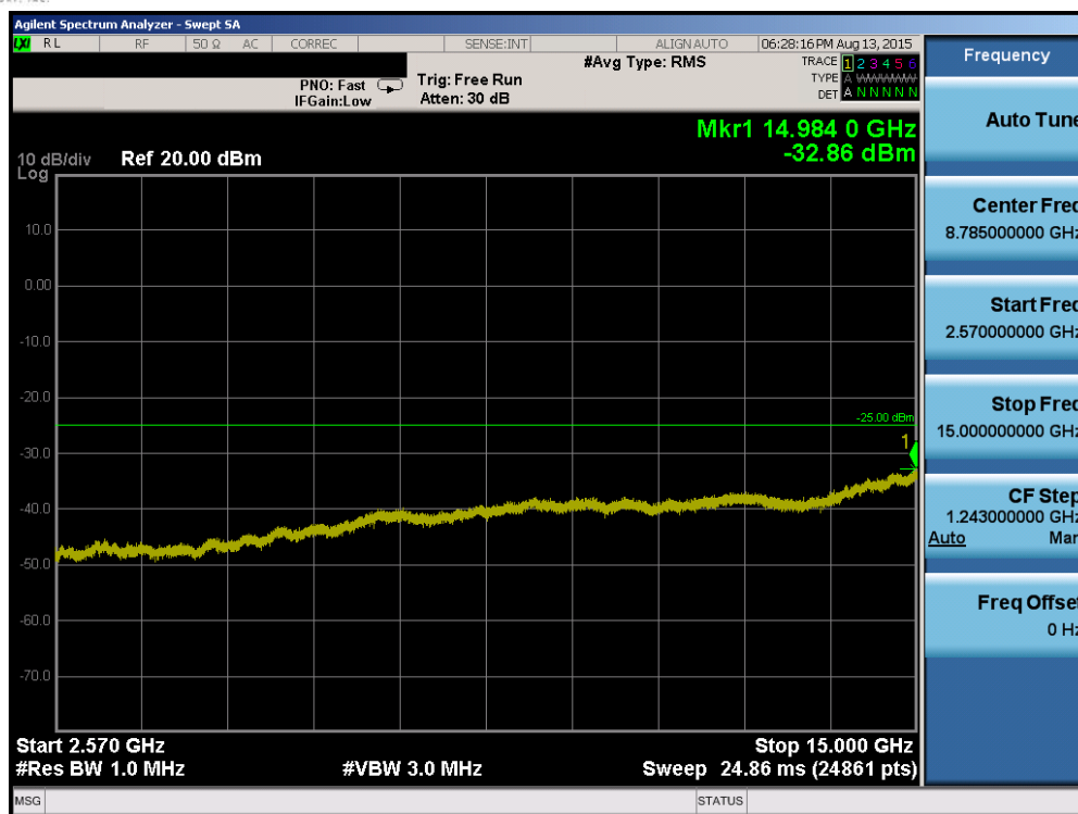
Plot 6-85. Conducted Spurious Plot (Band 7 – 20.0MHz QPSK – RB Size 1, RB Offset 0 – Mid Channel)
