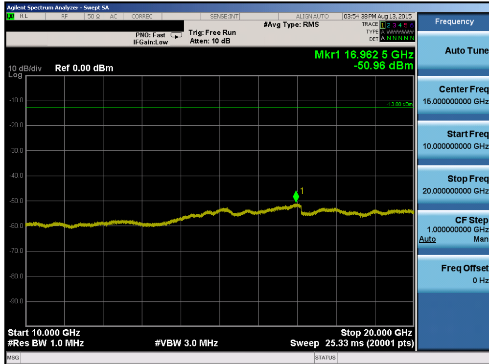
Plot 6-65. Conducted Spurious Plot (Band 4 – 1.4MHz QPSK – RB Size 1, RB Offset 0 – Low Channel)
