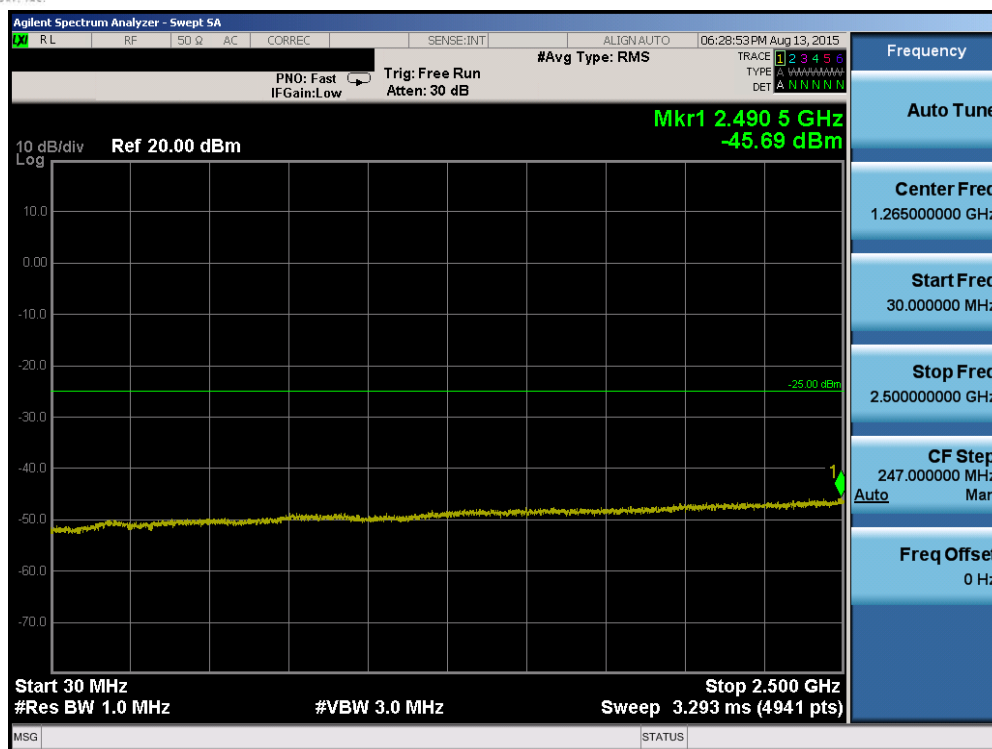
Plot 6-87. Conducted Spurious Plot (Band 7 – 20.0MHz QPSK – RB Size 1, RB Offset 0 – High Channel)
