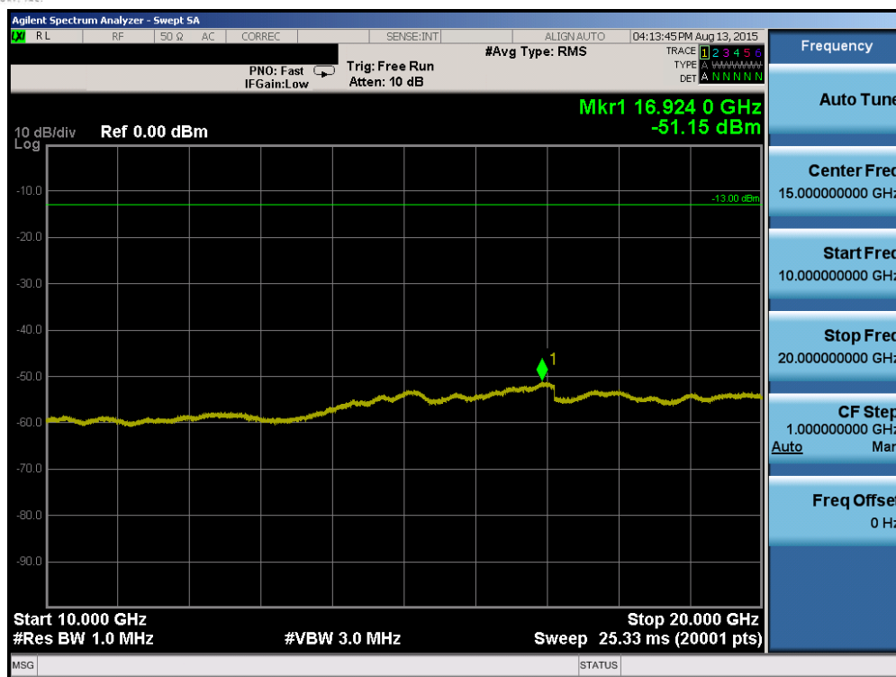
Plot 6-71. Conducted Spurious Plot (Band 4 – 1.4MHz QPSK – RB Size 1, RB Offset 0 – High Channel)
