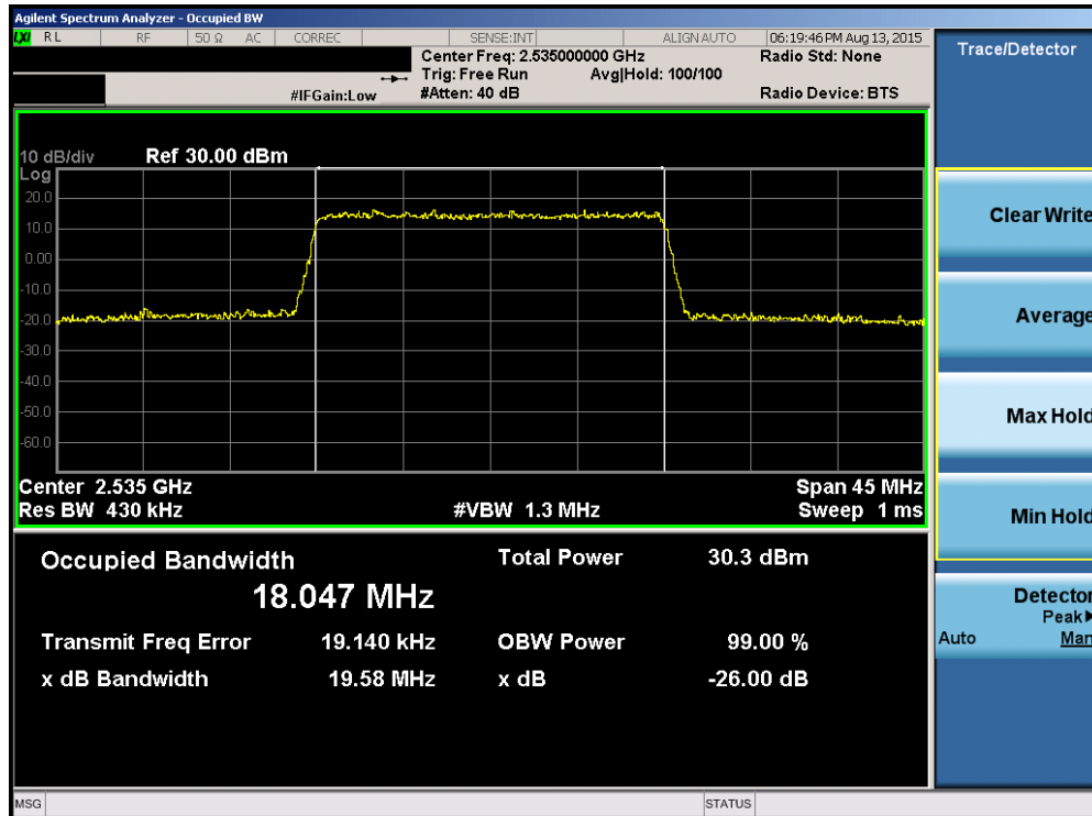
Plot 6-44. Occupied Bandwidth Plot (Band 7 – 20.0MHz 16-QAM – RB Size 100)
