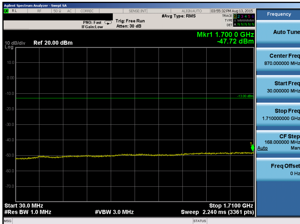
Plot 6-66. Conducted Spurious Plot (Band 4 – 1.4MHz QPSK – RB Size 1, RB Offset 0 – Mid Channel)
