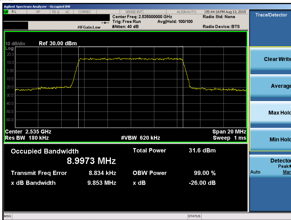
Plot 6-39. Occupied Bandwidth Plot (Band 7 – 10.0MHz QPSK – RB Size 50)
