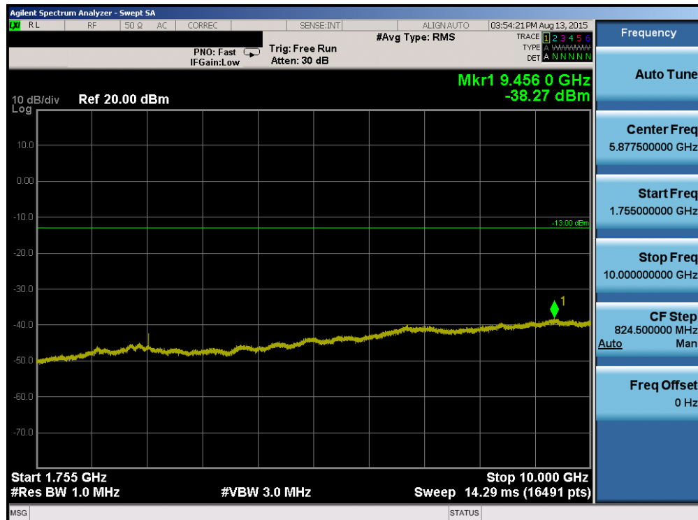
Plot 6-64. Conducted Spurious Plot (Band 4 – 1.4MHz QPSK – RB Size 1, RB Offset 0 – Low Channel)
