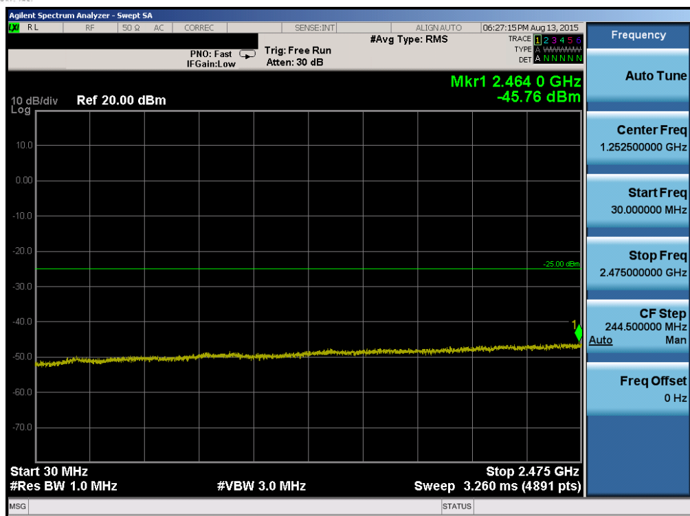
Plot 6-81. Conducted Spurious Plot (Band 7 – 20.0MHz QPSK – RB Size 1, RB Offset 0– Low Channel)
