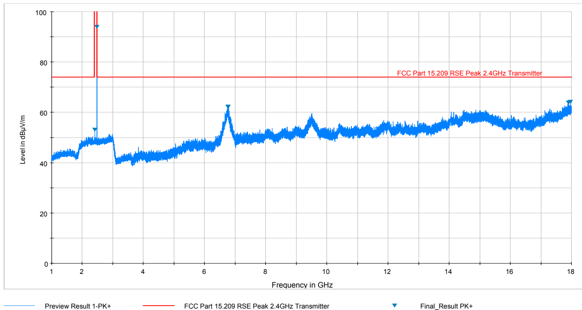
Plot 7-22. Radiated Spurious Plot above 1GHz (BT LE – Ch. 39, Ant. Pol. H)
