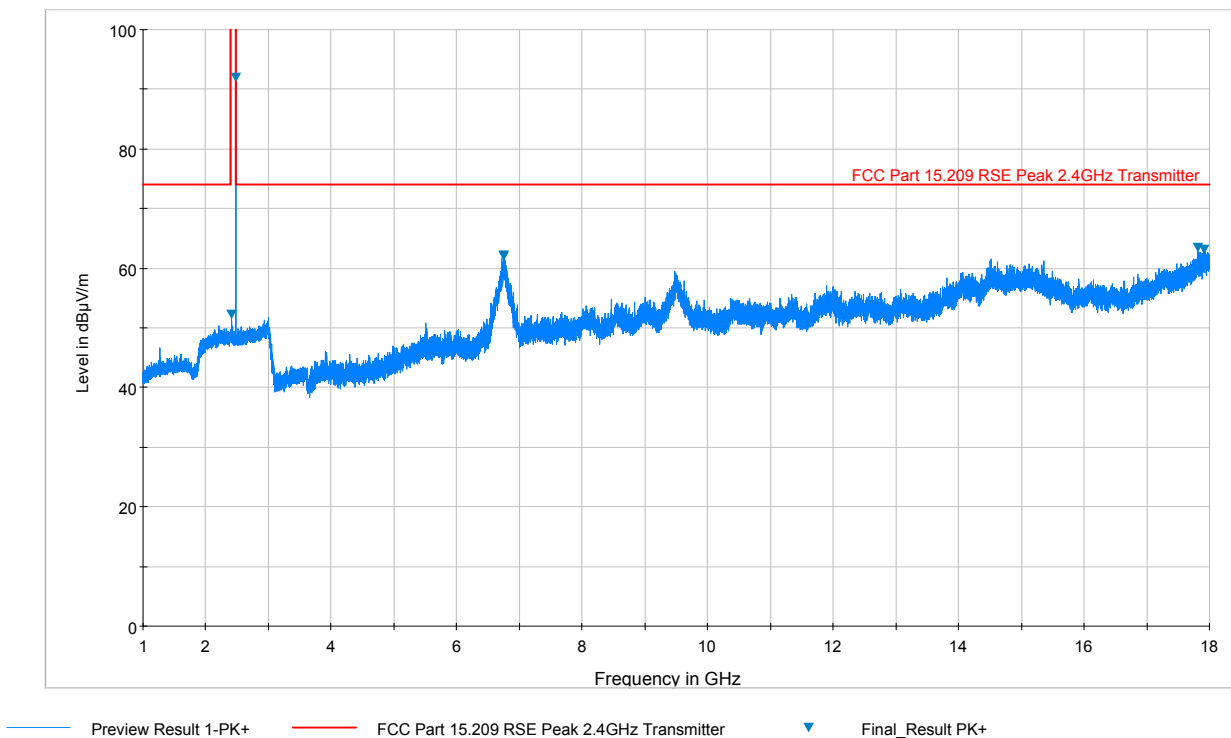
Plot 7-23. Radiated Spurious Plot above 1GHz (BT LE – Ch. 39, Ant. Pol. V)
