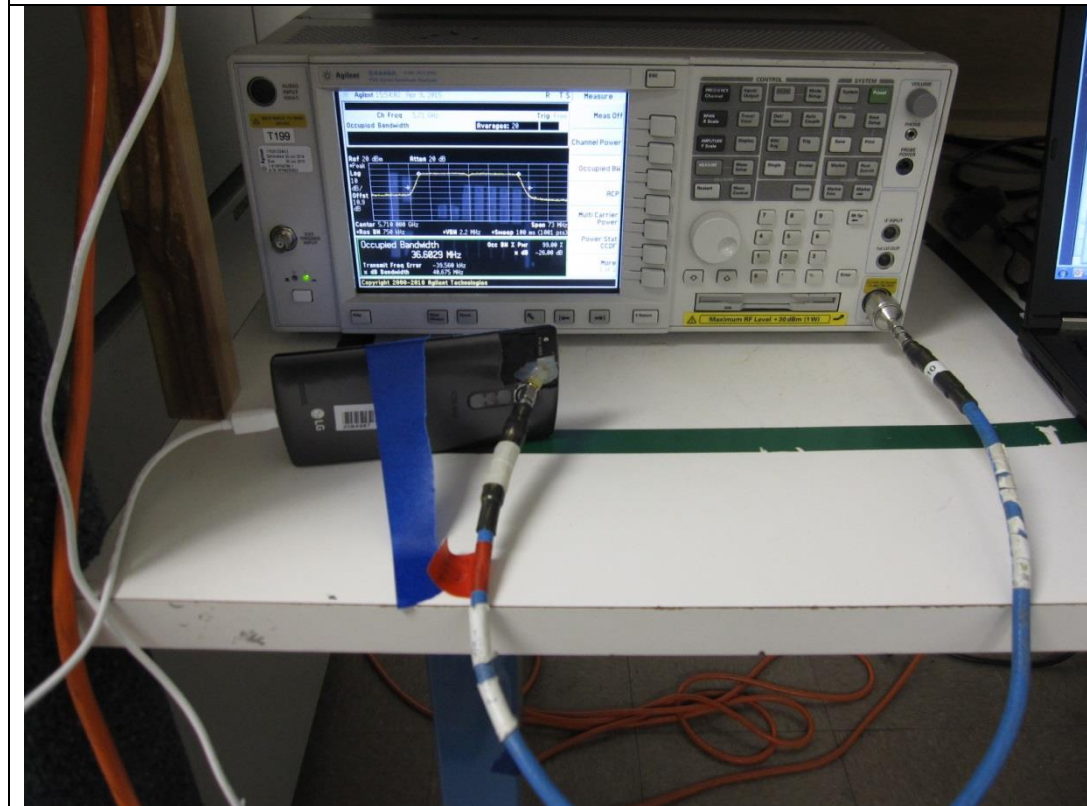
ANTENNA PORT CONDUCTED PHOTO
