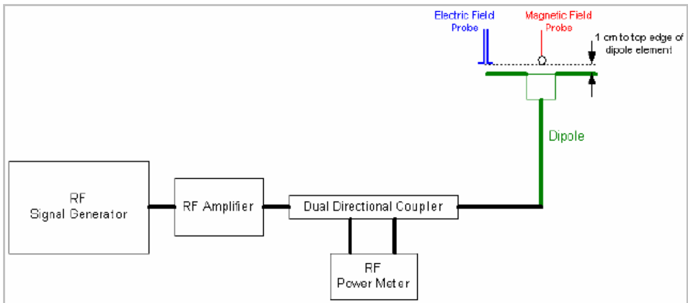
Setup diagram
