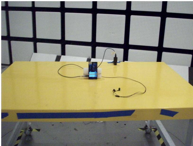
RADIATED EMISSION FRONT PHOTO
