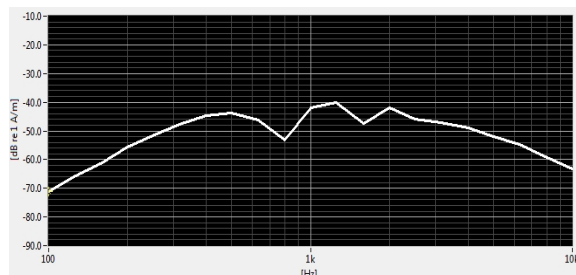
Figure 7-2 Worst-case ABM2 Plot for WD
