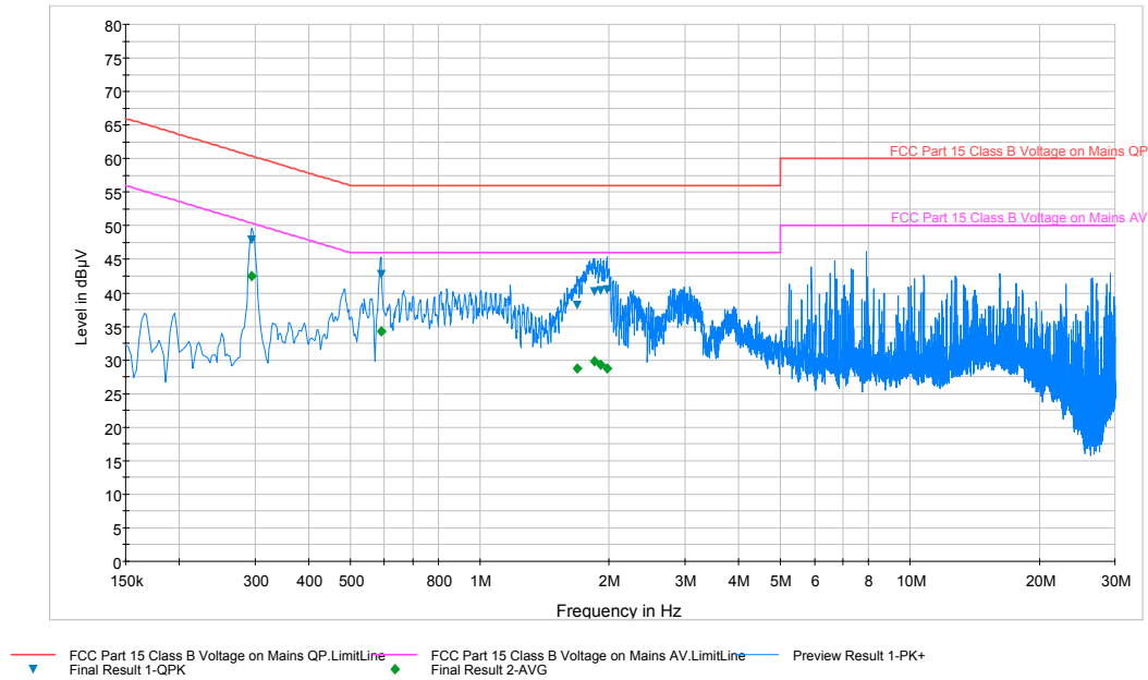
Plot 6-36. Line Conducted Plot with 802.11b (N)
