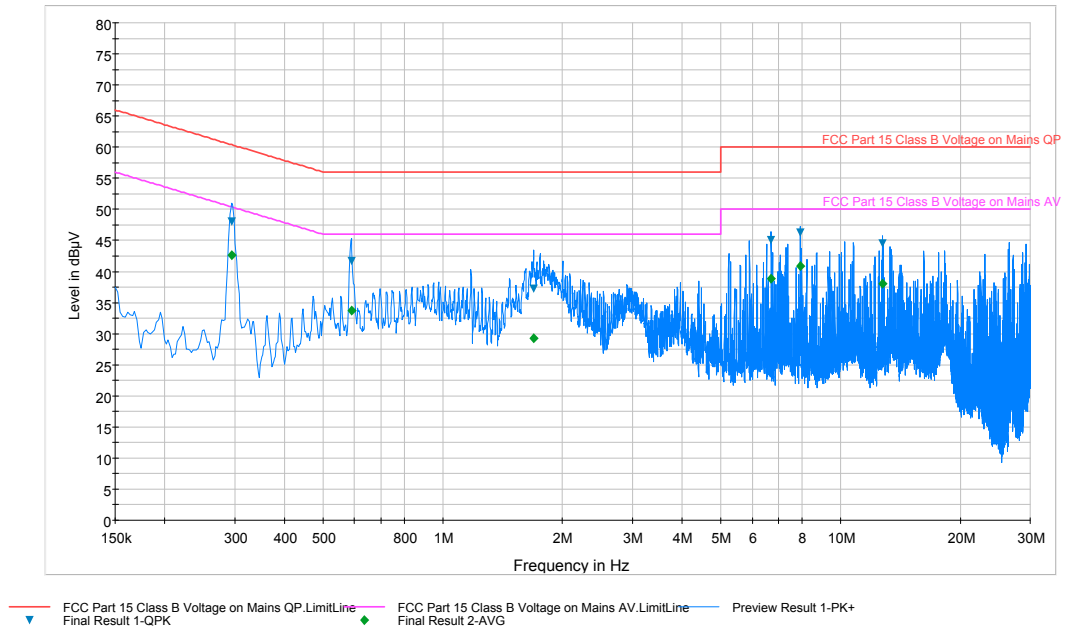
Plot 6-35. Line Conducted Plot with 802.11b (L1)
