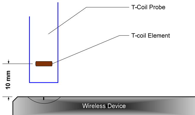
Figure 5-10 Measurement Distance
