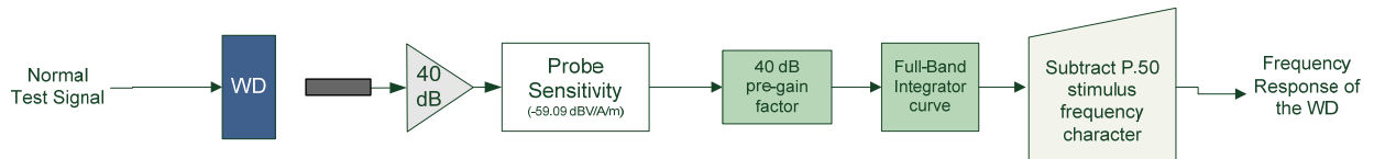
Figure 5-11 Frequency Response Block Diagram
