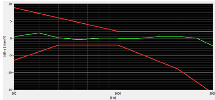
Figure 6-1 Axial Frequency Response
