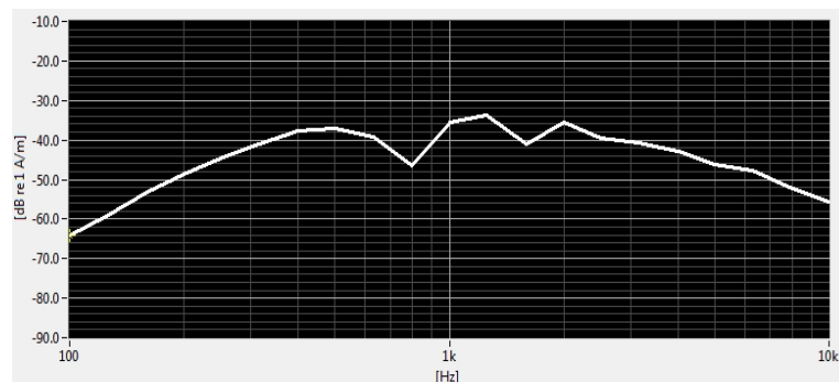
Figure 6-2 Worst-case ABM2 Plot for WD
