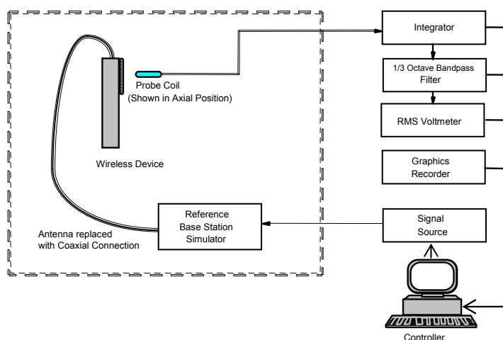
Figure 5-12 Audio Magnetic Field Test Setup
