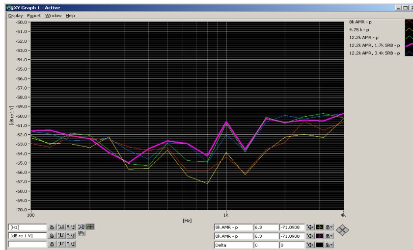
Figure 7-2 UMTS Audio Band Magnetic Noise
