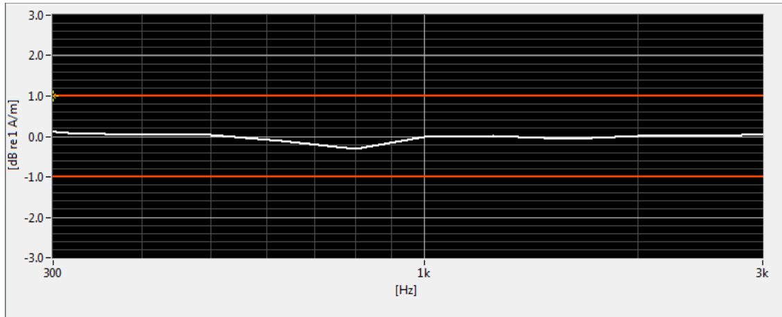
Figure 7-3 Helmholtz Coil Validation for Frequency Response
