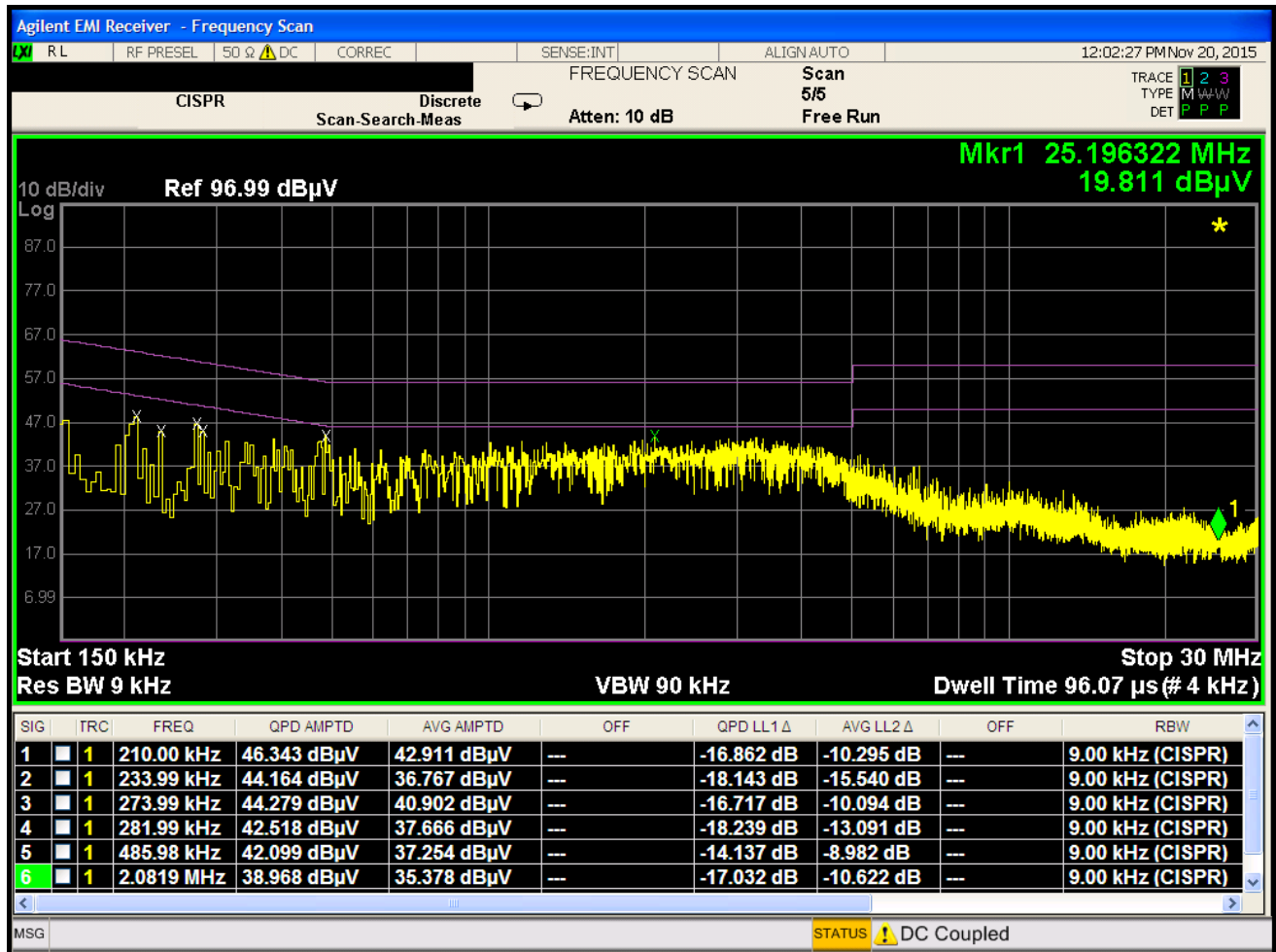
Plot 7-23. Line Conducted Plot with Bluetooth LE (N) Additional AC Adapter EAY64329102
