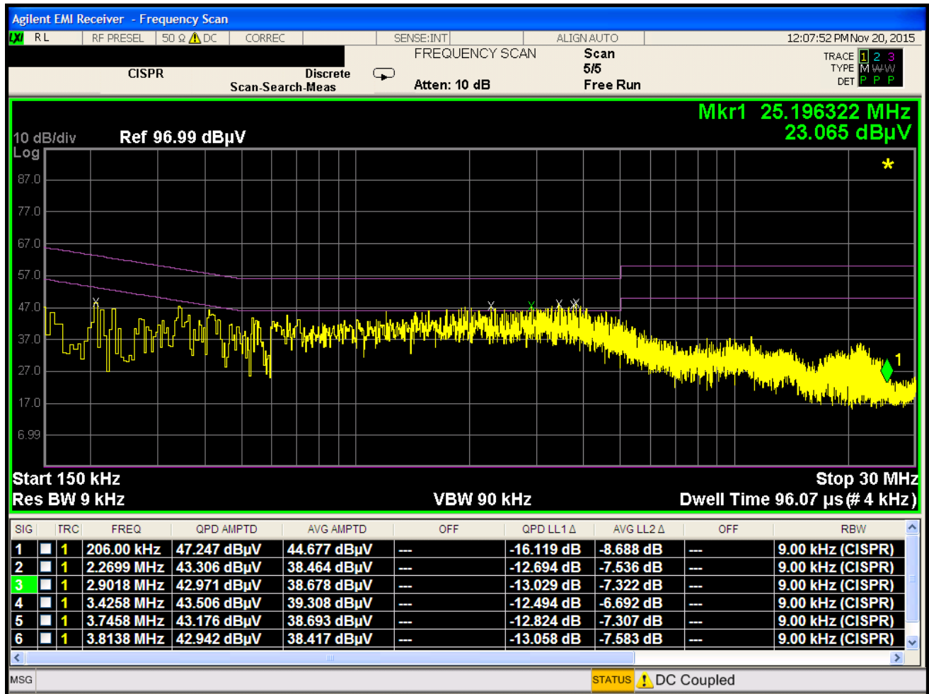
Plot 7-22. Line Conducted Plot with Bluetooth LE (L1) Additional AC Adapter EAY64329102
