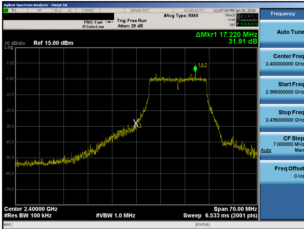
Plot 7-23. Band Edge Plot (802.11g– Ch. 1)
