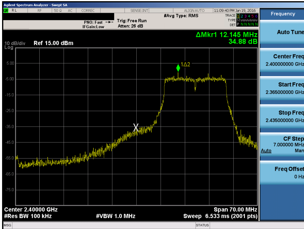
Plot 7-28. Band Edge Plot (802.11n (2.4GHz) – Ch. 2)
