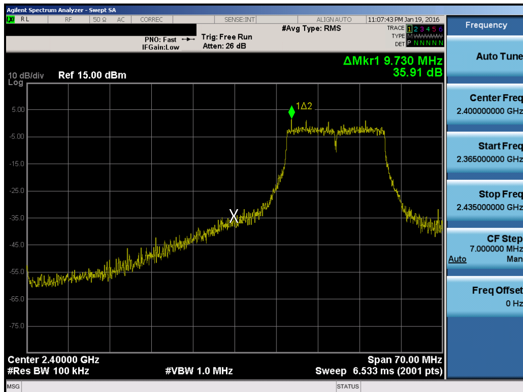
Plot 7-24. Band Edge Plot (802.11g – Ch. 2)
