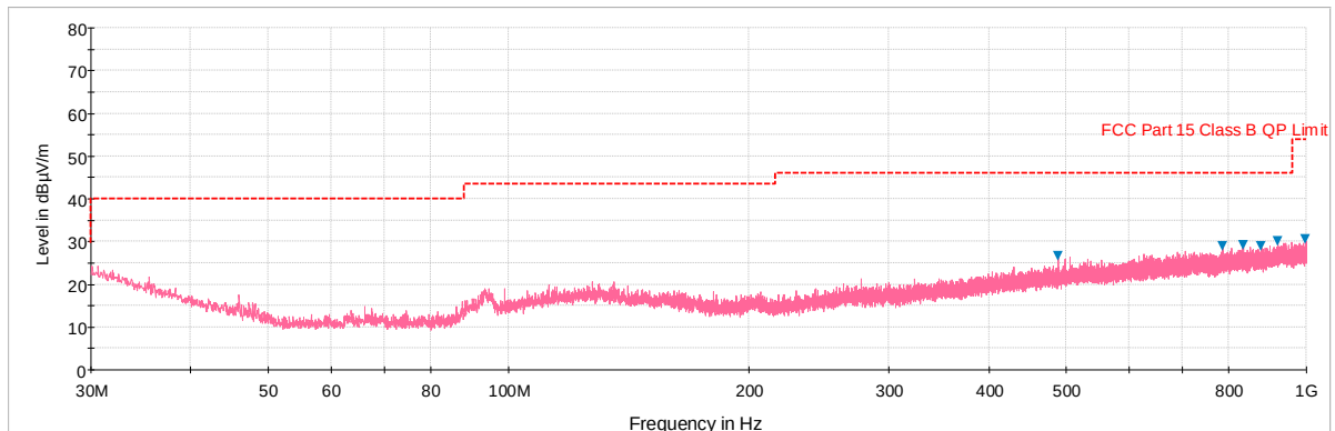
Plot 7-49. Radiated Spurious Plot below 1GHz (Pol. H)
