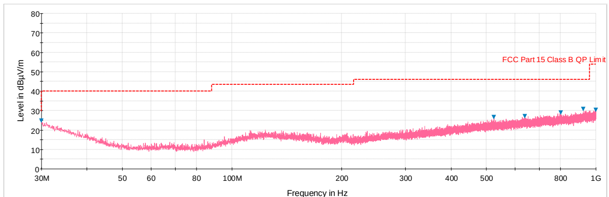
Plot 7-50. Radiated Spurious Plot below 1GHz (Pol. V)
