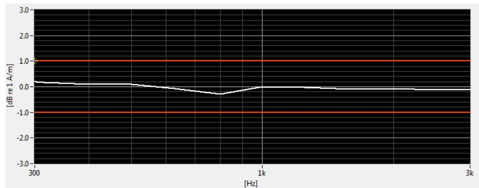
Figure 6-3 Helmholtz Coil Validation for Frequency Response
