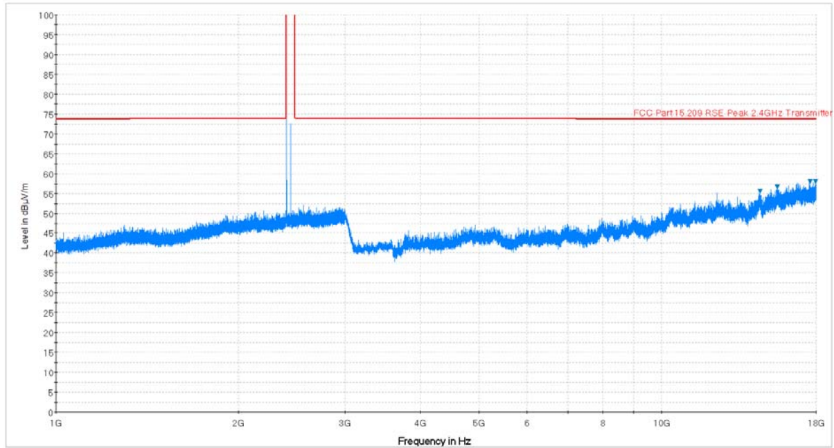
Plot 6-42. Radiated Spurious Plot above 1GHz (BT – Ch. 0, Ant. Pol. H)
