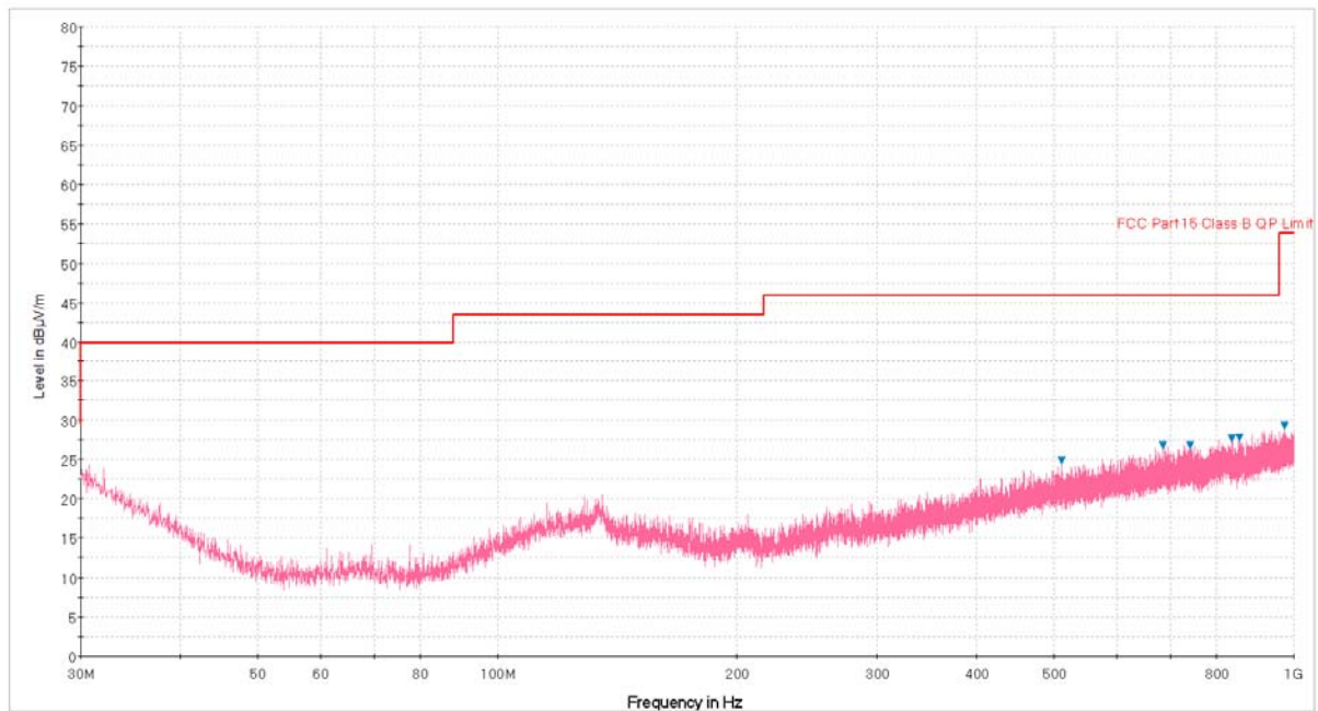
Plot 6-53. Radiated Spurious Plot below 1GHz (Pol. V)
