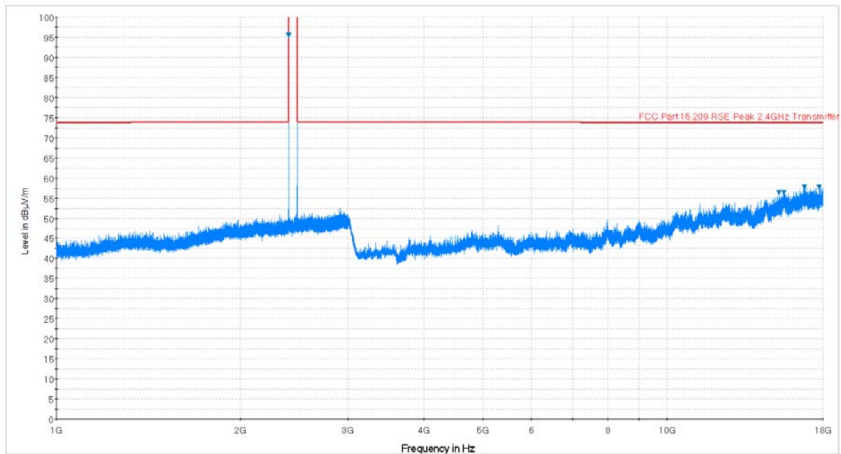
Plot 6-43. Radiated Spurious Plot above 1GHz (BT – Ch. 0, Ant. Pol. V)
