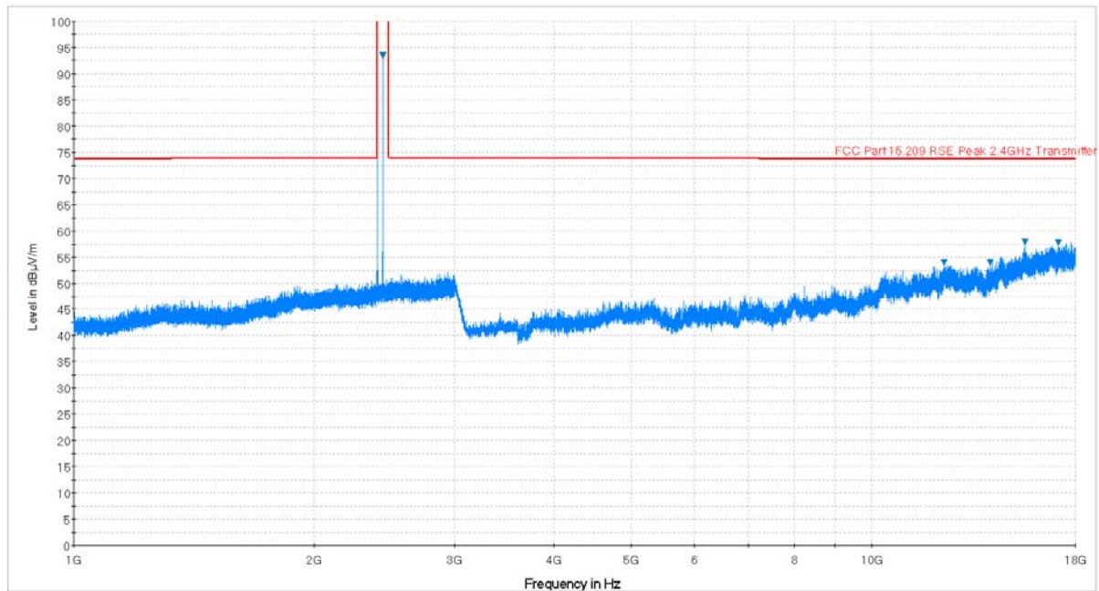
Plot 6-45. Radiated Spurious Plot above 1GHz (BT – Ch. 39, Ant. Pol. V)
