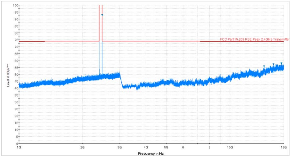
Plot 6-47. Radiated Spurious Plot above 1GHz (BT – Ch. 78, Ant. Pol. V)
