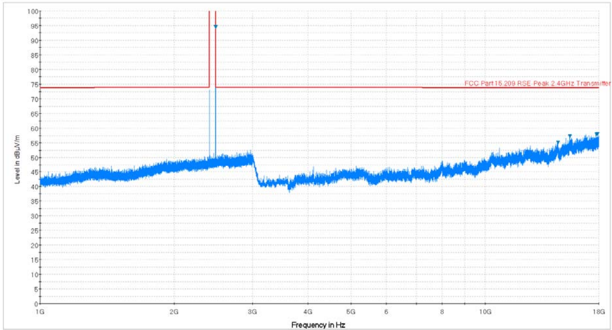
Plot 6-46. Radiated Spurious Plot above 1GHz (BT – Ch. 78, Ant. Pol. H)
