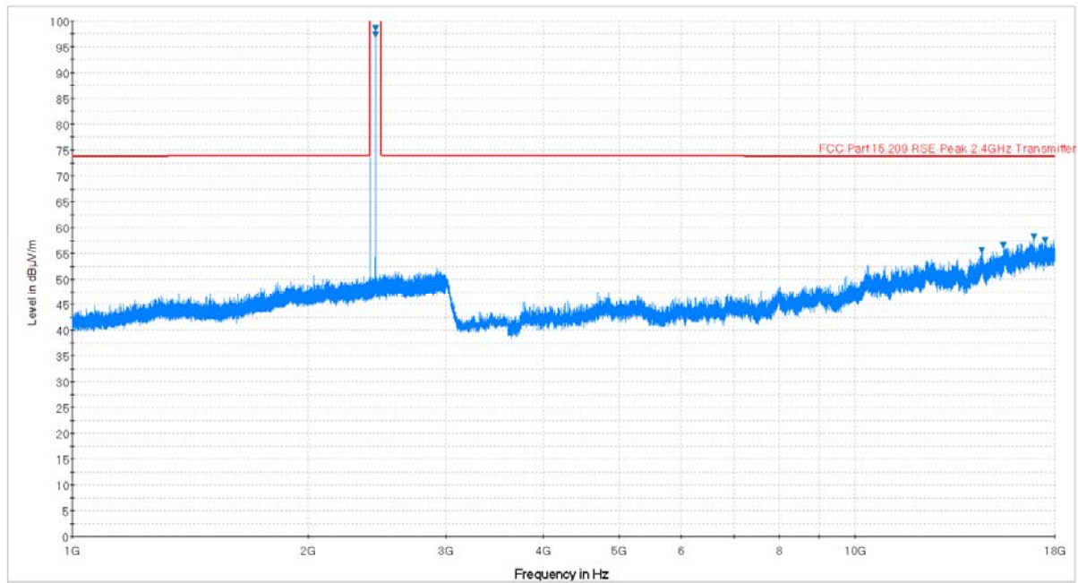
Plot 6-44. Radiated Spurious Plot above 1GHz (BT – Ch. 39, Ant. Pol. H)
