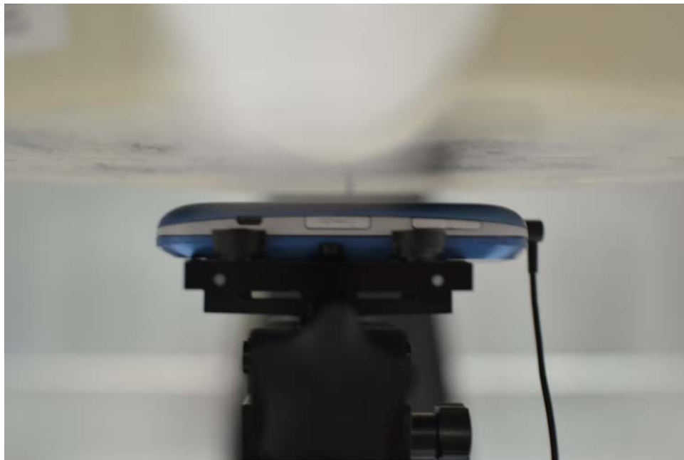
SAR Test Setup Photo 6: Back side at 1.5 cm with headphones
