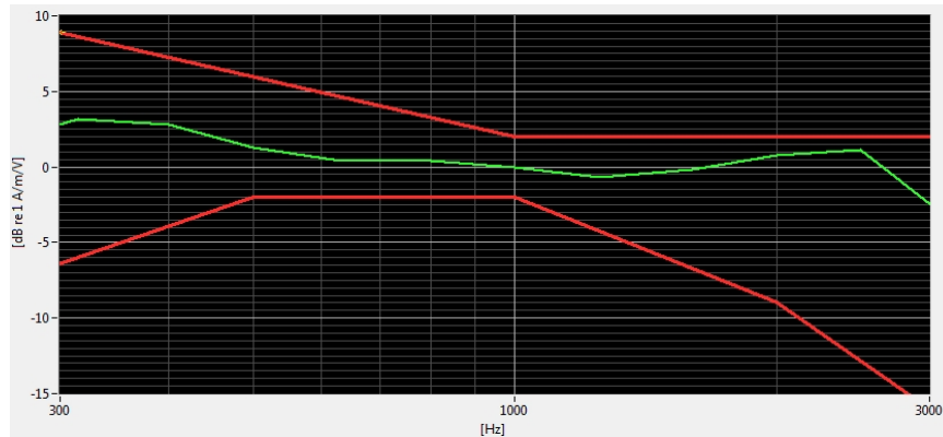
Figure 7-1 Axial Frequency Response
