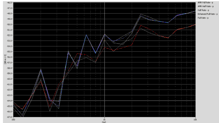
Figure 5-11 Vocoder Analysis for ABM Noise
