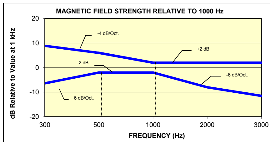
Figure 4-1 Magnetic field frequency response for Wireless Devices with an axial field \leq -15 dB (A/m) at 1 kHz
