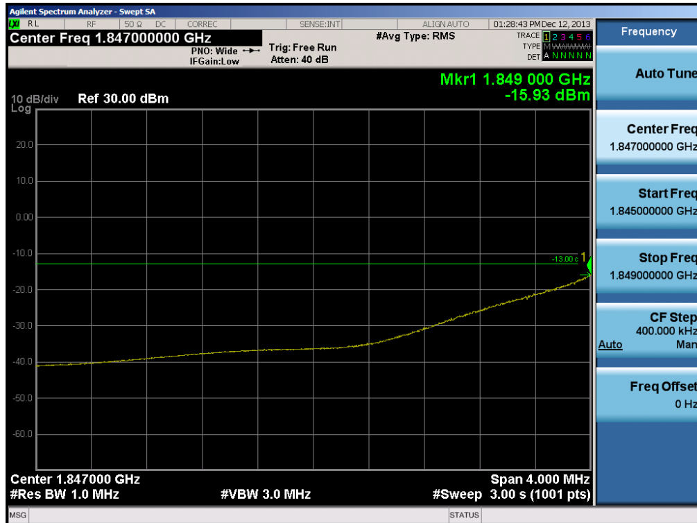
Plot 6-18. 4MHz Span Plot (PCS CDMA Mode – Ch. 25)
