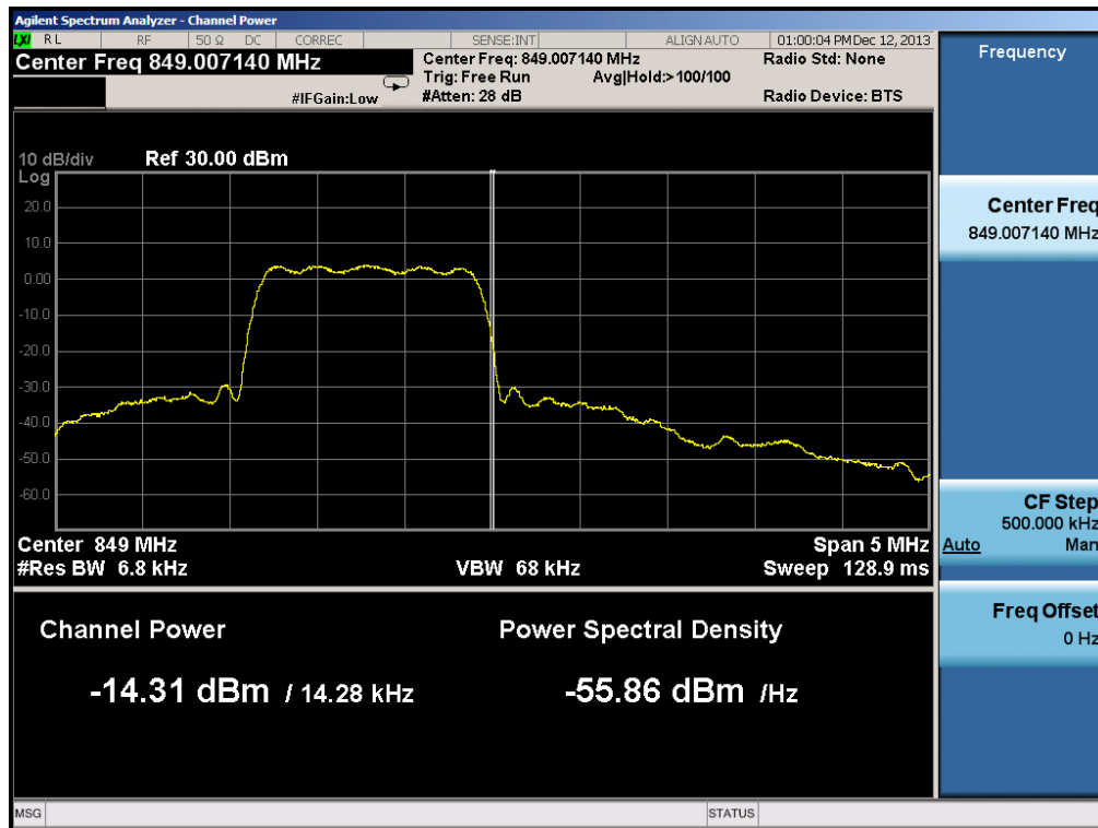
Plot 6-16. Band Edge Plot (Cellular CDMA Mode – Ch. 777)
