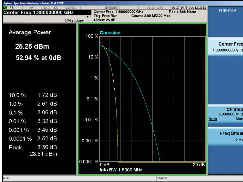
Plot 6-21. Peak-Average Ratio Plot (PCS CDMA Mode – Ch. 600)
