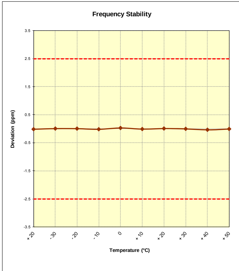
Figure 6-7. Frequency Stability Graph (Cellular CDMA Mode – Ch. 384)
