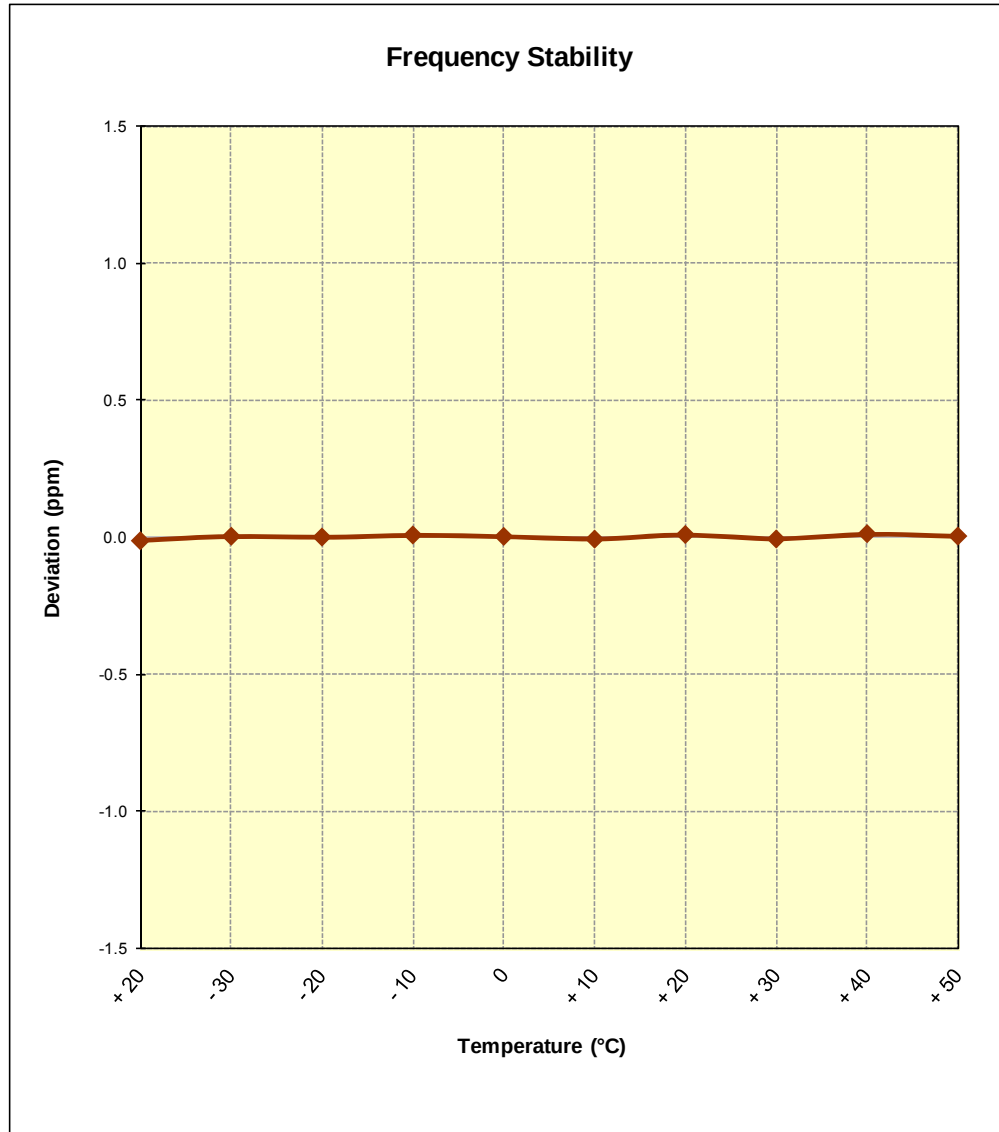
Figure 6-8. Frequency Stability Graph (PCS CDMA Mode – Ch. 600)
