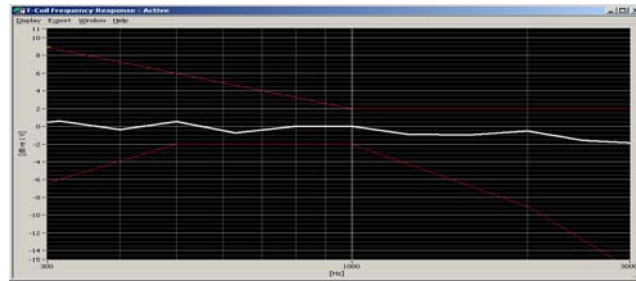
Figure 6-1 Axial Frequency Response
