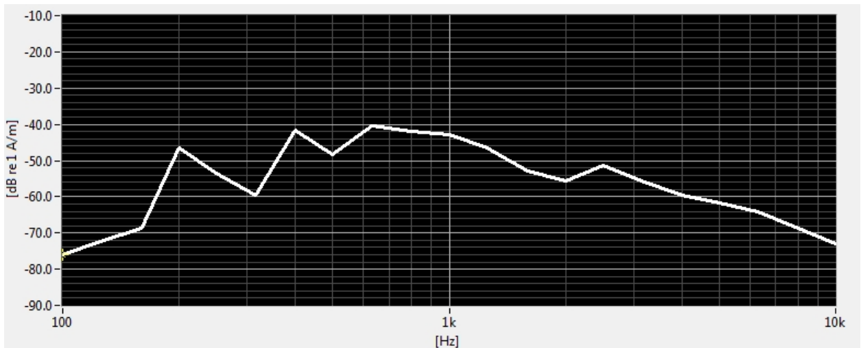
Figure 6-3 Worst-case ABM2 Plot for GSM
