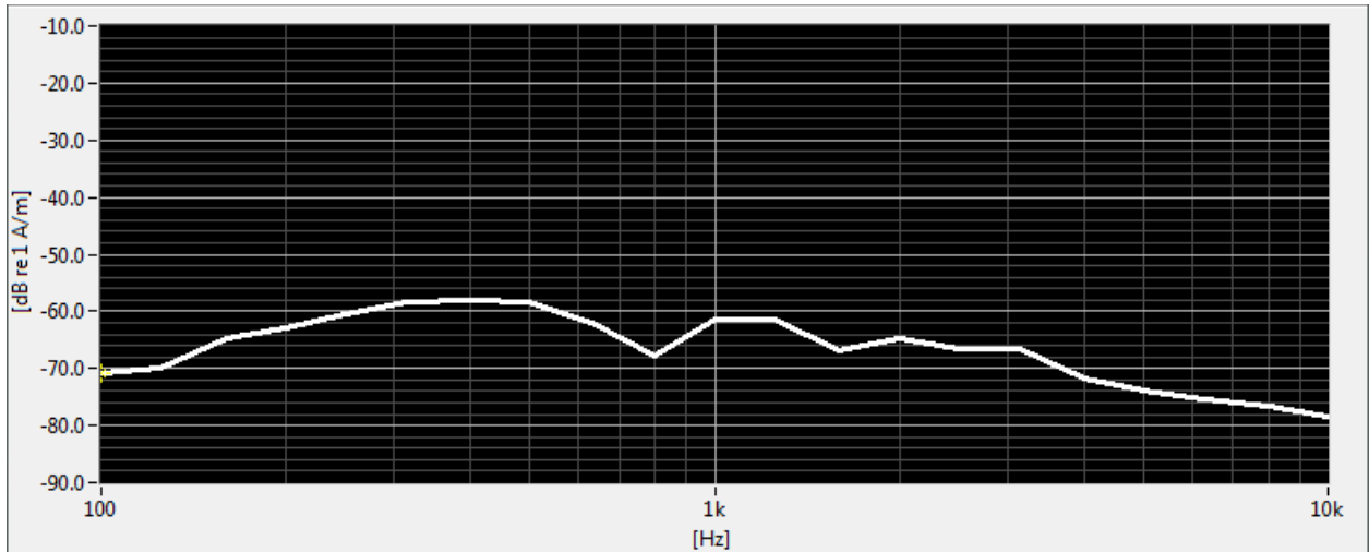
Figure 6-2 Worst-case ABM2 Plot for CDMA
