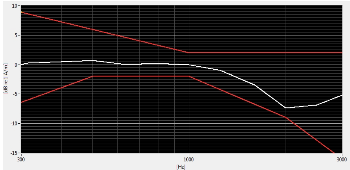
Figure 6-1 Axial Frequency Response
