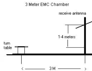
Figure 6-1. Test Instrument & Measurement Setup
