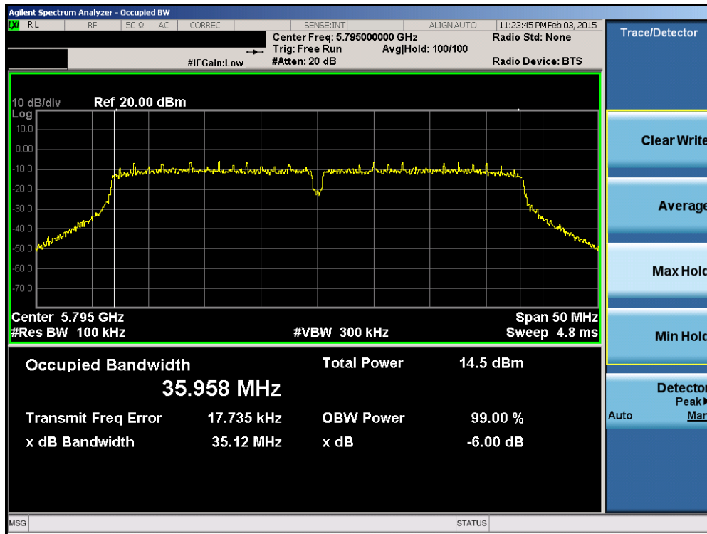
Plot 6-32. 6dB Bandwidth Plot (40MHz BW 802.11n (UNII Band 3) – Ch. 159)
