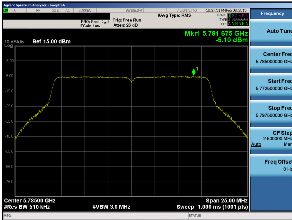
Plot 6-58. Power Spectral Density Plot (802.11a (UNII Band 3) – Ch. 157)
