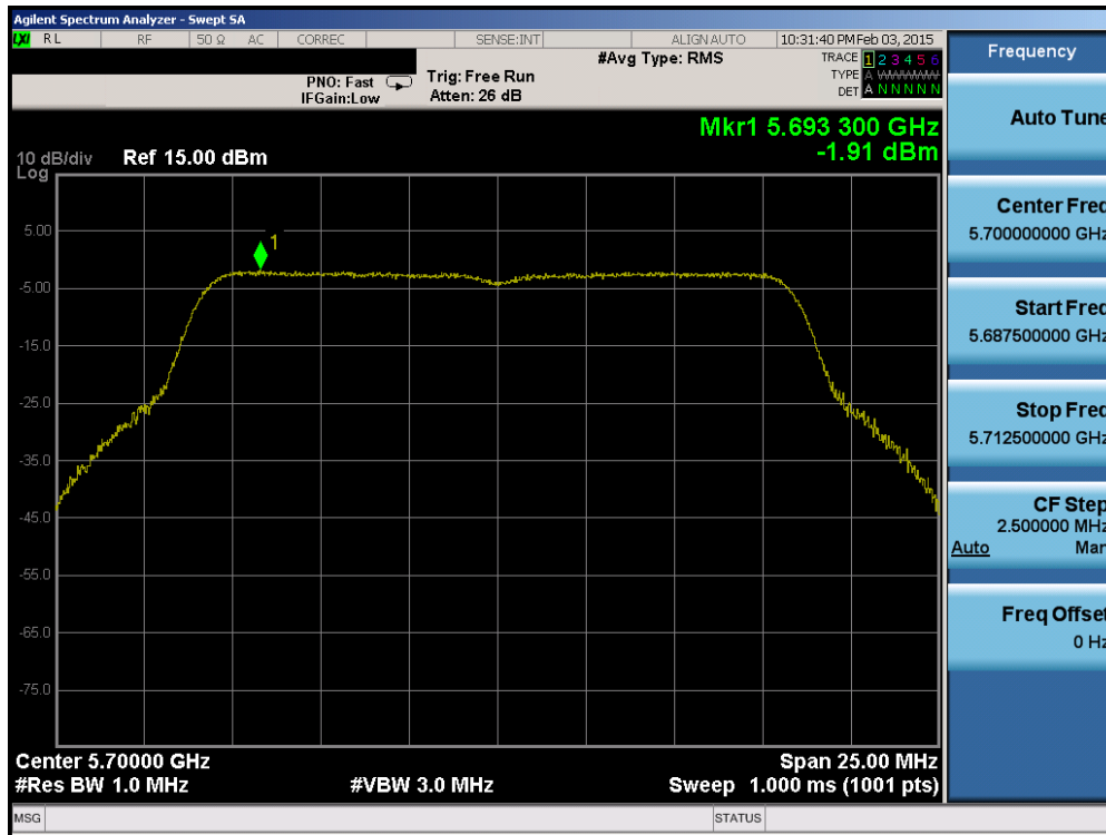
Plot 6-51. Power Spectral Density Plot (802.11a (UNII Band 2C) – Ch. 140)
