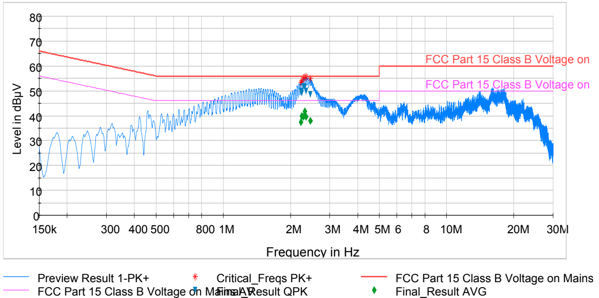
Plot 6-98. Line Conducted Plot with 802.11a UNII Band 2A (N)
