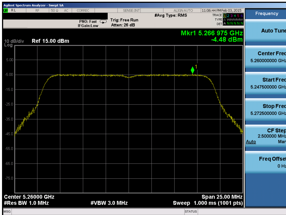
Plot 6-44. Power Spectral Density Plot (20MHz BW 802.11n (UNII Band 2A) – Ch. 52)
