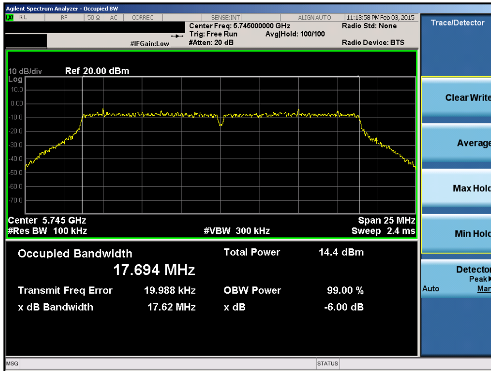
Plot 6-28. 6dB Bandwidth Plot (20MHz BW 802.11n (UNII Band 3) – Ch. 149)
