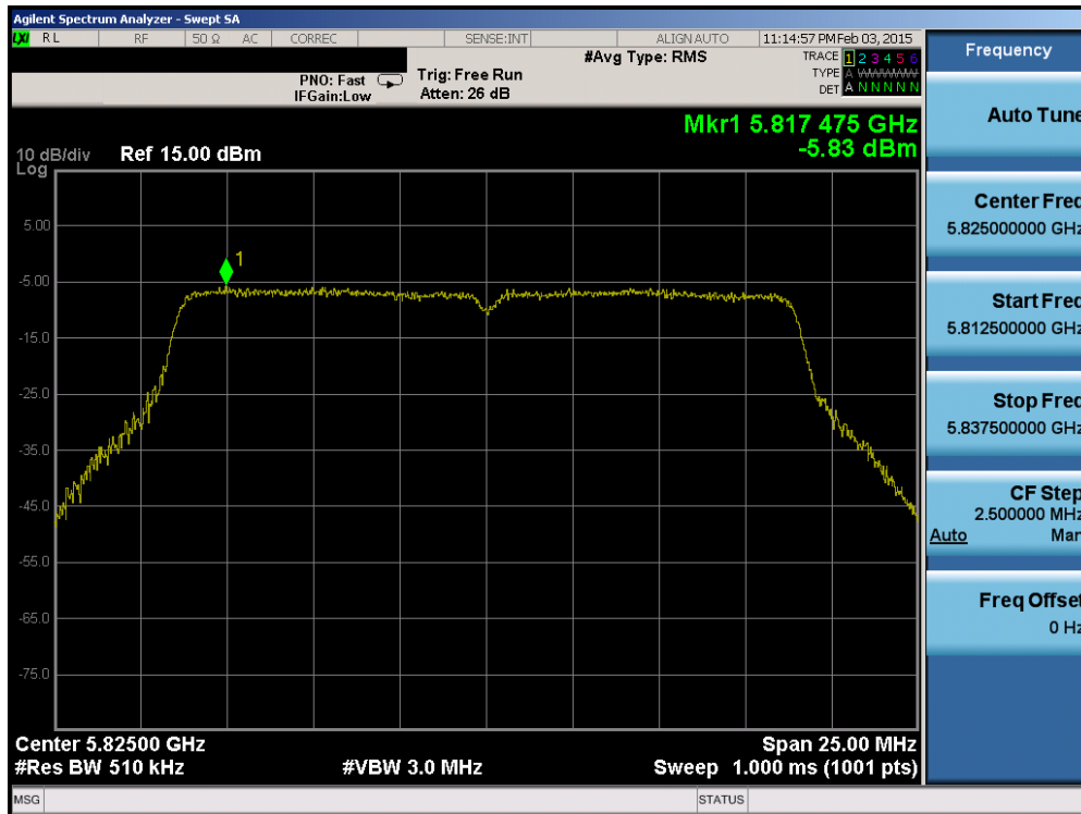
Plot 6-62. Power Spectral Density Plot (20MHz BW 802.11n (UNII Band 3) – Ch. 165)
