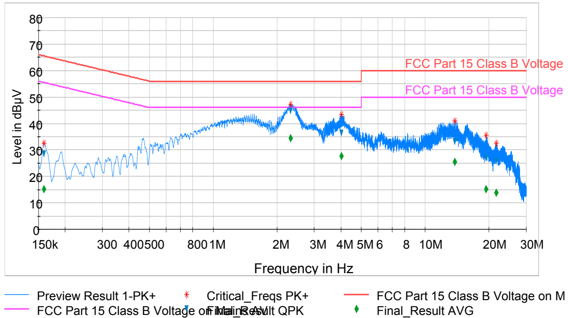
Plot 6-99. Line Conducted Plot with 802.11a UNII Band 2C (L1)
