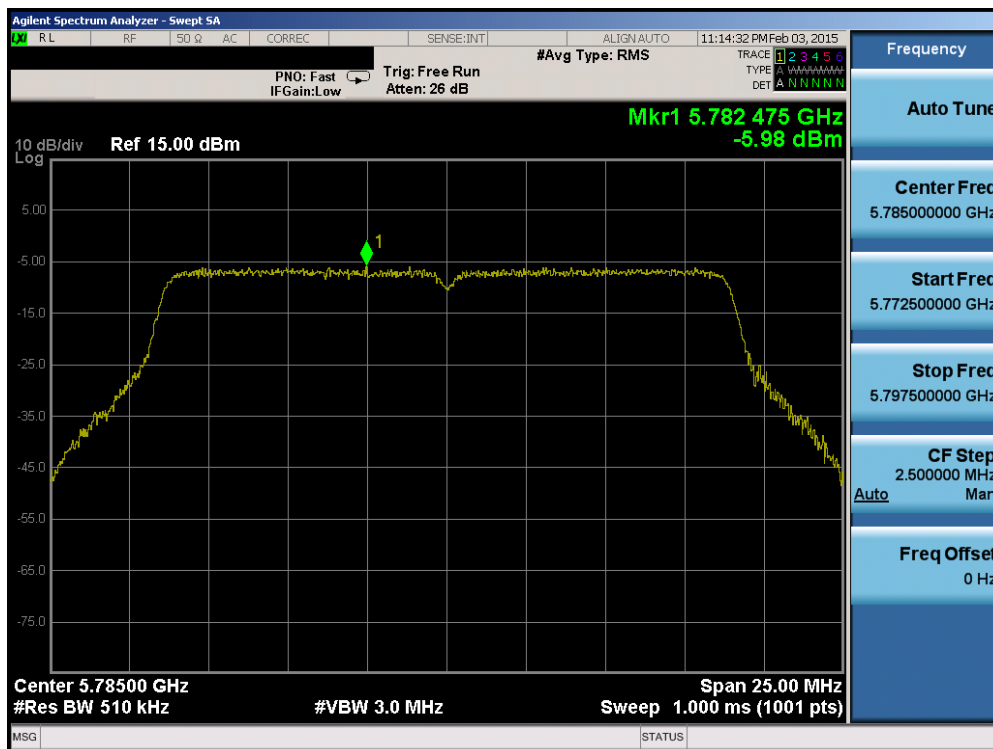
Plot 6-61. Power Spectral Density Plot (20MHz BW 802.11n (UNII Band 3) – Ch. 157)
