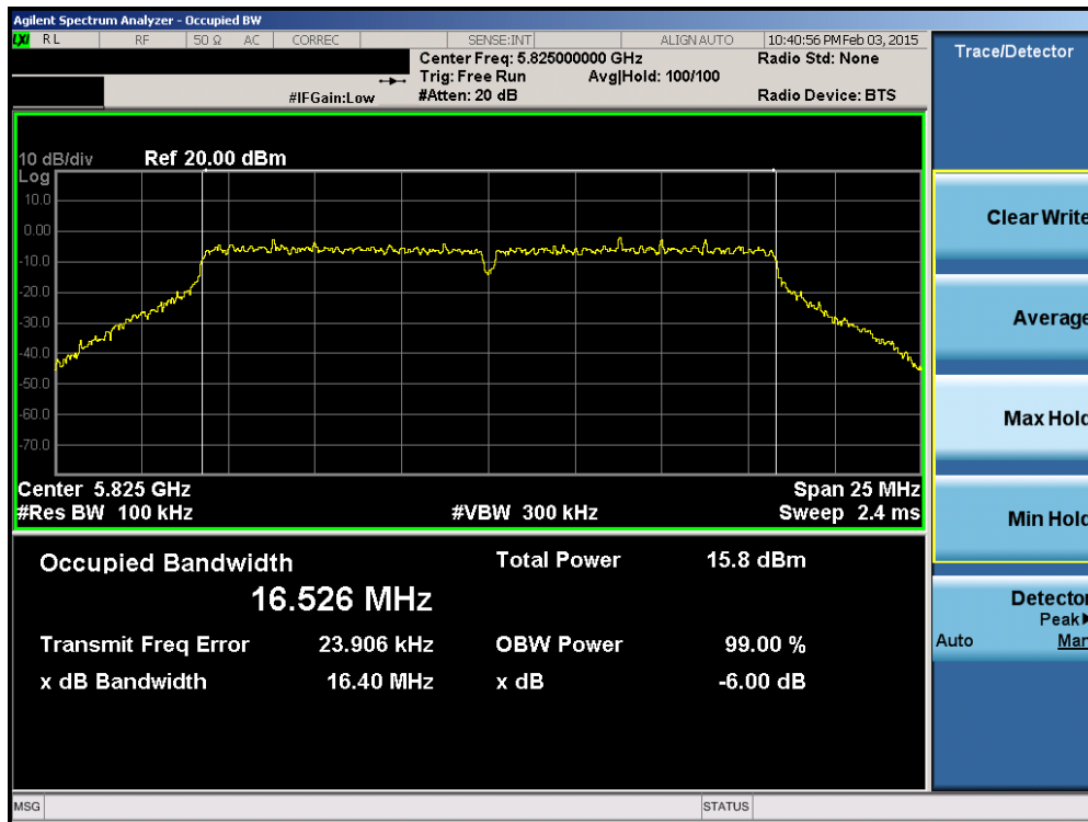
Plot 6-27. 6dB Bandwidth Plot (802.11a (UNII Band 3) – Ch. 165)
