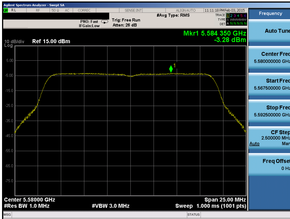
Plot 6-53. Power Spectral Density Plot (20MHz BW 802.11n (UNII Band 2C) – Ch. 116)
