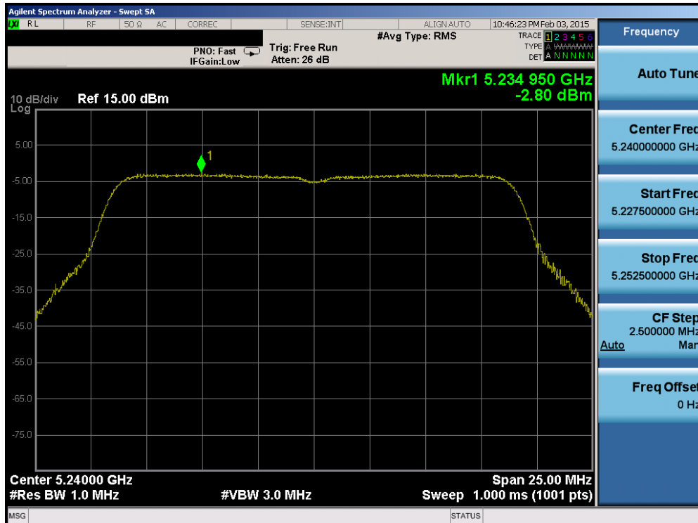
Plot 6-38. Power Spectral Density Plot (20MHz BW 802.11n (UNII Band 1) – Ch. 48)
