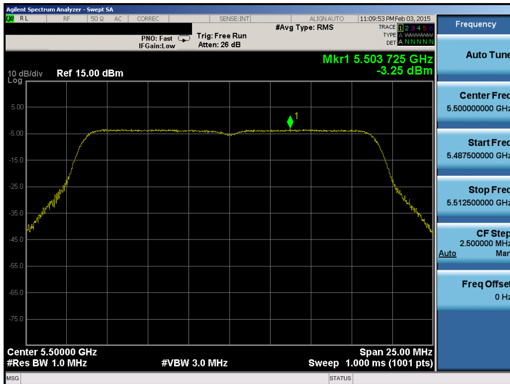
Plot 6-52. Power Spectral Density Plot (20MHz BW 802.11n (UNII Band 2C) – Ch. 100)
