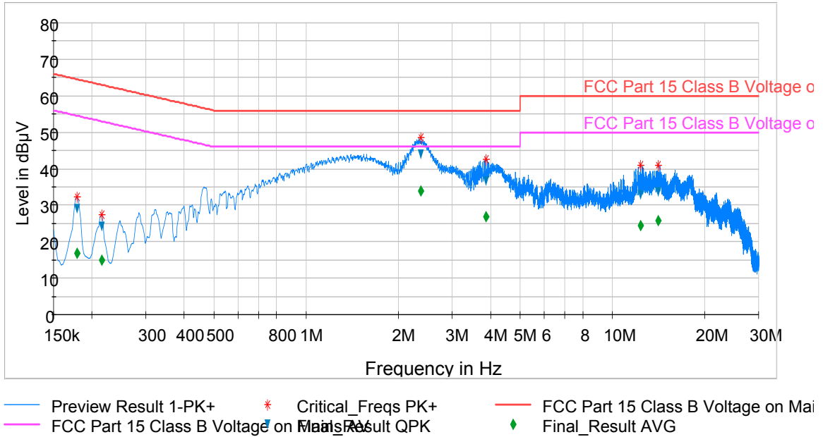
Plot 6-95. Line Conducted Plot with 802.11a UNII Band 1 (L1)
