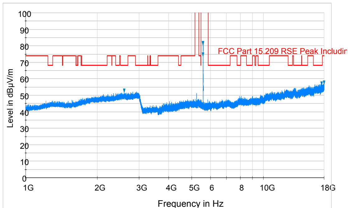
Plot 6-70. Radiated Spurious Plot above 1GHz (802.11a – U2C Ch. 116, Ant. Pol. V)
