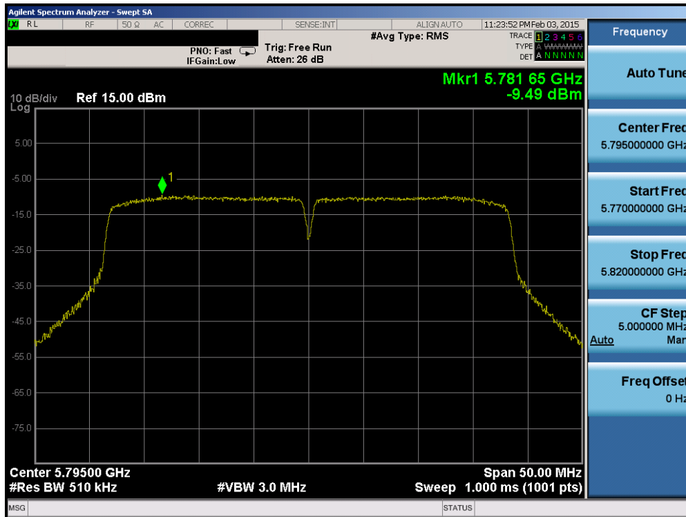
Plot 6-64. Power Spectral Density Plot (40MHz BW 802.11n (UNII Band 3) – Ch. 159)
