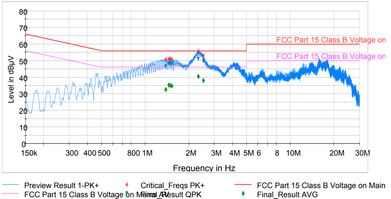
Plot 6-96. Line Conducted Plot with 802.11a UNII Band 1 (N)
