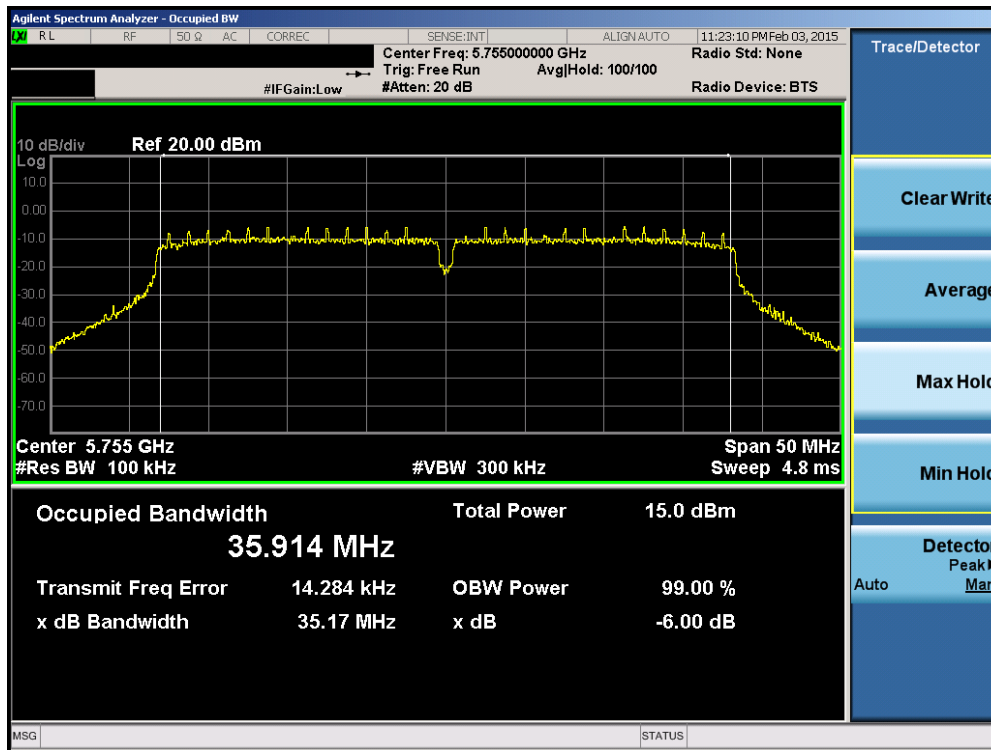
Plot 6-31. 6dB Bandwidth Plot (40MHz BW 802.11n (UNII Band 3) – Ch. 151)
