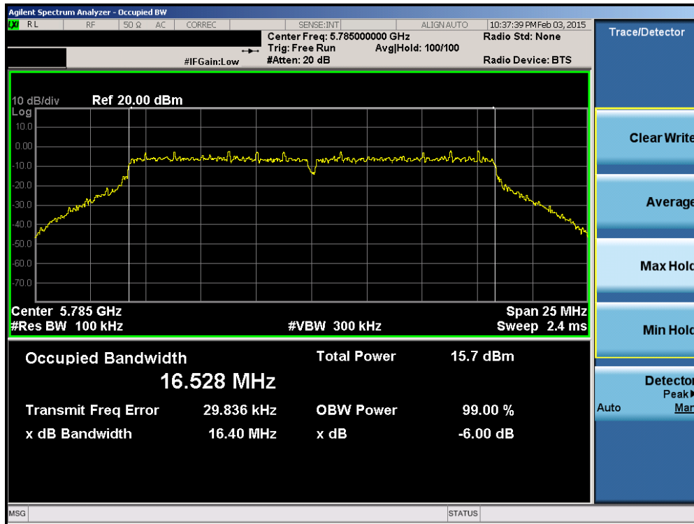
Plot 6-26. 6dB Bandwidth Plot (802.11a (UNII Band 3) – Ch. 157)
