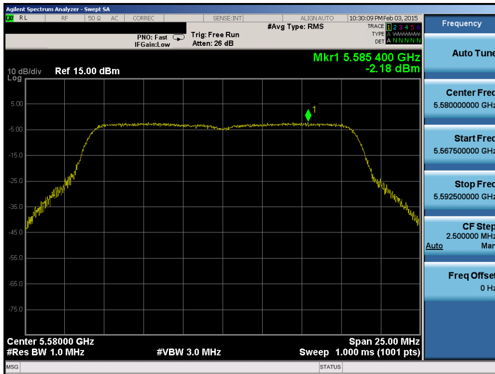
Plot 6-50. Power Spectral Density Plot (802.11a (UNII Band 2C) – Ch. 116)
