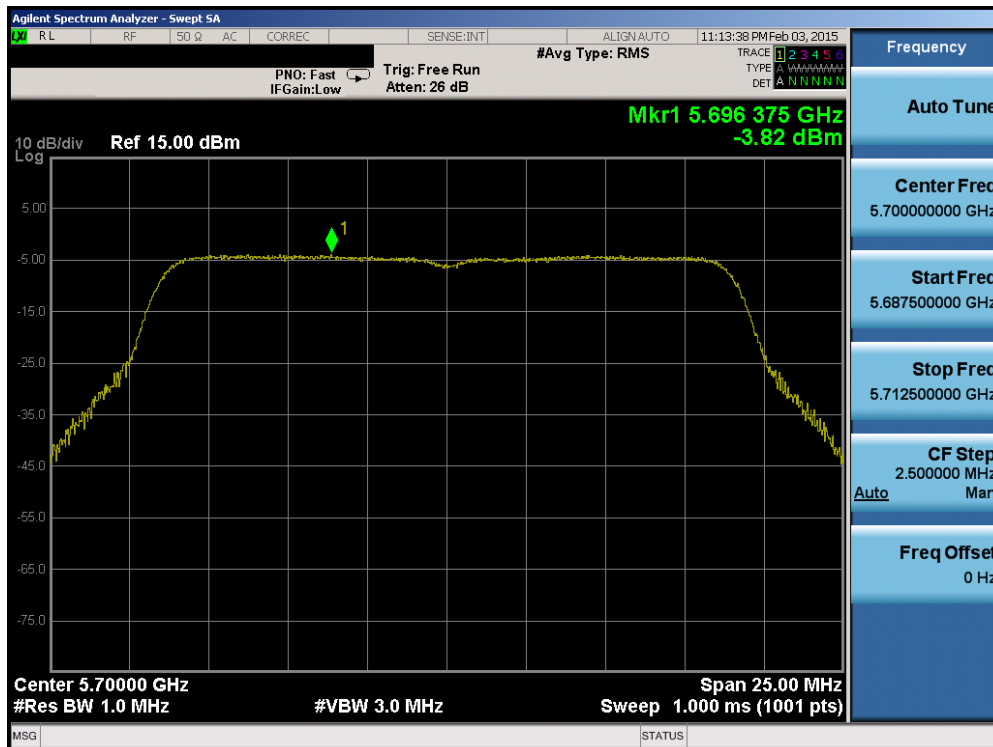
Plot 6-54. Power Spectral Density Plot (20MHz BW 802.11n (UNII Band 2C) – Ch. 140)
