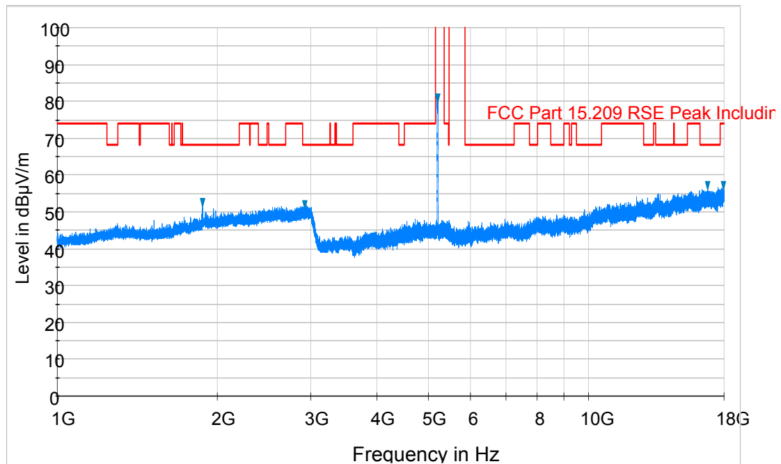
Plot 6-66. Radiated Spurious Plot above 1GHz (802.11a – U1 Ch. 40, Ant. Pol. V)
