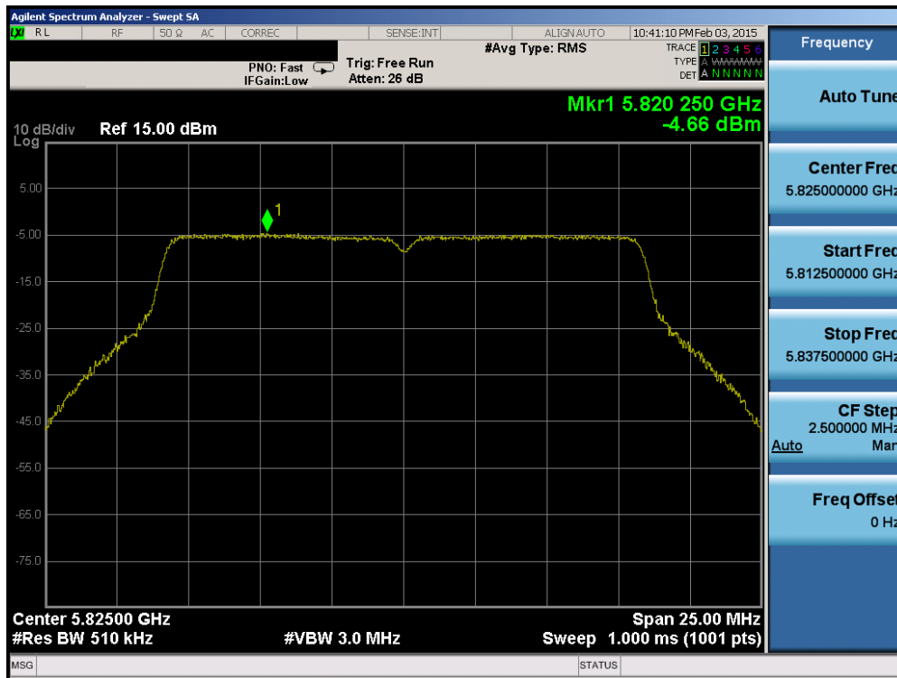
Plot 6-59. Power Spectral Density Plot (802.11a (UNII Band 3) – Ch. 165)
