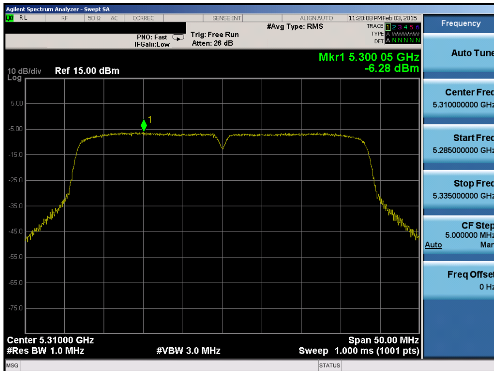
Plot 6-48. Power Spectral Density Plot (40MHz BW 802.11n (UNII Band 2A) – Ch. 62)
