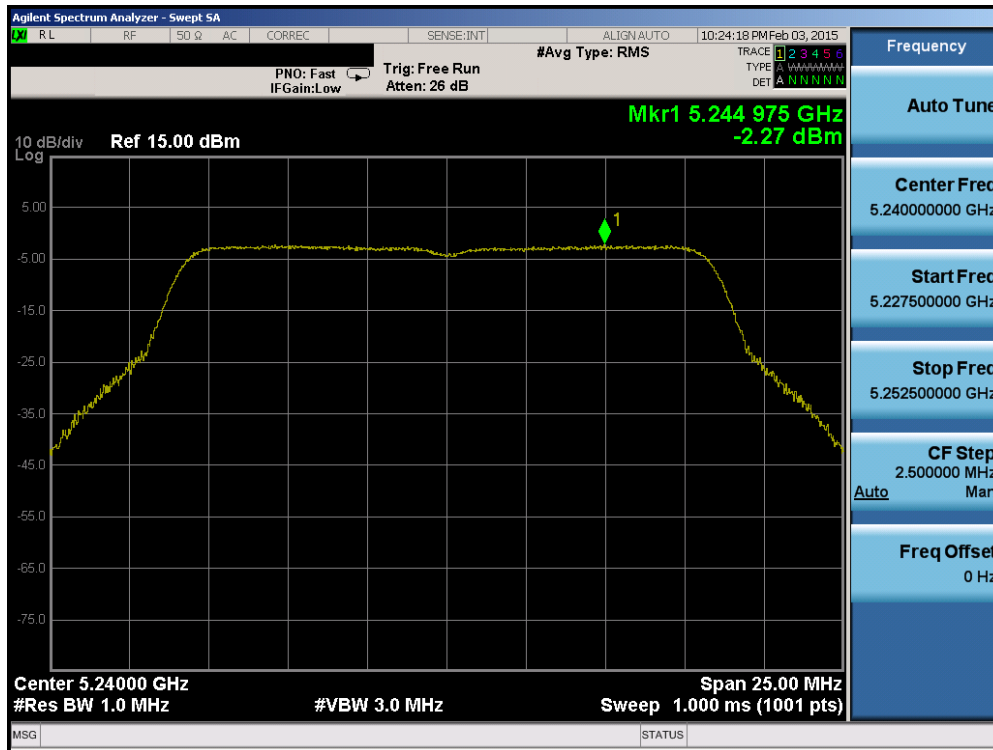
Plot 6-35. Power Spectral Density Plot (802.11a (UNII Band 1) – Ch. 48)
