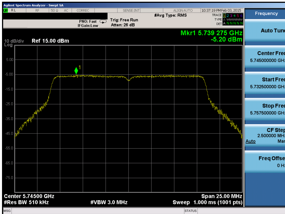
Plot 6-57. Power Spectral Density Plot (802.11a (UNII Band 3) – Ch. 149)
