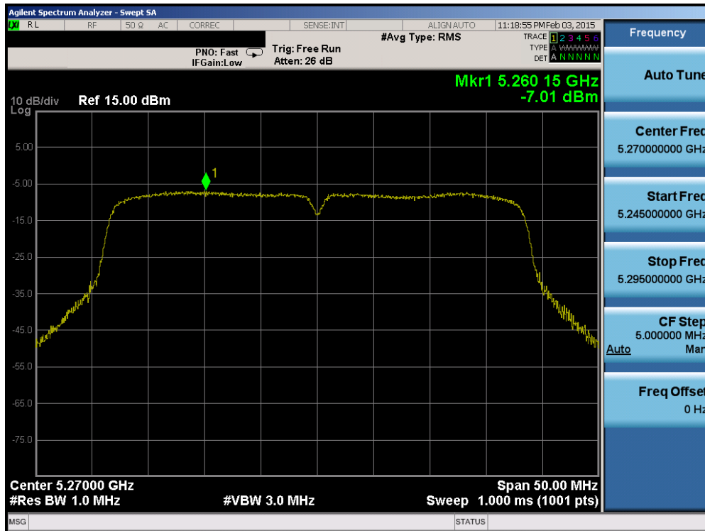
Plot 6-47. Power Spectral Density Plot (40MHz BW 802.11n (UNII Band 2A) – Ch. 54)
