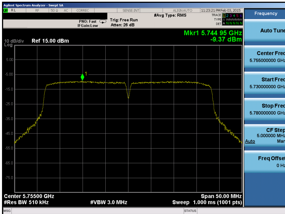
Plot 6-63. Power Spectral Density Plot (40MHz BW 802.11n (UNII Band 3) – Ch. 151)
