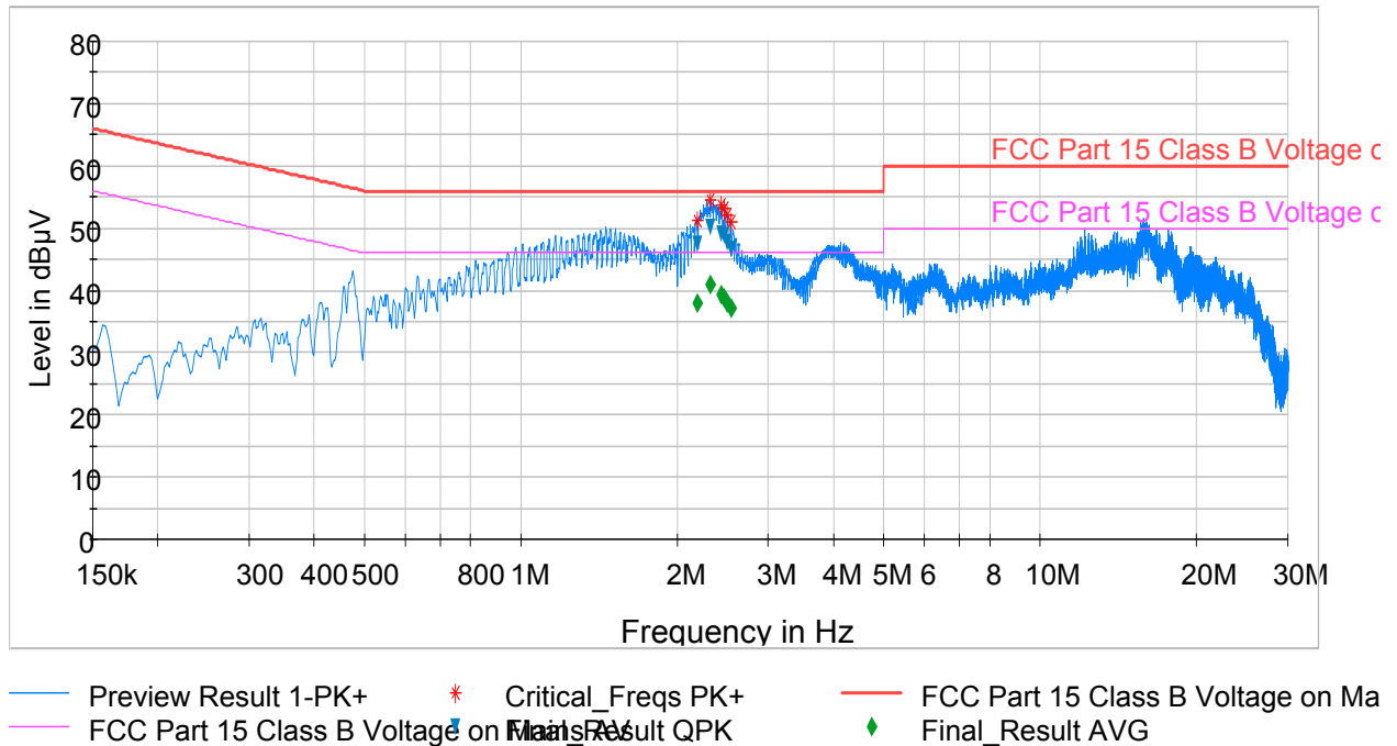
Plot 6-102. Line Conducted Plot with 802.11a UNII Band 3 (N)
