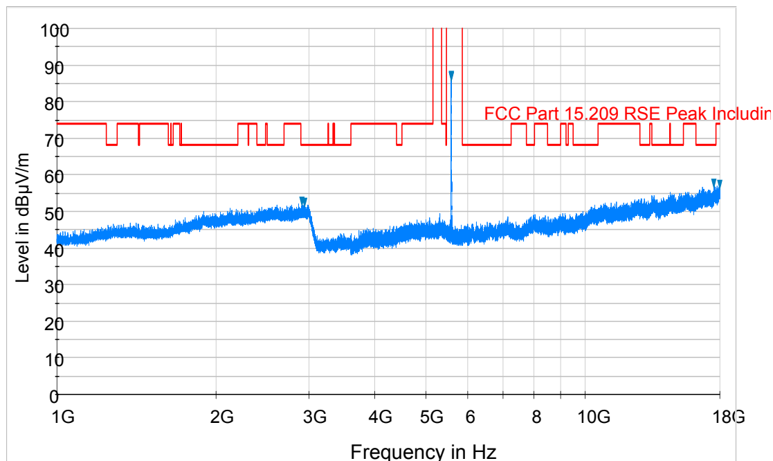
Plot 6-69. Radiated Spurious Plot above 1GHz (802.11a – U2C Ch. 116, Ant. Pol. H)
