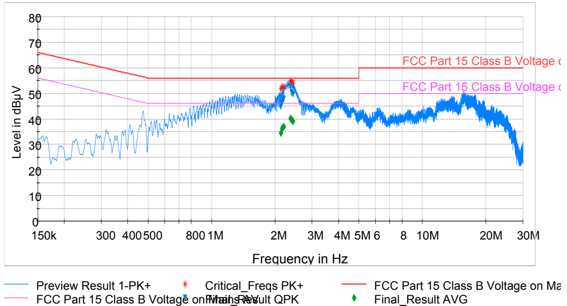
Plot 6-100. Line Conducted Plot with 802.11a UNII Band 2C (N)
