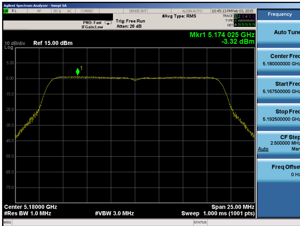
Plot 6-36. Power Spectral Density Plot (20MHz BW 802.11n (UNII Band 1) – Ch. 36)
