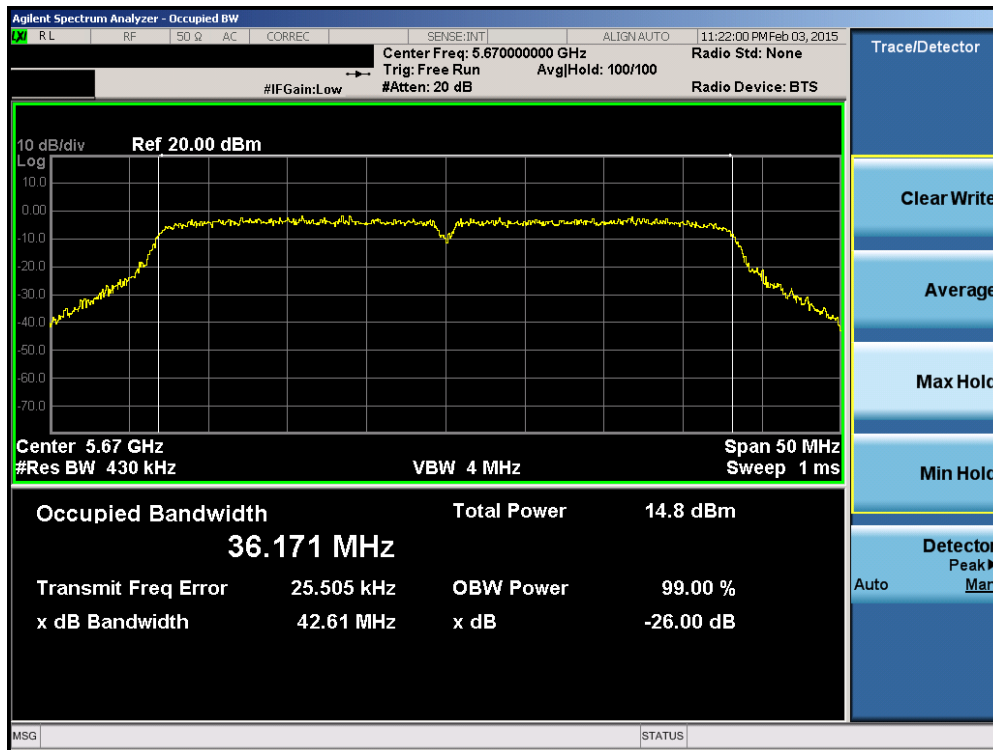
Plot 6-24. 26dB Bandwidth Plot (40MHz BW 802.11n (UNII Band 2C) – Ch. 134)
