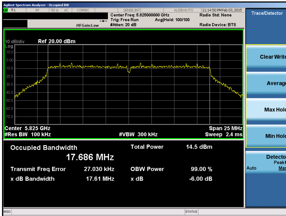
Plot 6-30. 6dB Bandwidth Plot (20MHz BW 802.11n (UNII Band 3) – Ch. 165)
