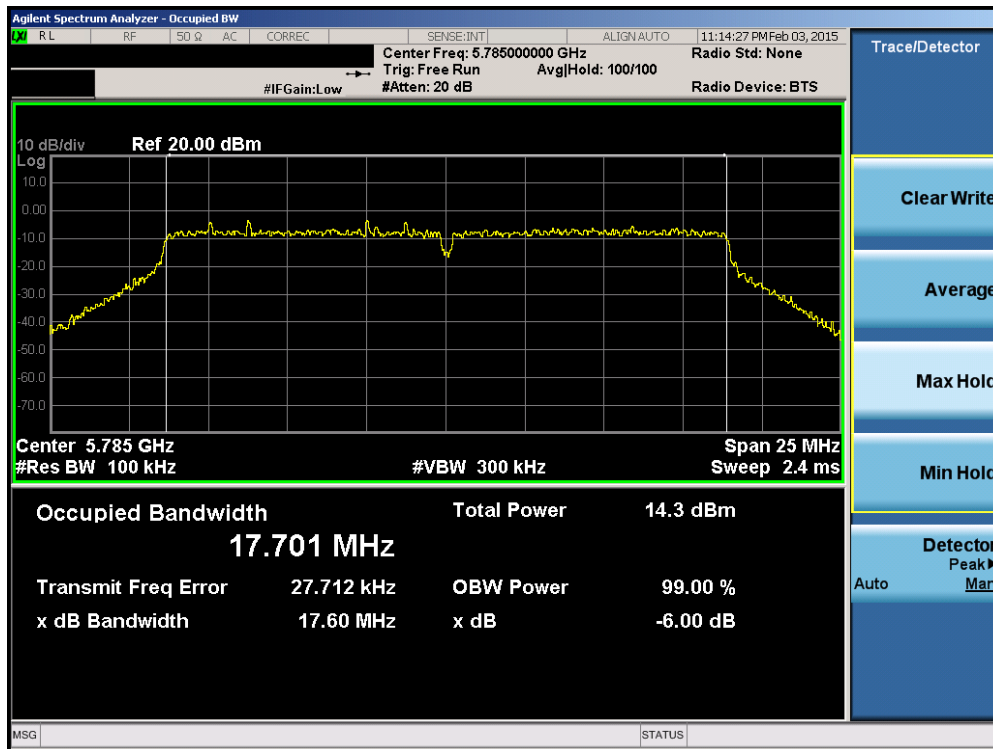
Plot 6-29. 6dB Bandwidth Plot (20MHz BW 802.11n (UNII Band 3) – Ch. 157)
