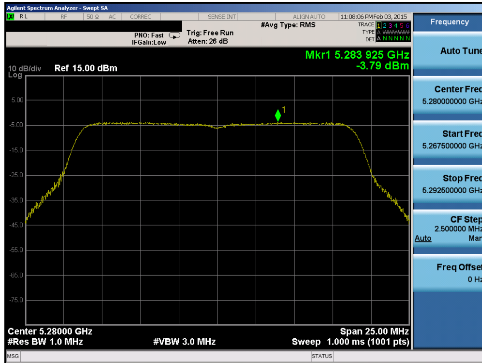
Plot 6-45. Power Spectral Density Plot (20MHz BW 802.11n (UNII Band 2A) – Ch. 56)
