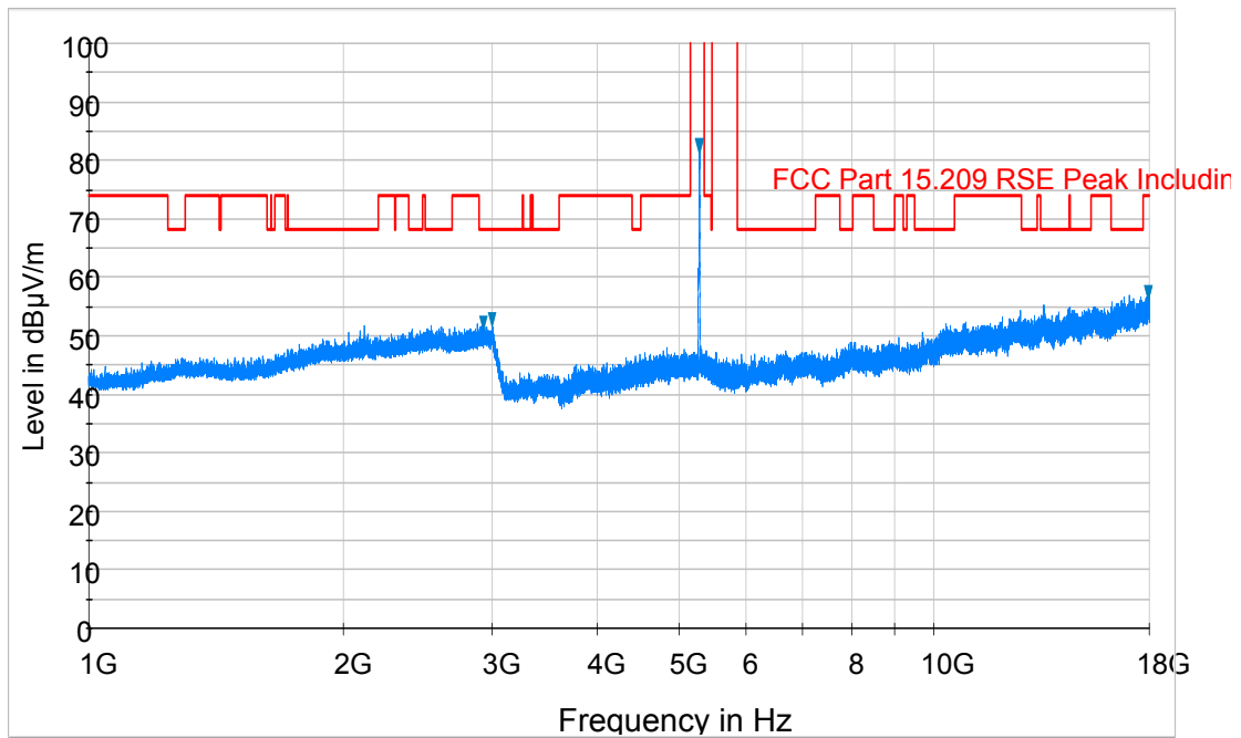
Plot 6-68. Radiated Spurious Plot above 1GHz (802.11a – U2A Ch. 56, Ant. Pol. V)
