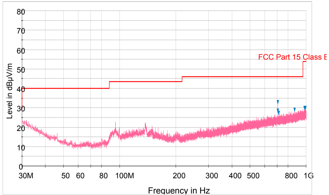
Plot 6-93. Radiated Spurious Plot below 1GHz (802.11a – U3 Ch. 157, Ant. Pol. H)
