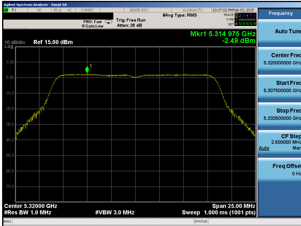
Plot 6-43. Power Spectral Density Plot (802.11a (UNII Band 2A) – Ch. 64)
