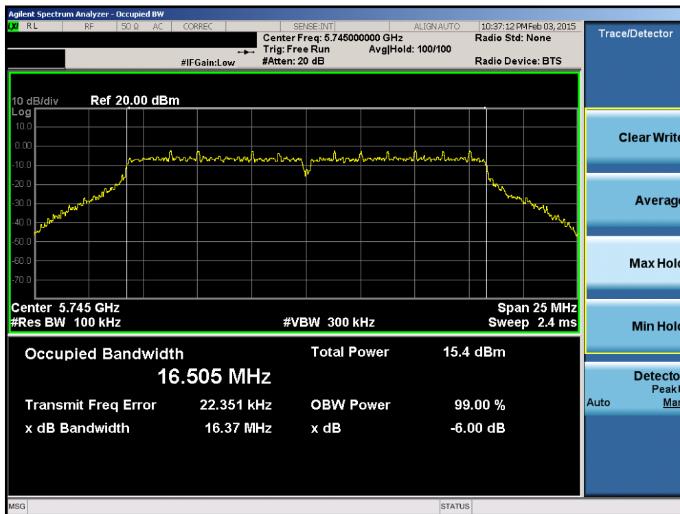
Plot 6-25. 6dB Bandwidth Plot (802.11a (UNII Band 3) – Ch. 149)
