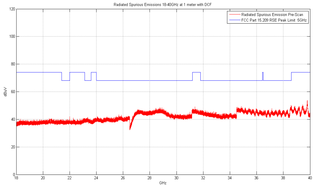
Plot 6-74. Radiated Spurious Plot above 18GHz (802.11a – Ant. Pol. V)
