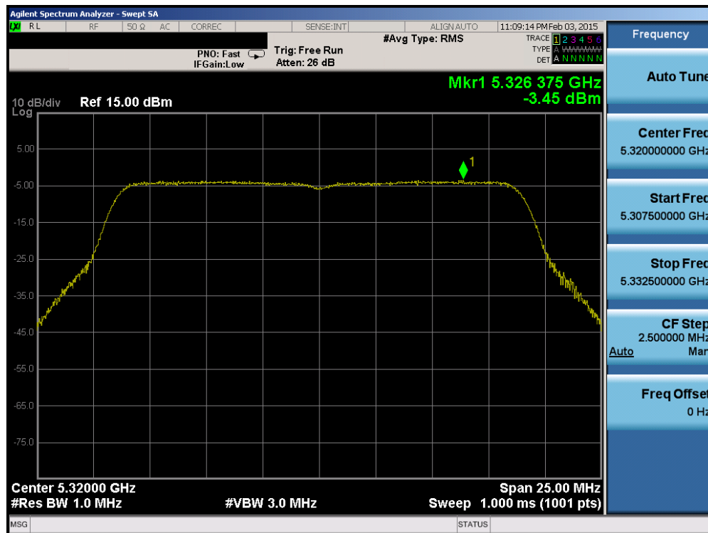
Plot 6-46. Power Spectral Density Plot (20MHz BW 802.11n (UNII Band 2A) – Ch. 64)
