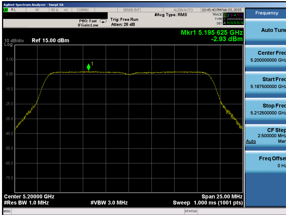
Plot 6-37. Power Spectral Density Plot (20MHz BW 802.11n (UNII Band 1) – Ch. 40)
