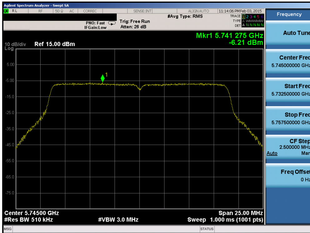
Plot 6-60. Power Spectral Density Plot (20MHz BW 802.11n (UNII Band 3) – Ch. 149)
