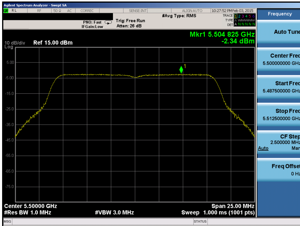
Plot 6-49. Power Spectral Density Plot (802.11a (UNII Band 2C) – Ch. 100)
