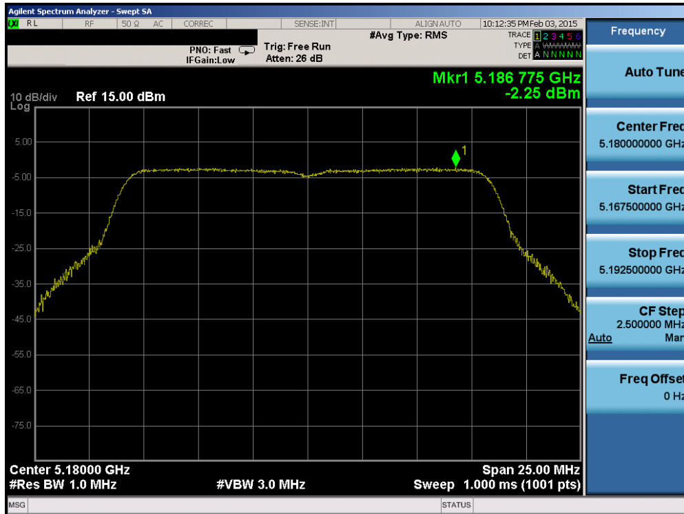
Plot 6-33. Power Spectral Density Plot (802.11a (UNII Band 1) – Ch. 36)
