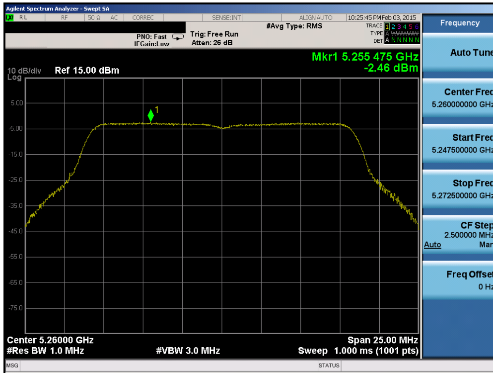
Plot 6-41. Power Spectral Density Plot (802.11a (UNII Band 2A) – Ch. 52)
