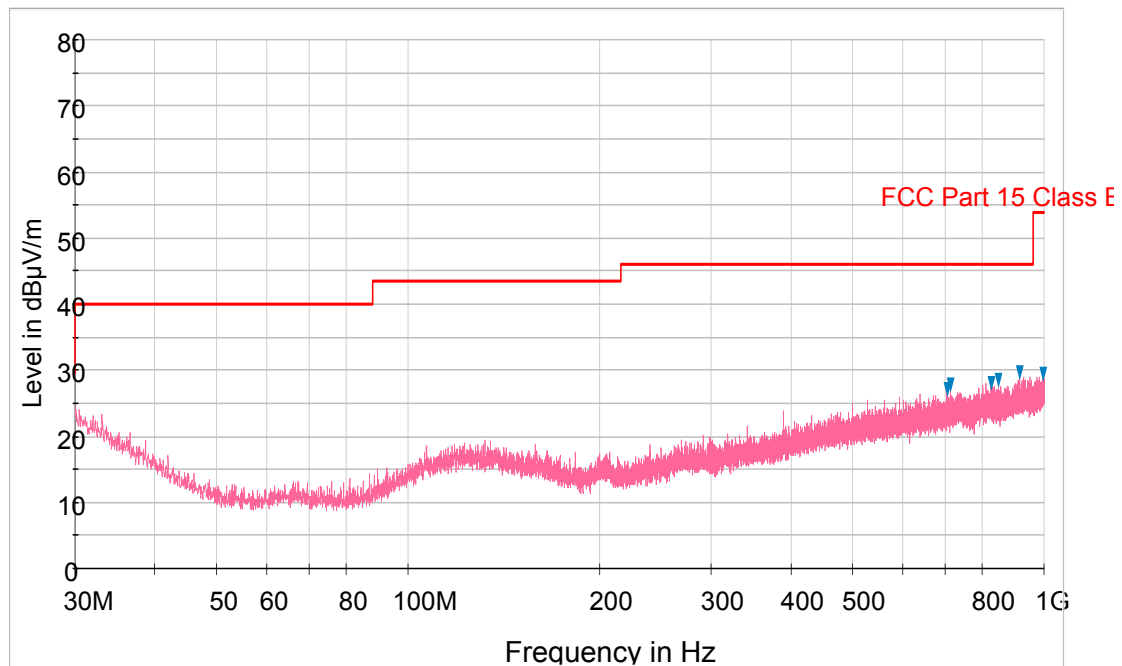
Plot 6-94. Radiated Spurious Plot below 1GHz (802.11a – U3 Ch. 157, Ant. Pol. V)
