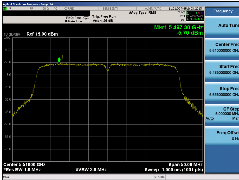
Plot 6-55. Power Spectral Density Plot (40MHz BW 802.11n (UNII Band 2C) – Ch. 102)
