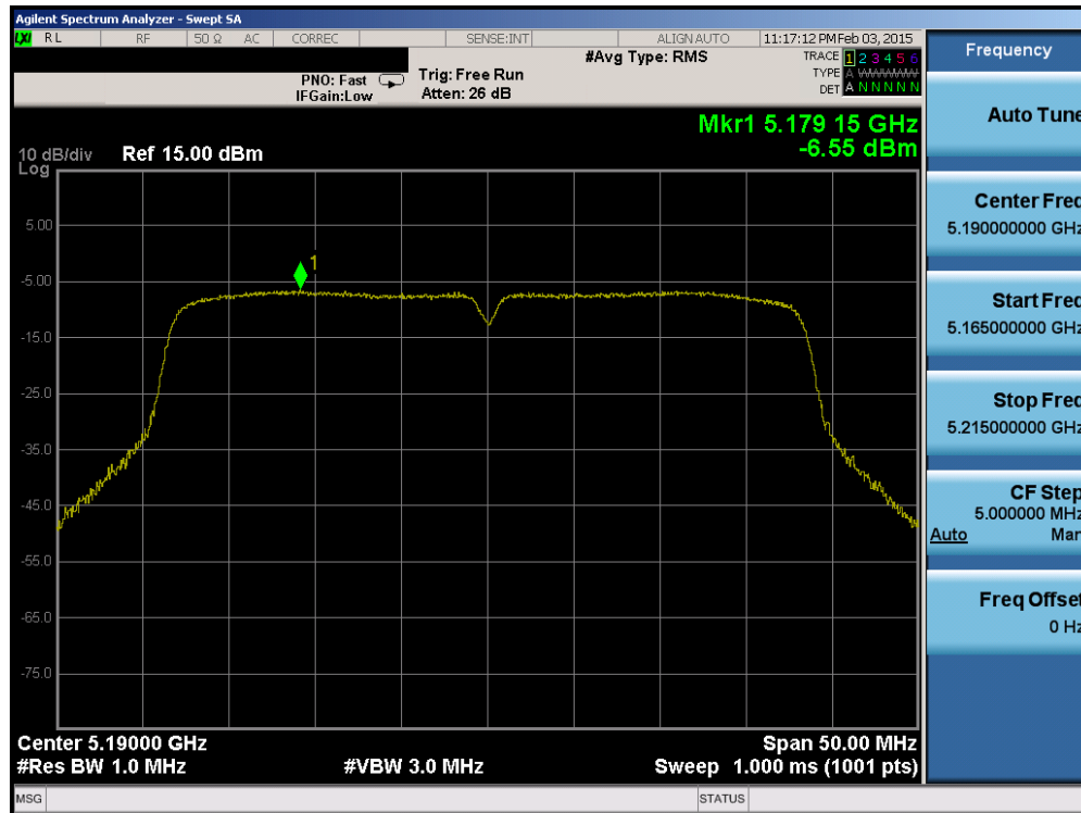
Plot 6-39. Power Spectral Density Plot (40MHz BW 802.11n (UNII Band 1) – Ch. 38)
