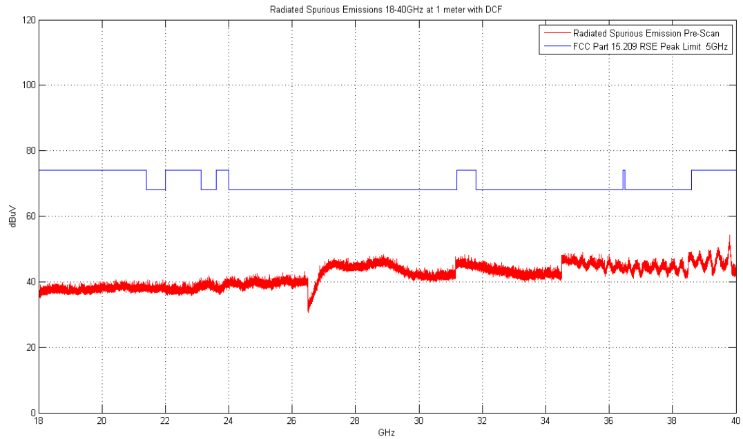
Plot 6-73. Radiated Spurious Plot above 18GHz (802.11a – Ant. Pol. H)
