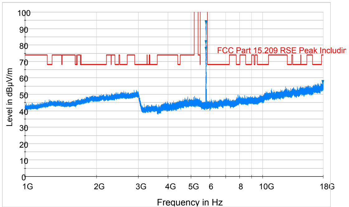
Plot 6-71. Radiated Spurious Plot above 1GHz (802.11a – U3 Ch. 157, Ant. Pol. H)
