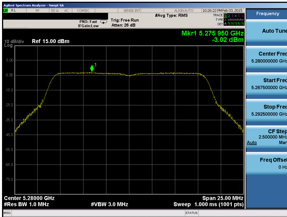
Plot 6-42. Power Spectral Density Plot (802.11a (UNII Band 2A) – Ch. 56)
