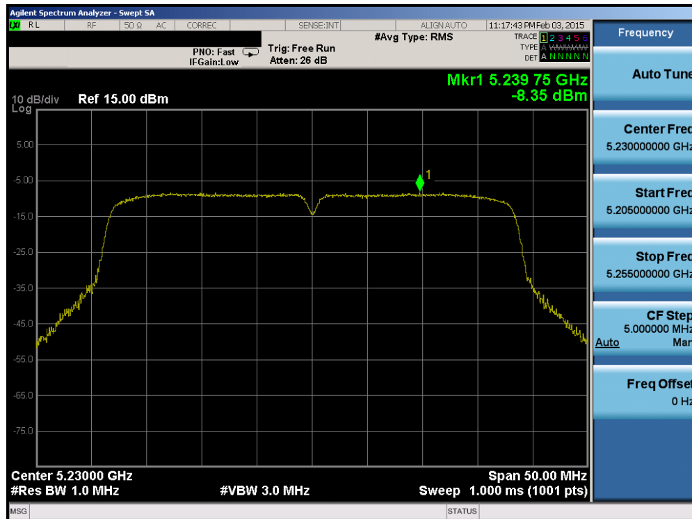
Plot 6-40. Power Spectral Density Plot (40MHz BW 802.11n (UNII Band 1) – Ch. 46)
