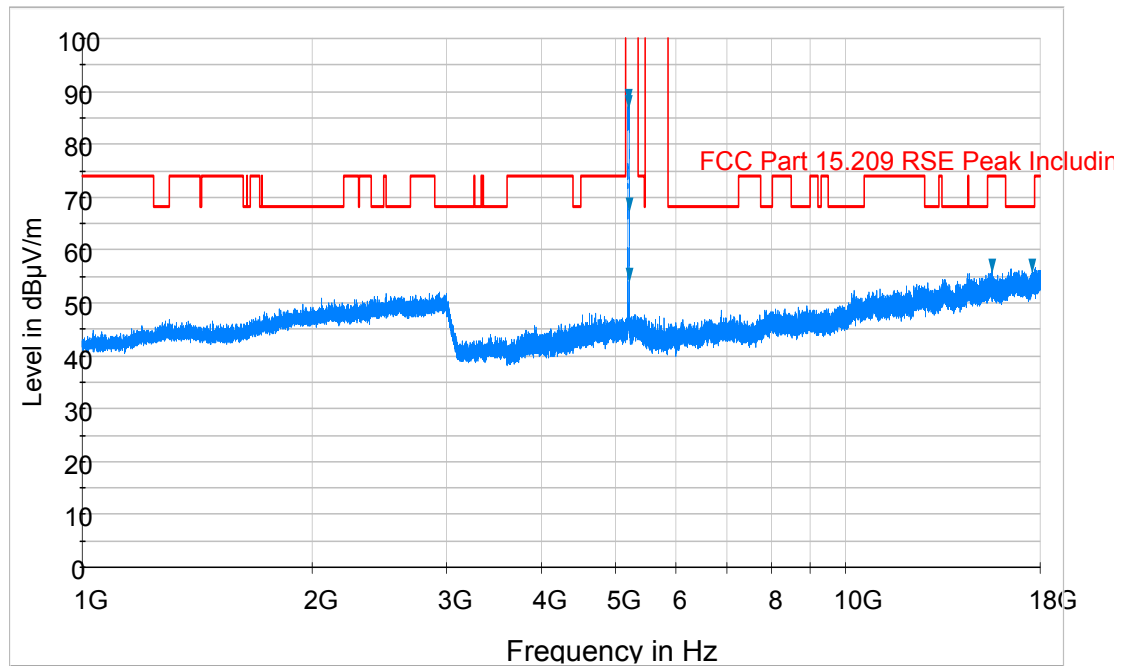
Plot 6-65. Radiated Spurious Plot above 1GHz (802.11a – U1 Ch. 40, Ant. Pol. H)
