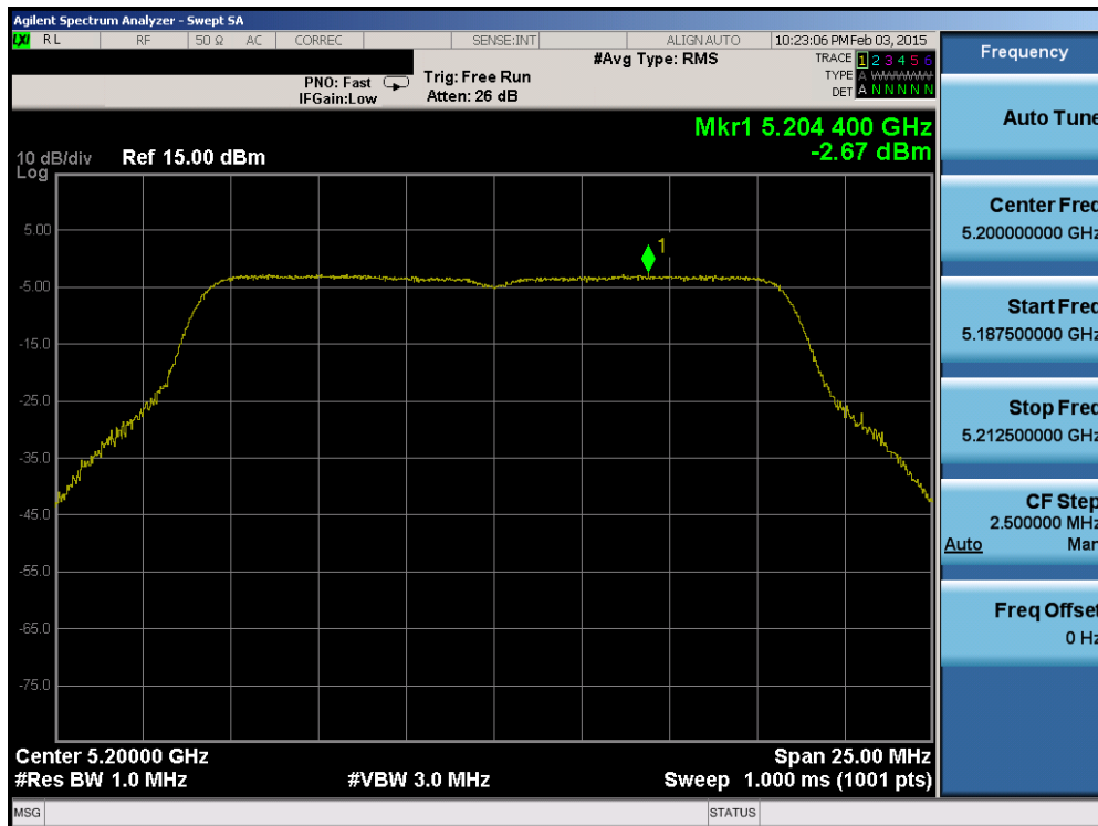
Plot 6-34. Power Spectral Density Plot (802.11a (UNII Band 1) – Ch. 40)
