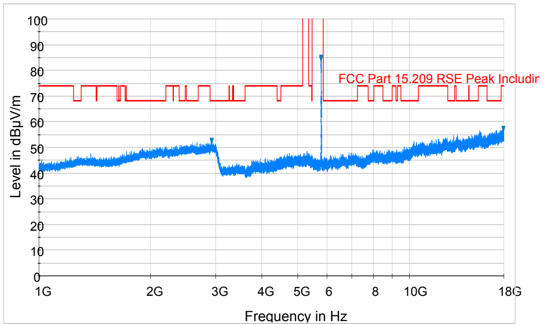
Plot 6-72. Radiated Spurious Plot above 1GHz (802.11a – U3 Ch. 157, Ant. Pol. V)
