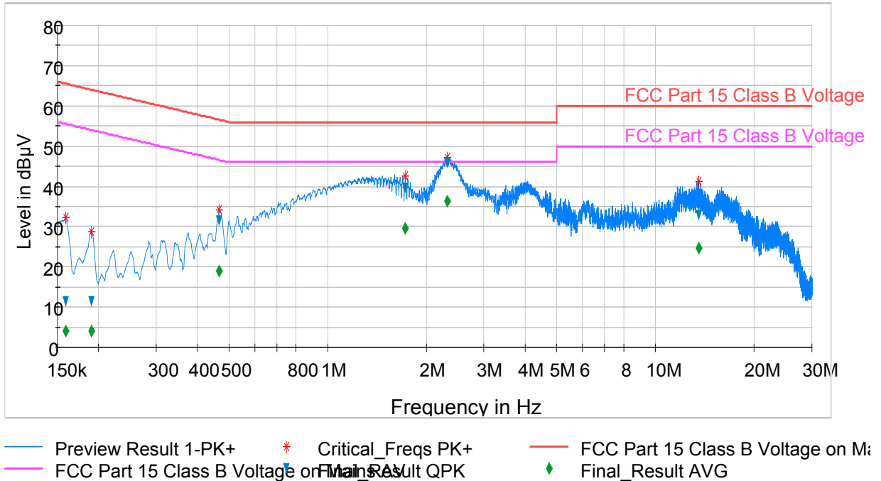
Plot 6-97. Line Conducted Plot with 802.11a UNII Band 2A (L1)
