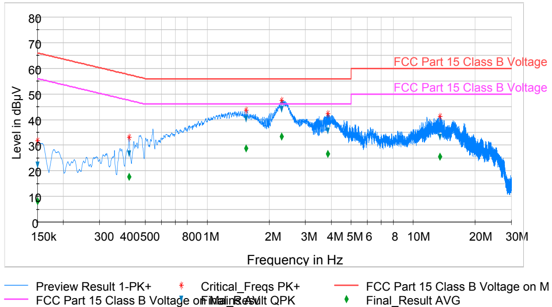
Plot 6-101. Line Conducted Plot with 802.11a UNII Band 3 (L1)
