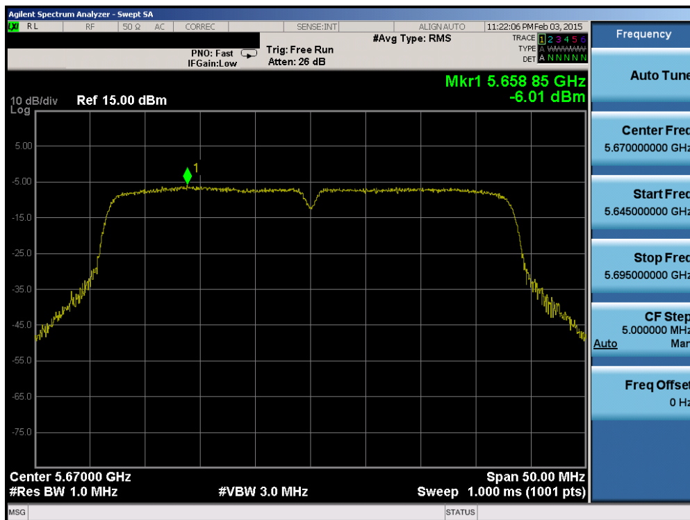
Plot 6-56. Power Spectral Density Plot (40MHz BW 802.11n (UNII Band 2C) – Ch. 134)
