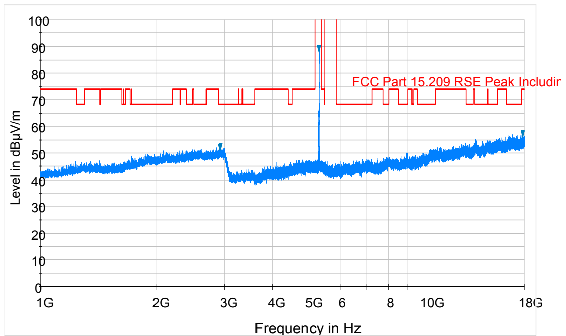
Plot 6-67. Radiated Spurious Plot above 1GHz (802.11a – U2A Ch. 56, Ant. Pol. H)
