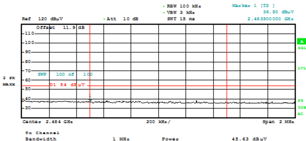
Plot 6-18. Radiated Restricted Upper Band Edge Measurement (Average)
